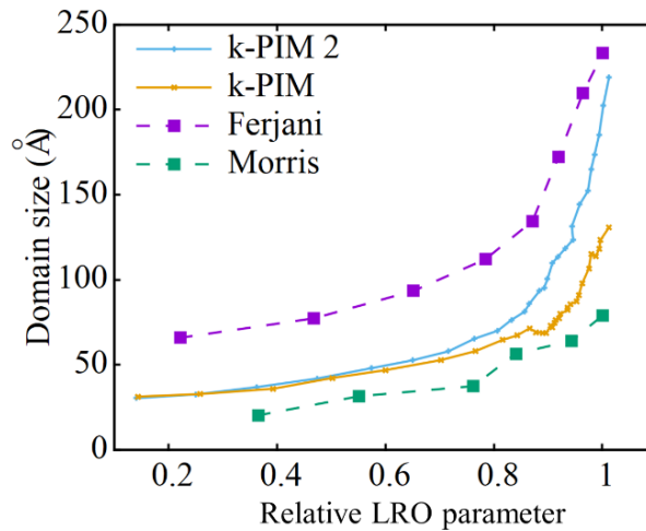
Figure III.21. Evolution of the ordered domain size as function of relative long-range order parameter in Fe-75%Ni at T=743 K (470 °C): comparison between the AKMC results and experiments of Ferjani et al. (Ferjani, Bley, and Calvayrac 1977) and Morris et al. (Morris et al. 1976).
