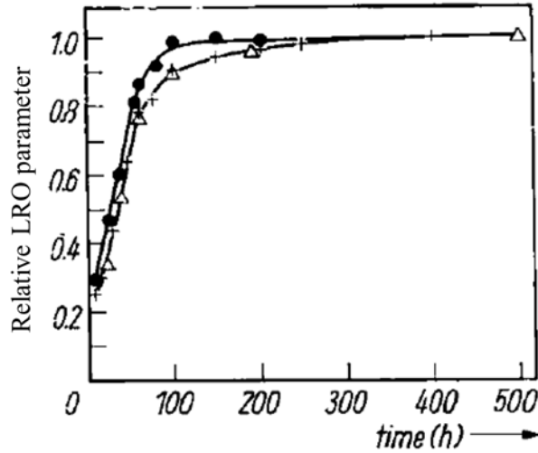
Figure III.1. Evolution of the relative long-range order parameter with time: ● Fe-73%Ni at T = 480^\circ\text{C} (753 K); \Delta Fe-75%Ni at T = 480^\circ\text{C} (753 K); + Fe-75%Ni at T = 497^\circ\text{C} (770 K) (Calvayrac and Fayard 1973)
