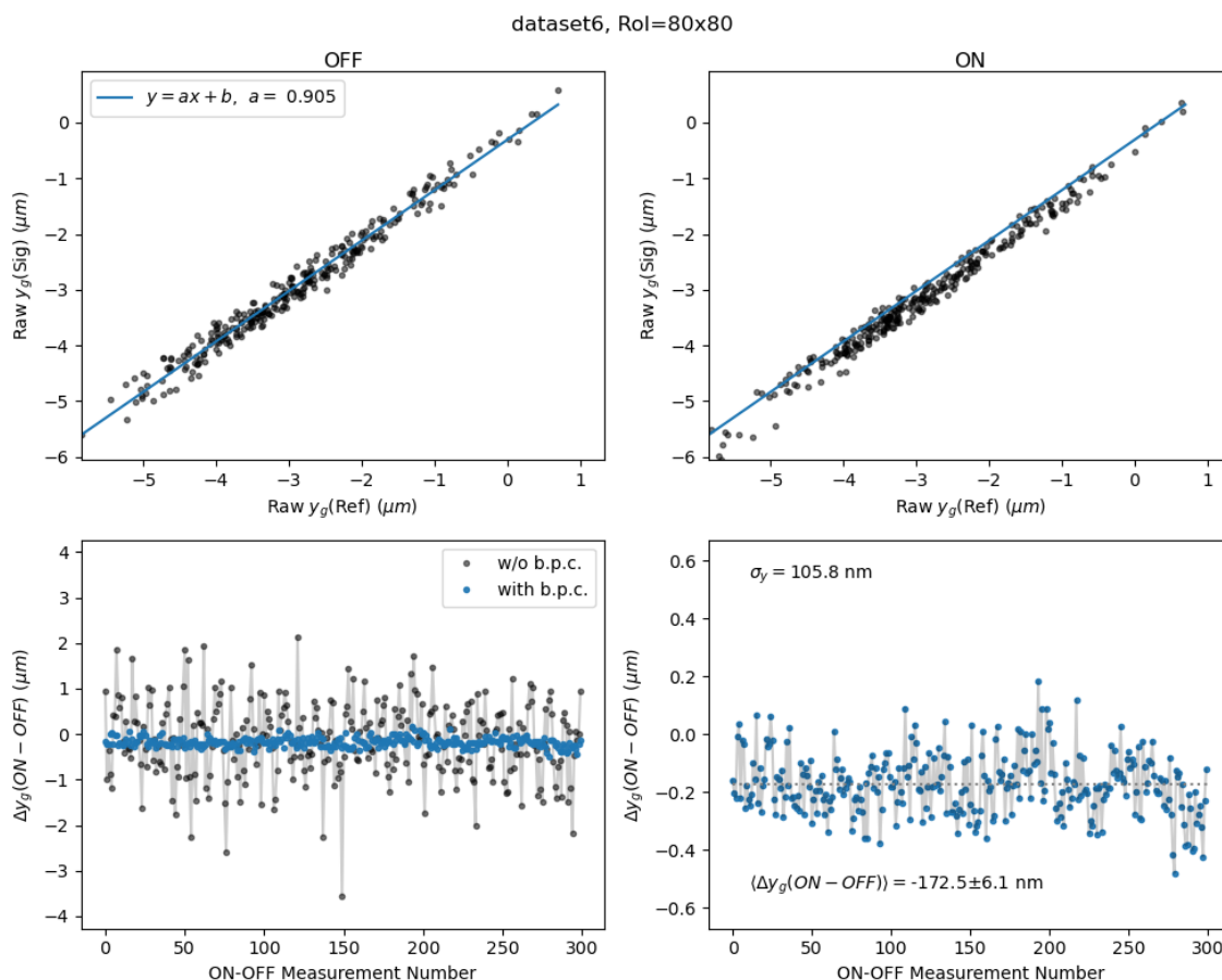
Figure 3.4: (Upper plots) Linear correlation of the barycenters in intensity of the interference signal \bar{y}_{sig}(i) and the back-reflection \bar{y}_{ref}(i) , calculated along the vertical axis y . The data are shown as black points, for both OFF (left panel) and ON (right panel) measurements, while the result of the linear fit obtained using the OFF data only is shown in both panels as a blue line. (Lower plots) black points: ON-OFF raw signal \bar{y}_{sig}^{ON}(i) - \bar{y}_{sig}^{OFF}(i) without beam pointing correction; blue points: ON-OFF reconstructed signal \Delta y(i) = \bar{y}_{corr}^{ON}(i) - \bar{y}_{corr}^{OFF}(i) after beam pointing correction. The signal \Delta y(i) is clearly identifiable in the lower right plot with an average value \Delta y = \langle \Delta y(i) \rangle = -172.5 \pm 6.1 nm. In this example, data have been collected on December, the 22th, 2022, dataset6.
