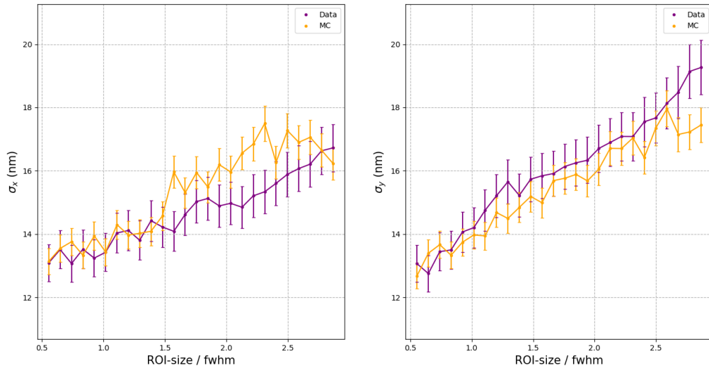
Figure 6.8: Evolution the spatial resolution in both direction \sigma_x (left panels) and \sigma_y (right panels), as a function of the RoI size over the spot size (FWHM) for both CCD cameras at the highest intensity I_{ref,max} (in ADU content) of the reference pulse. The results are given for the CCD camera 5.86 with I_{ref,max}^{5.86} \approx 2690 ADU (upper panels) and CCD 1.85 with I_{ref,max}^{1.85} \approx 3040 ADU (lower panels).
