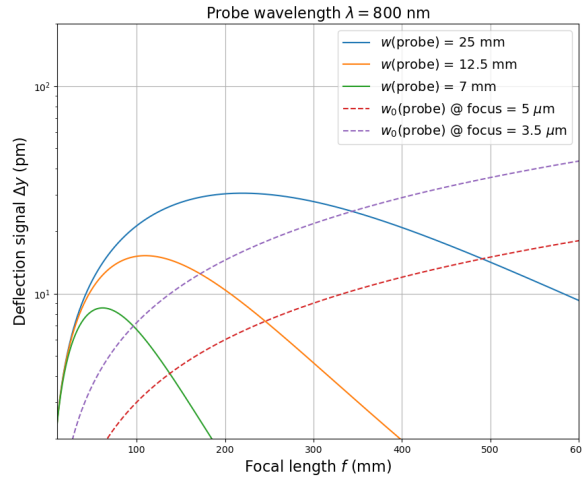
Figure 2.6: Plot of the DeLLight signal \Delta y (in pm) in the dark output of the interferometer as a function of the focal length f for three different waists w (25 mm in blue, 12.5 mm in orange and 7 mm in green) of the collimated probe beam in the interferometer, and for a pump waist at focus W_0 = 5\mu\text{m} . In dashed lines is plotted the signal \Delta y depending on the focal length, with the minimum waist w_0 of the probe beam at focus fixed at 5\mu\text{m} (red) and 3.5\mu\text{m} (purple), while w is a free parameter. The wavelength of the probe beam is 800 nm. The DeLLight signal is \Delta y = 14 \pm 1 pm for either f \approx 500 mm, w_0 = 5\mu\text{m} , w = 25 mm or f \approx 150 mm, w_0 = 3.5\mu\text{m} , w = 12.5 mm.
