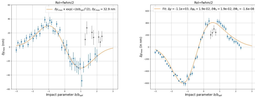
Figure 9.16: Measured deflection signal as a function of the impact parameter b of the pump pulse in the interaction area over its optimal value b_{opt} . (Left) Direct deflection signal \delta y_{mes} without amplification. We fit, in orange, that signal using the function: \delta y(b) = \delta y_{max} (b/b_{opt}) \exp((1 - (b/b_{opt})^2)/2) . (Right) Amplified deflection signal \Delta y_{mes} = \mathcal{A} \times \delta y_{mes} , where the amplification factor \mathcal{A} is negative as expected. In orange line is the result of the fit taking into account the phase signal \delta\psi(b) and the phase noise \delta\phi(y) = \delta\phi_0 + \delta\phi_1 y (see text for details).
