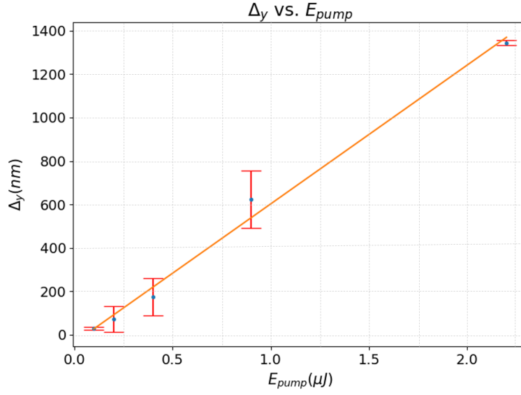
Figure 8.3: Evolution of the vertical displacement \Delta y (nm) of the intensity profile of the interference signal in the dark output of the Sagnac interferometer, for different pump energies \mathcal{E}_{pump} ( \mu J ). Data are in red and the linear fit is in orange.
