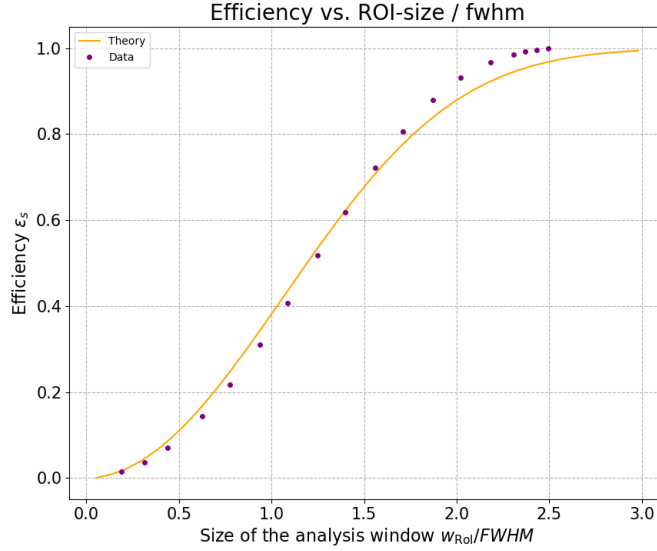
Figure 3.3: Evolution of the theoretical efficiency \epsilon_s (orange) as a function of the ROI-size w_{RoI} , normalised to the FWHM of the Gaussian beam profile. The measured efficiency is plotted in purple.
