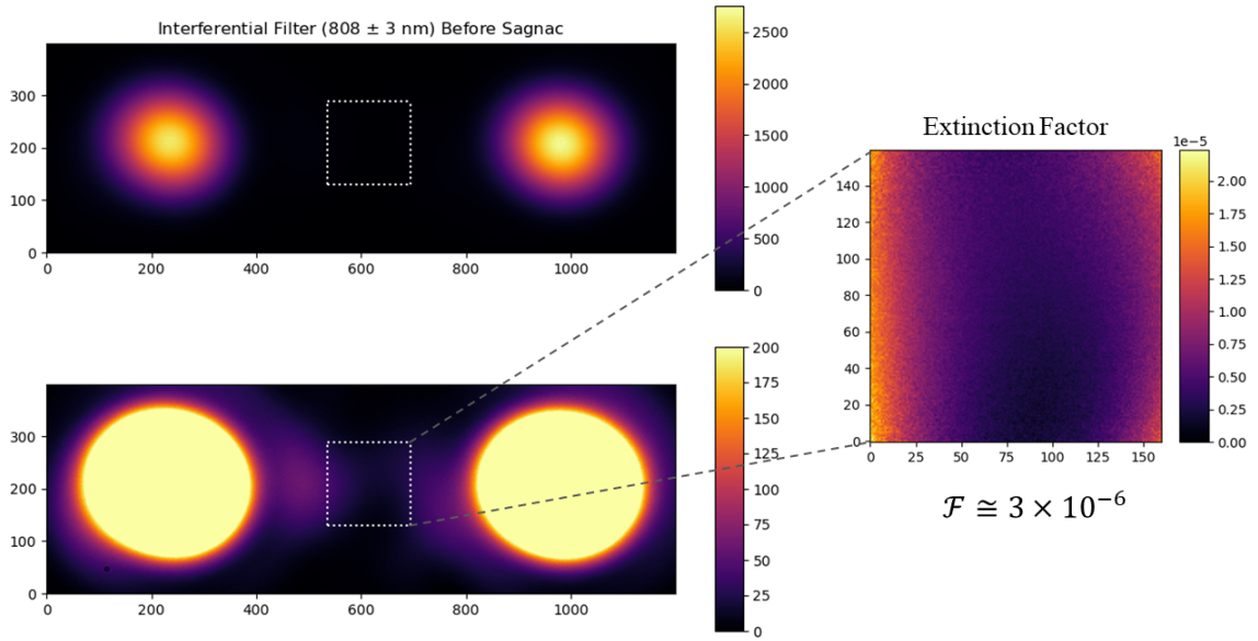
Figure 5.4: Same as figure 5.3, but with the spectral filter placed before the triangular Sagnac interferometer. The maximal extinction factor achieved is \mathcal{F} \approx 3 \times 10^{-6} in the centre.
