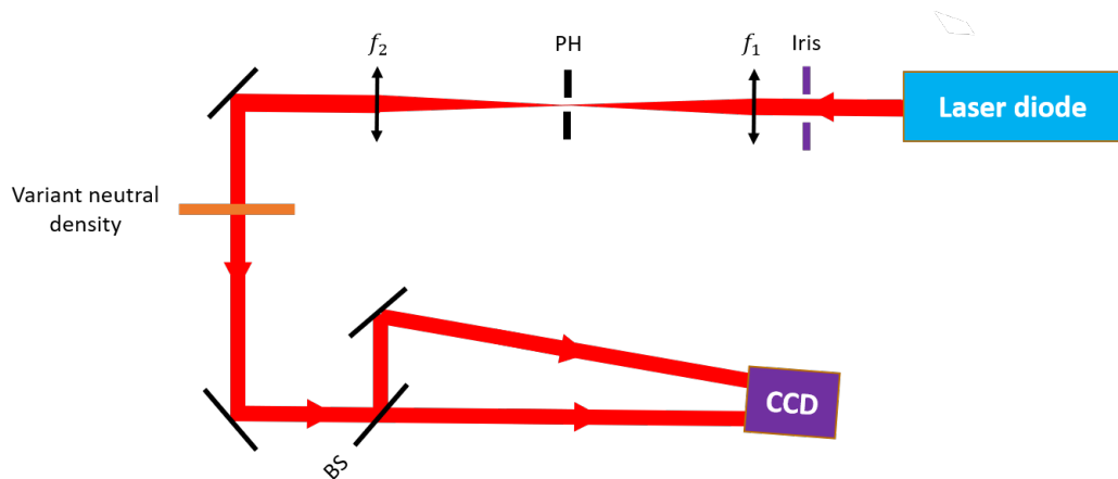
Figure 6.1: Schematic of the experimental setup to measure the spatial resolution. A telescope composed of two lenses (focal length f_1 = 150 \text{ mm} and f_2 = 100 \text{ mm} ) and a pinhole (PH) of diameter 75 \mu\text{m} shape the incident beam profile coming from the laser diode.
