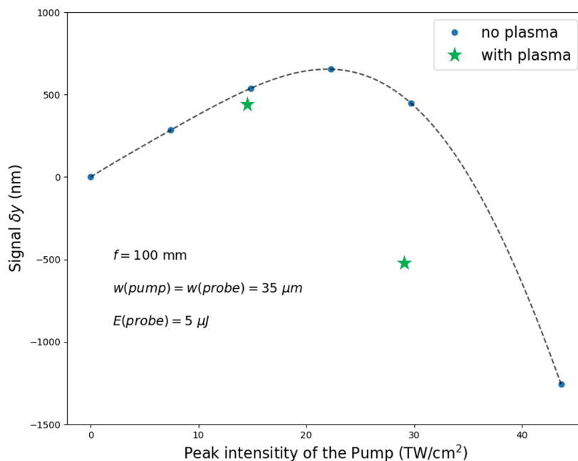
Figure 9.6: Expected un-amplified vertical shift \delta y = f \times \langle \delta \theta_y \rangle (in nm) of the barycenter of the probe intensity profile after deflection by the pump pulse in the interferometer, as a function of the pump peak intensity at focus (in \text{TW}/\text{cm}^2 ), for a focal length in the interferometer f = 100 mm and an efficiency \epsilon_s = 1 . The blue dots (with polynomial fit in dashed line) correspond to the expected values for the optical Kerr effect with higher order indexes (from equation 9.6). The green dots correspond to the expected values when the contribution of the plasma index is added. This simulation takes into account the contribution of the probe peak intensity at focus. The input parameters for Gaussian pulses are: minimum waists at focus w_0(\text{pump}) = 31.1 \mu\text{m} and w_0(\text{probe}) = 35.4 \mu\text{m} ; pulse duration 55 fs; probe energy 5 \mu\text{J} .
