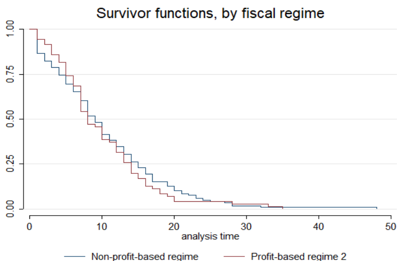
Figure 2: Kaplan-Meier estimates of time duration by Tax regime (Profit base fiscal regime 2)
