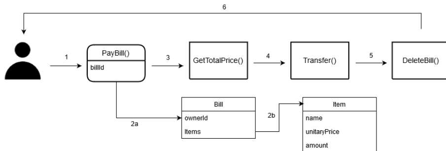
Figure 6.3: Chaincode steps for paying a bill. 1: user invokes the payBill function. 2: the function retrieves the associated bill and its owner, and the items linked to it. 3: The price is computed. 4: the chaincode tries to send the total price from the user to the bill owner. 5: if successful, the bill is deleted, and 6: the user receives a confirmation.
