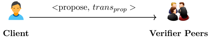
Figure 3.4: Transaction Proposal.
