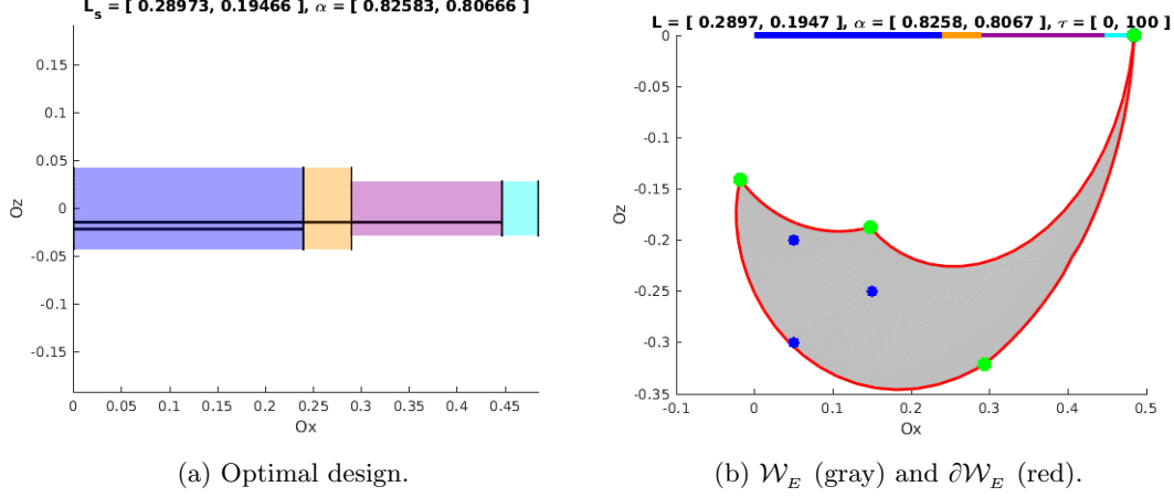
Figure 6.5: Soft robot's optimal design - achieving multiple points.
