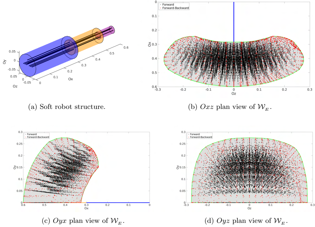
Figure 4.12: Scenario 5 - \mathcal{W}_E estimation via forward approach (black points) and forward-backward approach (gray area).
