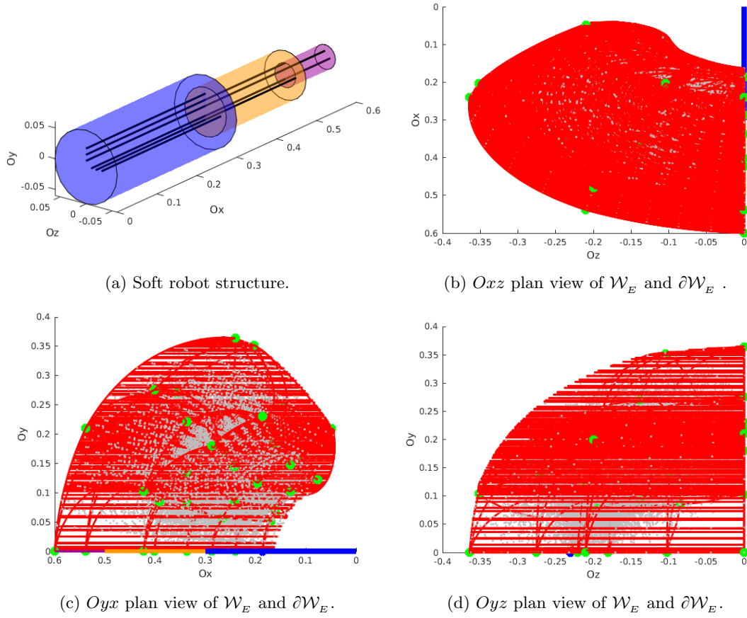
Figure 5.13: Scenario 7 - W_E estimation via forward approach (gray points) and workspace boundaries \partial W_E computed via the continuation approach (red curves and green bifurcation points).
