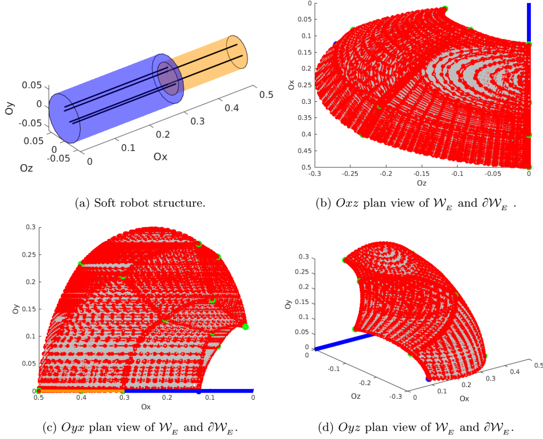
Figure 5.11: Scenario 5 - W_E estimation via forward approach (gray points) and workspace boundaries \partial W_E computed via the continuation approach (red curves and green bifurcation points).
