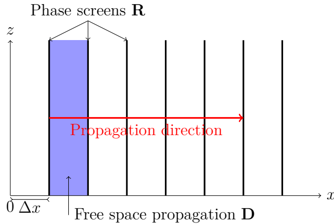
Figure 1.4: Split-step method.
