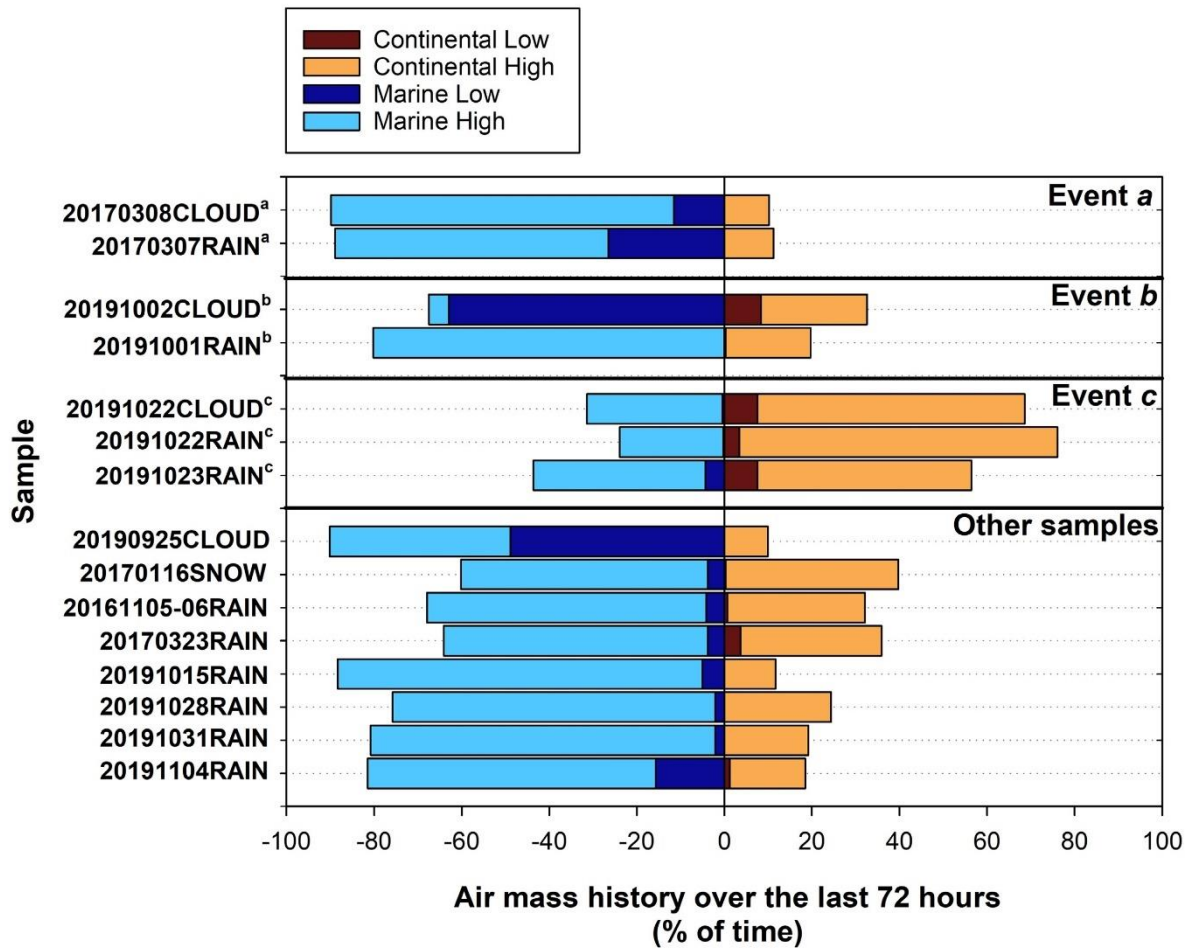
Figure 1. Air masses' history over the 72 h preceding sampling, expressed as % of the time spent over continental (right, brown) or marine (left, blue) surfaces, in the free troposphere (High) or in the planetary boundary layer (Low). Data were extracted from ERA5 backward trajectory plots at cloud altitude for rain samples or PUY altitude for clouds and snow. The % of time spent over marine surfaces is shown as negative values for graphical representation. *Superscripted letters indicate chronological associations between cloud and rain samples.
