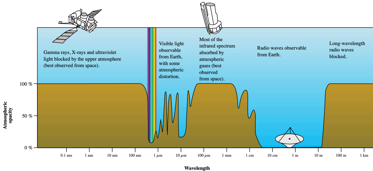
Figure 3.1: Schematic view of the atmosphere opacity of the electromagnetic radiation. Only a fraction, in the radio domain is is totally transparent. Credits: NASA.
