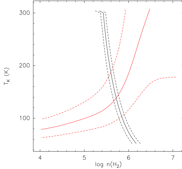
Figure 6.9: LVG grid performed to reproduce the physical conditions in N3 with SiO ratio 2-1/5-4 in black contours and H 2 CO line intensity ratio 3_{2,1} - 2_{2,0}/3_{0,3} - 2_{0,2} in red. The dashed lines correspond to a 10% uncertainty on line intensity ratios. We assumed the column density of both species to be 10^{14} \text{ cm}^{-2} .
