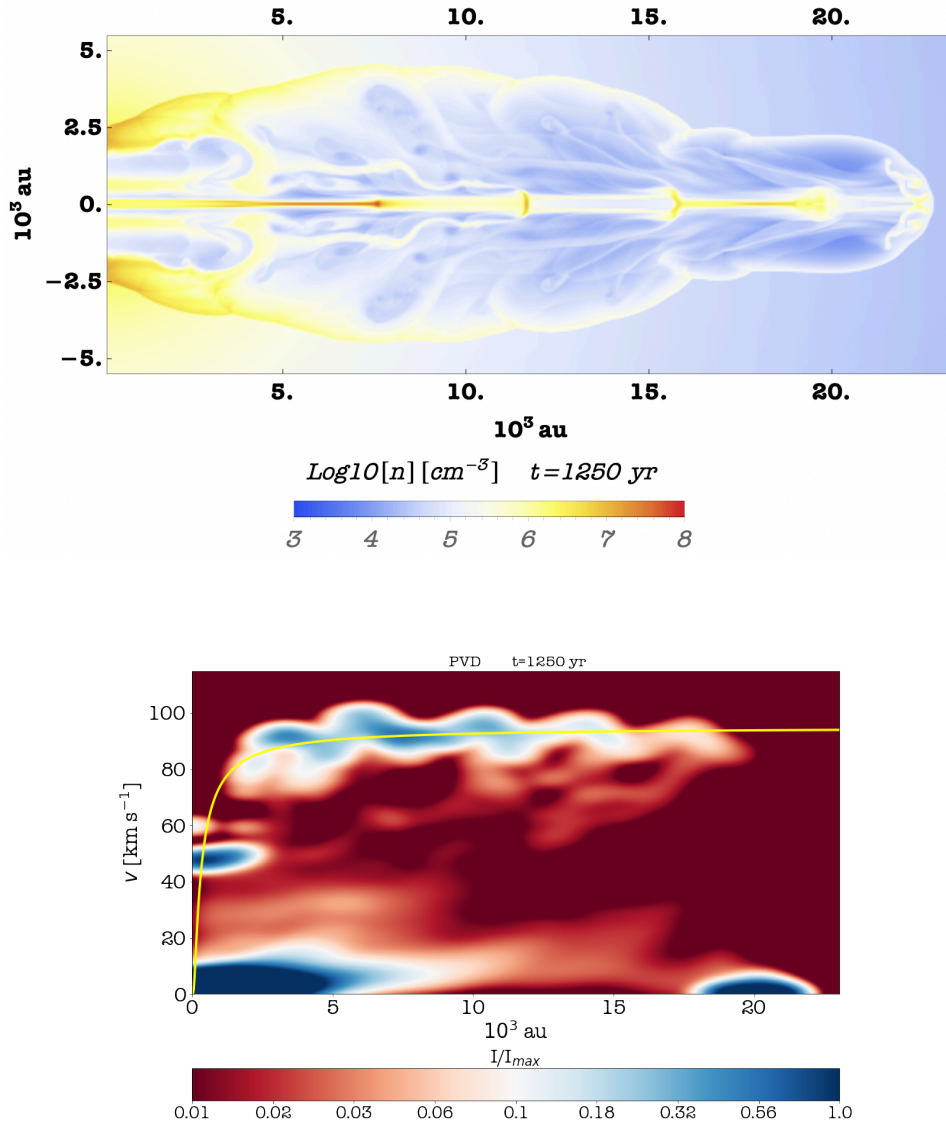
Figure 7.2: Best fitting model (M1) of the Cep E northern outflow at 1250 yr. (Top) Density distribution. The jet has propagated over a distance of 2.4 \times 10^4 au and formed a low-velocity cavity of 3000 au radius. Five knots and their associated wings are detected along the jet. (Bottom) Position-Velocity diagram of the CO emission along the jet main axis. The fit to the observational data (see Fig. 5.2) and corrected for the jet inclination with respect to the plane of the sky is superimposed in yellow.
