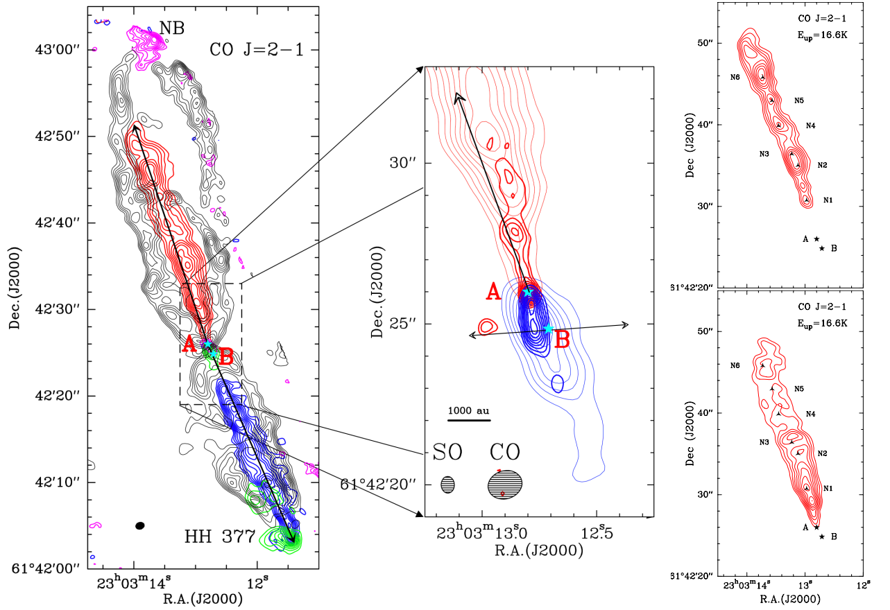
Figure 5.1: Molecular emission in the CepE outflow as observed: (left) in the CO 2–1 line with the PdBI at 1'' resolution by Lefloch et al. (2015): a) the outflow cavity walls (black) emitting at low velocities, in the range [-8; -3] km s ^{-1} and [-19; -14] km s ^{-1} in the northern and southern lobe, respectively; the jet, emitting at high velocities in the range [-135; -110] km s ^{-1} in the southern lobe (blue) and in the range [+40; +80] km s ^{-1} in the northern lobe (red); the southern terminal bow shock HH 377, integrated in the range [-77; -64] km s ^{-1} (green); the northern terminal bullet NB integrated in the velocity range [+84; +97] km s ^{-1} (magenta). (middle panel): SO N_J = 5_4-4_3 flux-integrated emission is displayed as thick contours superposed by the CO in thin. The arrows correspond to the CepE-B jet as determined by SiO J=5-4 transition. (right): emission integrated in the northern lobe in the range [55; 80] km s ^{-1} (upper) and [40; 55] km s ^{-1} (lower). First contour and contour interval are 20% and 10% of the peak intensity in each component, respectively. The synthesized beams are shown in the bottom left corner.
