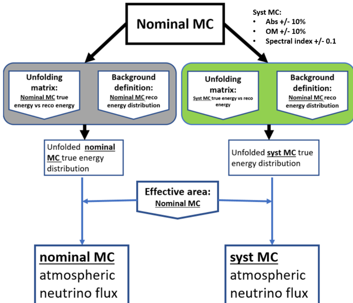
Figure 7.2: Schematic representation of the steps of the unfolding procedure to evaluate di effects of the systematics uncertainties on the atmospheric neutrino flux. The procedure starts with the nominal MC data as input for the unfolding, after which the procedure is divided in the nominal MC flux evaluation and the systematics fluxes evaluation. This procedure is used both for the muon neutrinos systematics evaluation and the electron neutrinos one.
