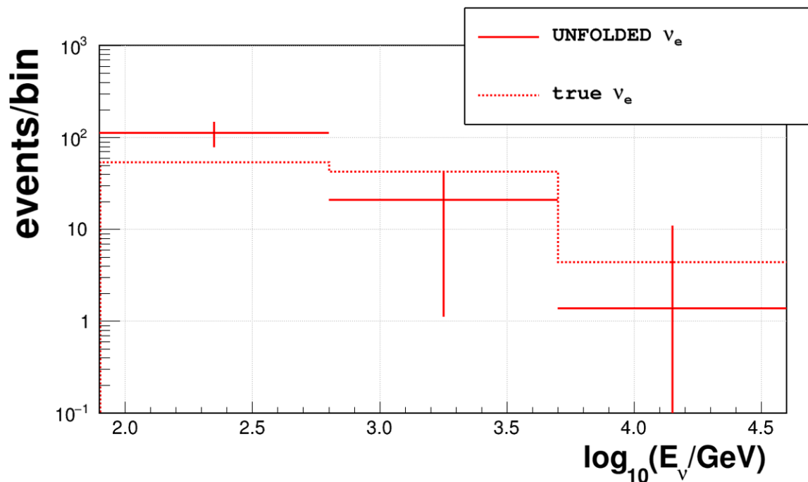
Figure 6.6: Electron neutrinos unfolded histogram compared with the true energy distributions generated in the Monte Carlo simulations. Crosses refer to unfolded distributions and dashed lines refer to simulated distributions.
