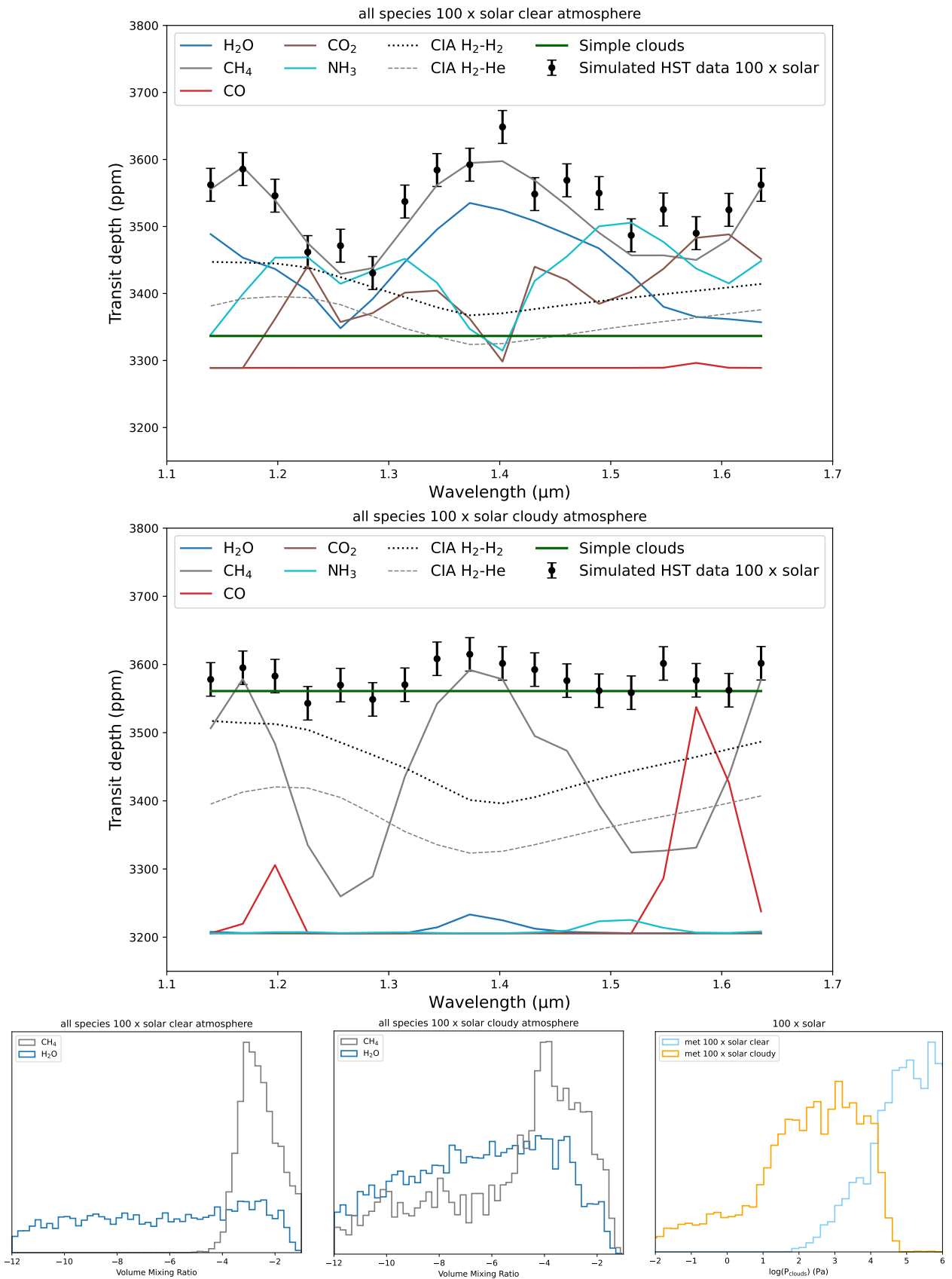
Figure 9.7: Results of the retrieval analysis on HST simulated data with CH 4 included as the main contributor and five transits observations.
