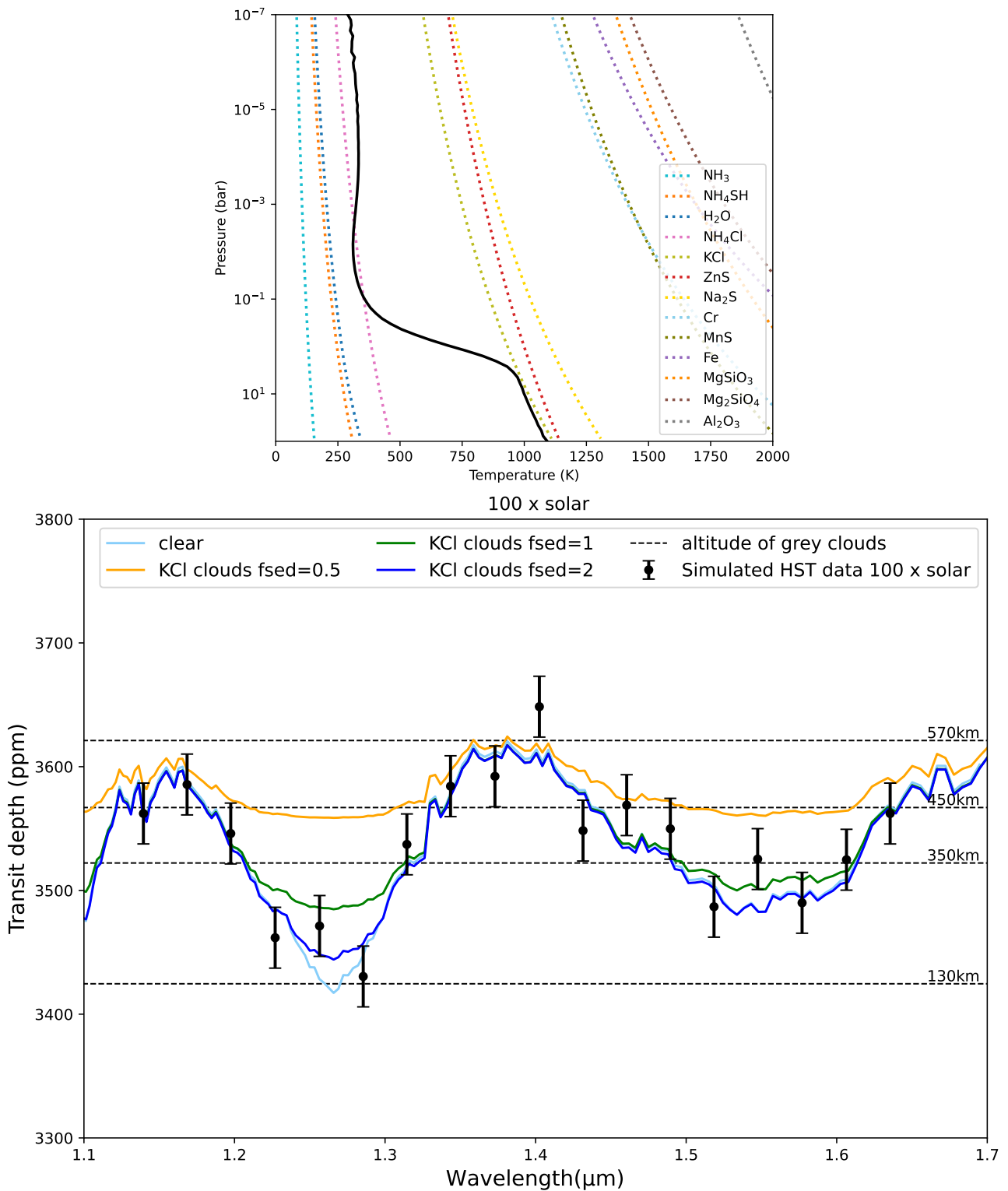
Figure 9.6: Simulated temperature–pressure profiles for LTT 3780 c (solid black lines) and condensation profiles (dotted lines) for a 100 \times solar metallicity atmosphere (top). Impact of radiative clouds in the transmission spectrum and altitudes of possible optically thick grey clouds (bottom).
