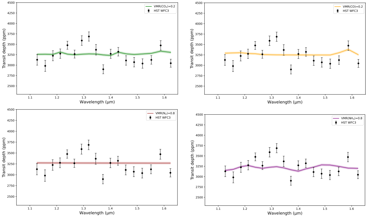
Figure 6.10: comparison of the best-fit atmospheric results for the TRAPPIST-1 h spectrum in the case of four forced secondary clear atmospheres with a volume mixing ratio of \text{CO}_2 fixed to 0.2 (upper left), \text{CO} to 0.2 (upper right), \text{N}_2 to 0.8 (bottom left), and ammonia to 0.8 (bottom right).
