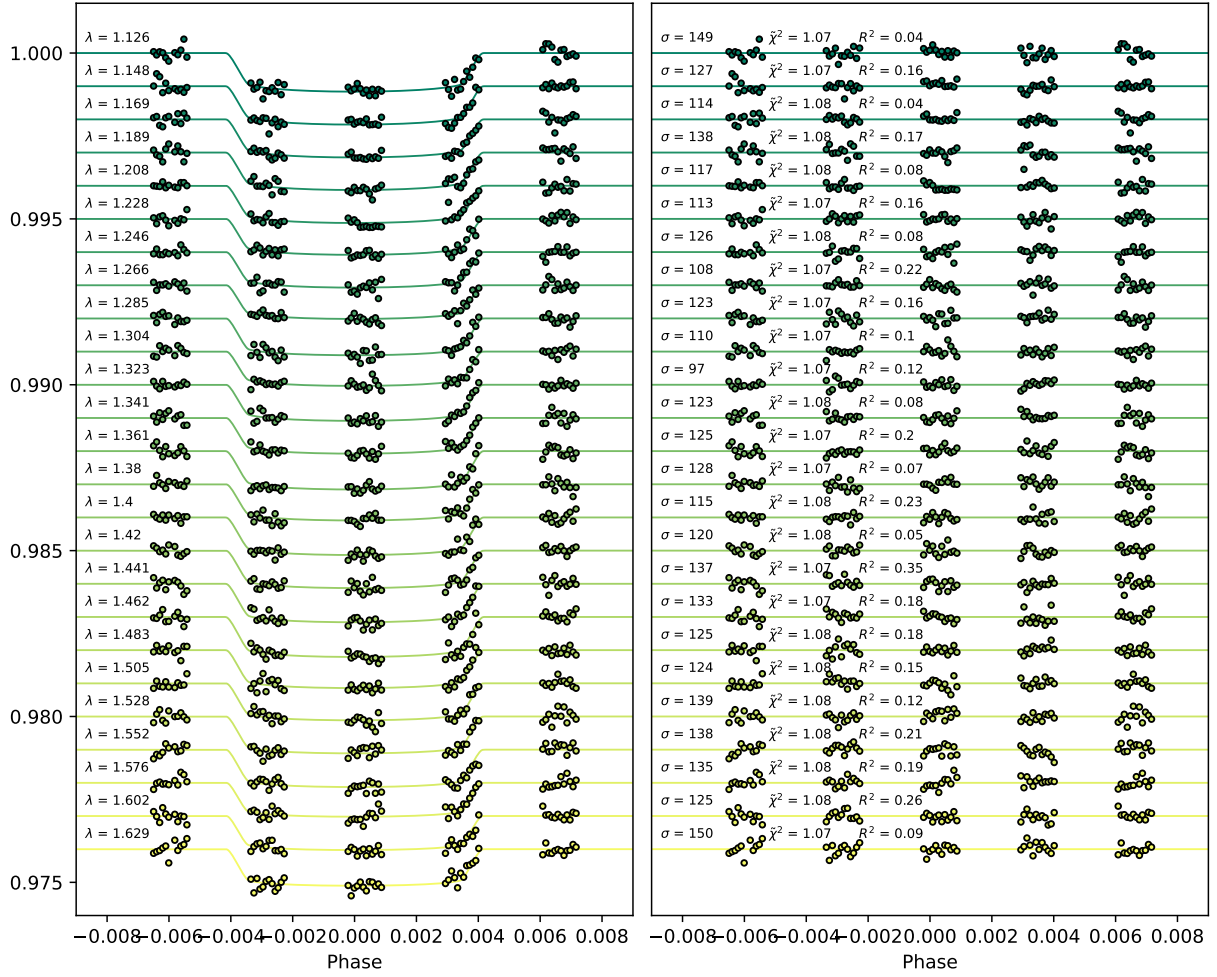
Figure 5.4: Spectral light curve fits for the first observation on HD 106315 c. An artificial offset in the y-axis was applied for clarity. For each light curve, the left panel shows the de-trended spectral light curves with the best-fit model in dotted lines, and the right panel shows the residuals and values for the standard deviation ( \sigma ) in ppm, the reduced Chi-squared ( \tilde{\chi}^2 ), and the auto-correlation ( R^2 ).
