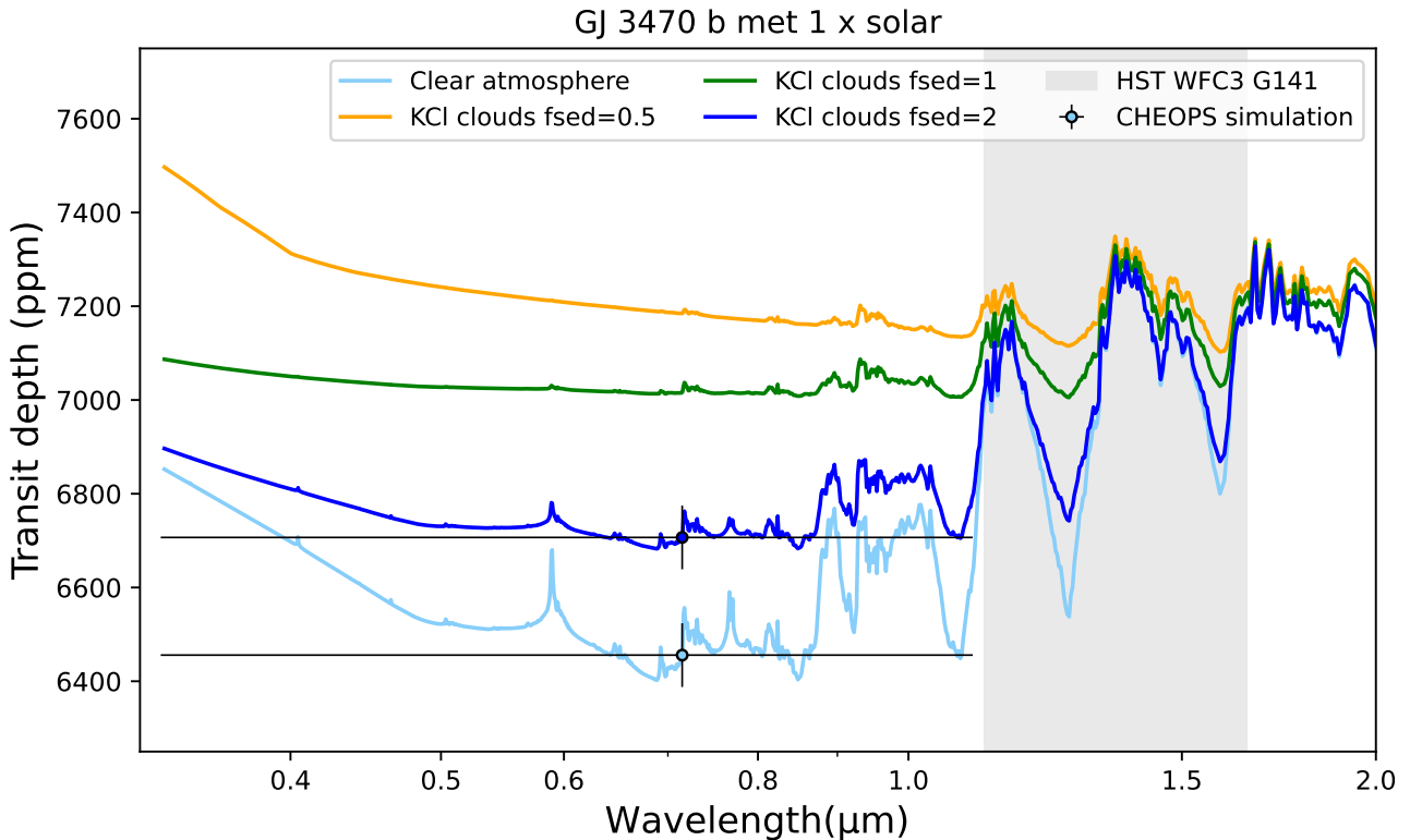
Figure 8.9: Impact of radiative clouds in the transmission spectrum of GJ3470 b for a 1 \times solar metallicity atmosphere. We include KCl clouds with three different sedimentation parameters and highlight the region probed by HST WFC3 G141 in grey. Simulations are from Exo-REM.
