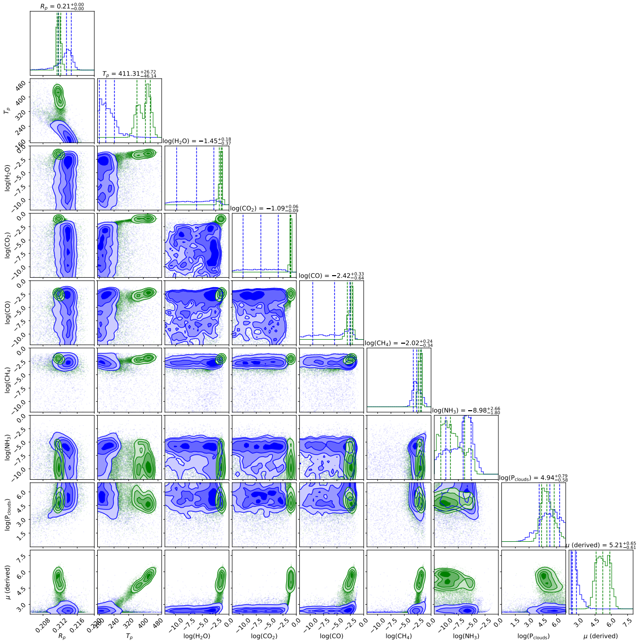
Figure 9.11: Posteriors distributions for the HST simulations with five transits of the WFC3 G141 (blue) and the JWST simulation with one transit of NIRISS and one transit of NIRSpec (green). The spectra are created based on the Exo-REM simulation of LTT 3780 c for 100 \times solar clear atmosphere.
