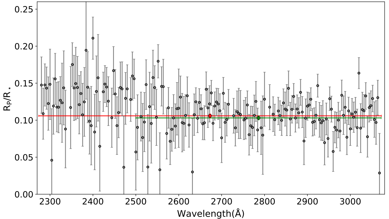
Figure 3.10: WASP-79b NUV transmission spectra in 4\text{\AA} bins for Observations 2. We indicate the overall NUV transmission spectrum (white light curve) R_P/R_\star(\text{NUV}) = 0.1059 in red, along with the planet-to-star radius ratio after 2500(\text{\AA}) in green R_P/R_\star(>2500\text{\AA}) = 0.1031 .
