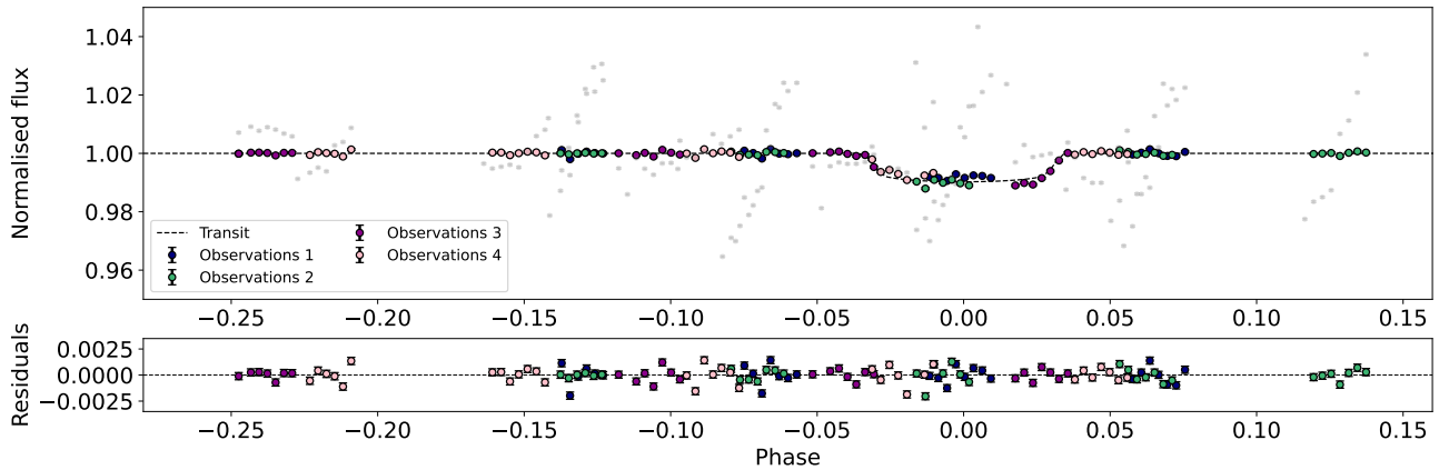
Figure 4.3: Normalised raw (grey) and corrected (colours) flux of 55-Cnc e four transit observations. The transit model is in a dotted line, computed for a planet-to-star radius ratio of 0.09353 \pm 0.00056 and centred at phase zero.
