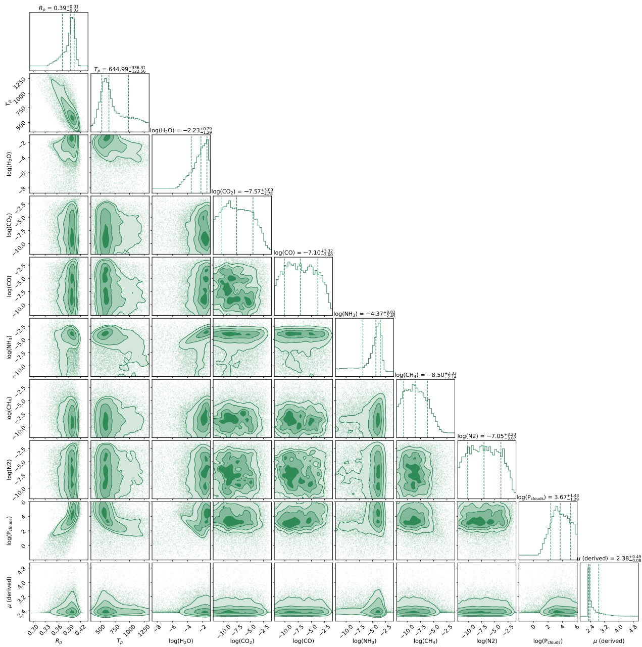
Figure 5.12: Posterior distributions including \text{N}_2 for the atmospheric retrieval on the extracted HD 106315 c spectrum.
