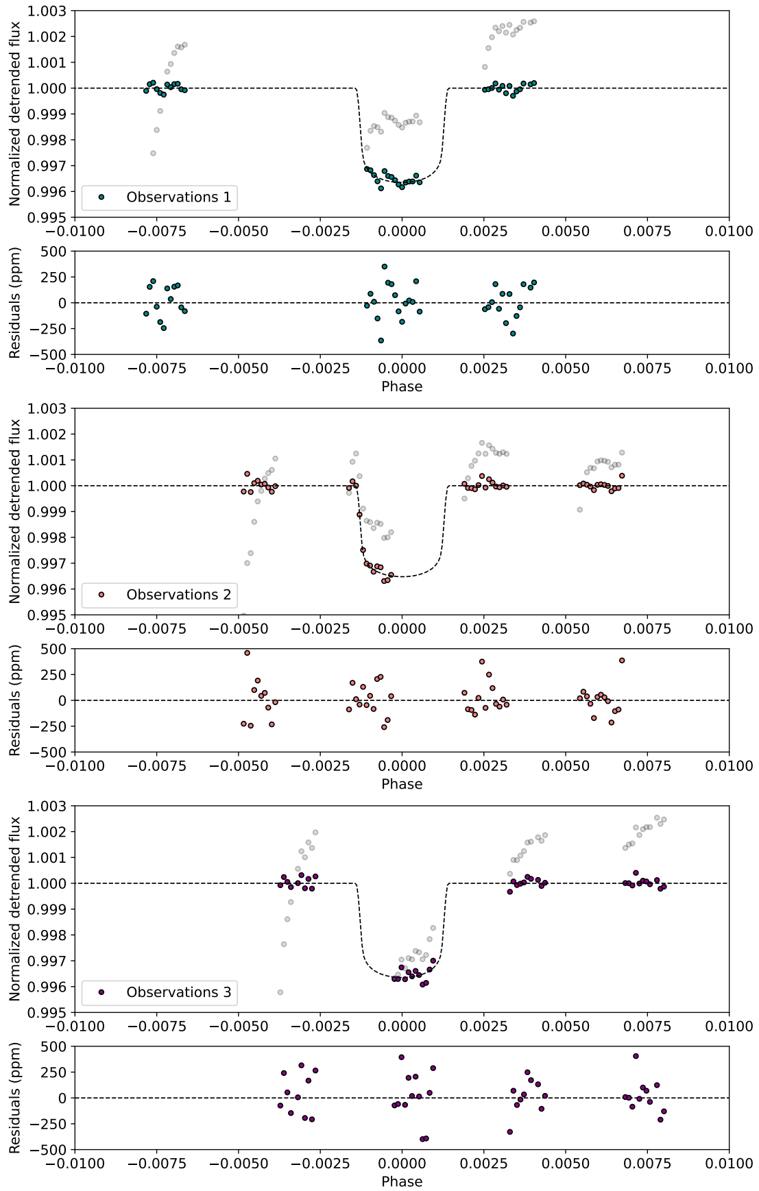
Figure 6.2: White light curve fits for the three observations on TRAPPIST-1h (top: July 2017, middle: September 2019, and bottom: July 2020). For every observation, we show the raw (grey), the de-trended flux (colour points) and the best-fit model (dotted lines) along with the residuals from the best-fit model.
