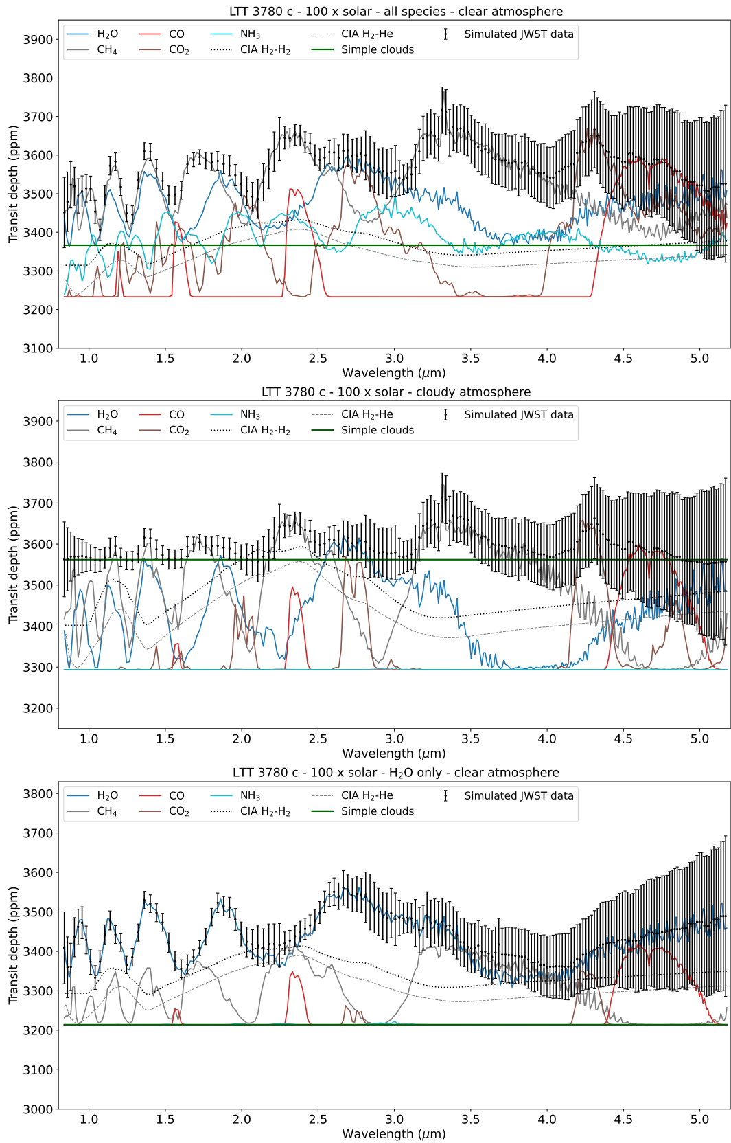
Figure 9.9: Best-fit opacity contributions to the JWST simulated transmission spectra of LTT 3780 c. We use Pandexo for the JWST observations based on Exo-REM simulations assuming a 100 \times solar atmospheric composition for a clear atmosphere (top), a cloudy atmosphere (middle) and a H 2 O only atmosphere (bottom). The mock retrieval analysis is performed with Tau-REX 3 .
