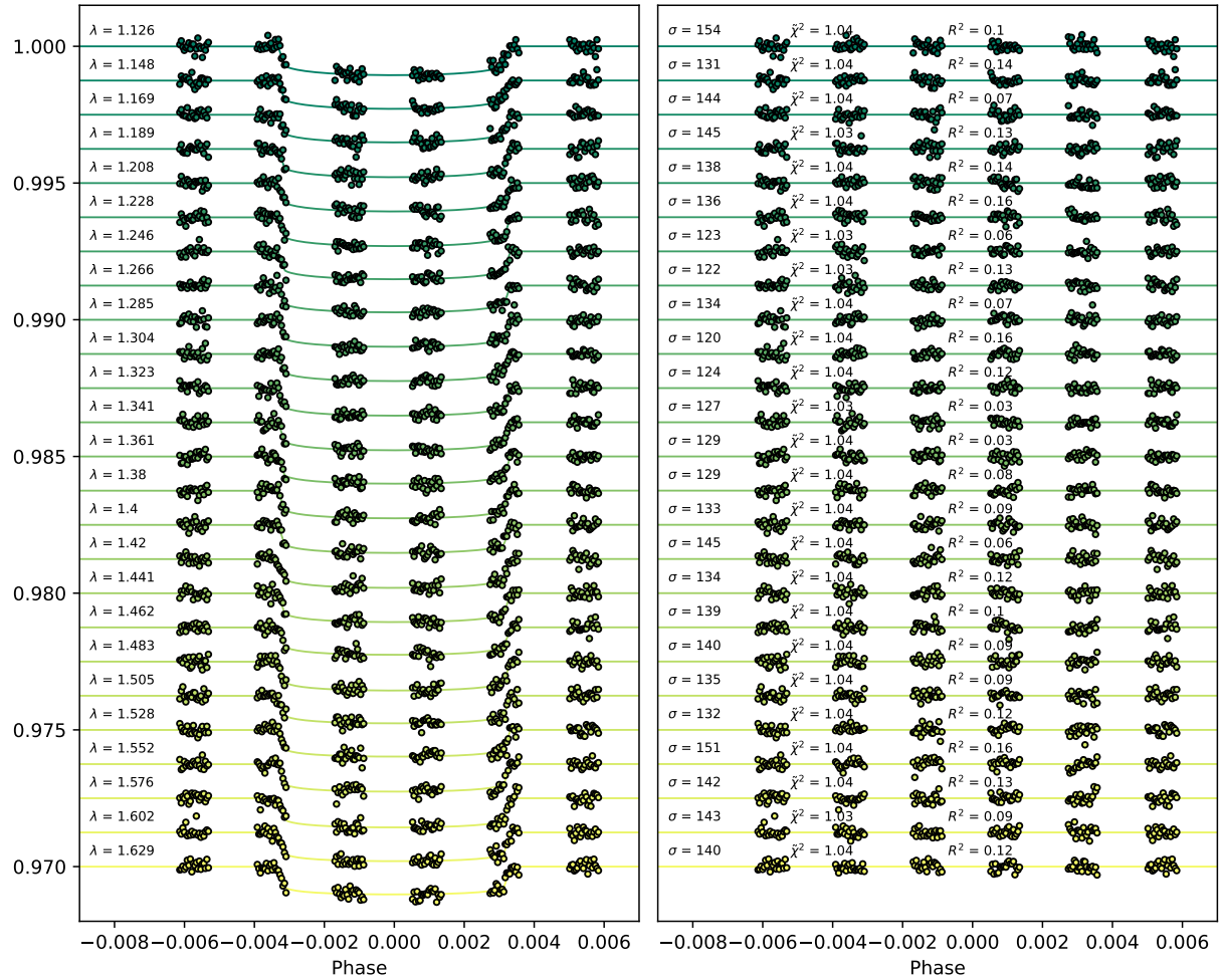
Figure 5.5: Spectral light curve fits for the first observation on HD 3167 c. An artificial offset in the y-axis was applied for clarity. For each light curve, the left panel shows the de-trended spectral light curves with the best-fit model in dotted lines, and the right panel shows the residuals and values for the standard deviation ( \sigma ) in ppm, the reduced Chi-squared ( \tilde{\chi}^2 ), and the auto-correlation ( R^2 ).
