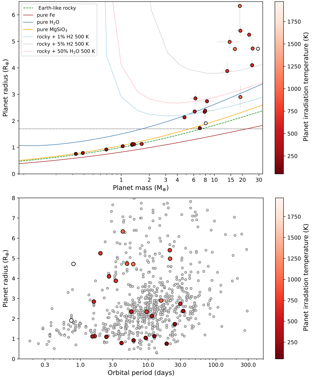
Figure 7.1: Mass radius measurements as a function of the irradiation temperature for planets studied here (top). Models compositions are from Zeng et al. (2019), and the horizontal dotted lines are set to the radius gap from Fulton et al. (2017). Distribution of the orbital period and the radius for planets in the sample (bottom). Known transiting planets with a published mass are shown in grey.
