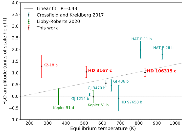
Figure 5.11: Normalized H 2 O amplitude in units of scale height as a function of equilibrium temperatures. Blue points are from Crossfield & Kreidberg (2017) and green points are from Libby-Roberts et al. (2020). Red points are computed using the method described in Crossfield & Kreidberg (2017) and spectra obtained in this work and from Tsiraras et al. (2018) for K2-18 b. The dotted line corresponds to a linear fit. The correlation coefficient was found to be lower than in Crossfield & Kreidberg (2017), 0.43 compared to 0.83.
