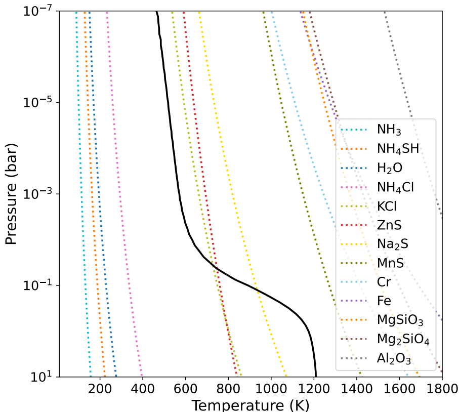
Figure 8.8: Simulated temperature-pressure profiles for GJ 3470 b (solid black lines) and condensation profiles (dotted lines) using Exo-REM. GJ 3470 b’s atmosphere is computed for a 1 × solar metallicity composition.
