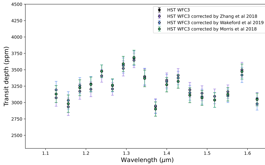
Figure C.2: Combined transit depth in ppm using the three HST/WFC3 G141 transit observations and corrected transit depth using stellar contamination models from Zhang et al. (2018) (purple), Wakeford et al. (2019) (blue), and Morris et al. (2018) (green). The latter (in green) and the raw extracted spectrum (in black) are almost similar because the stellar contribution of Morris et al. (2018) is flat in the HST/WFC3 NIR wavelength range.
