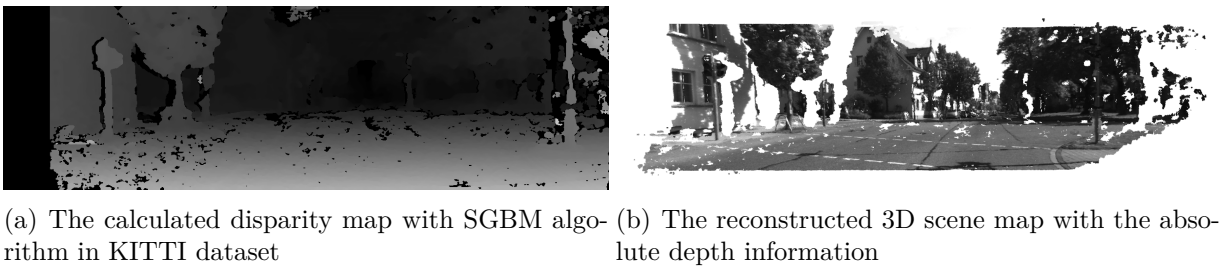
Figure 2.18 – The disparity map and depth-aware scene reconstruction results in KITTI dataset
