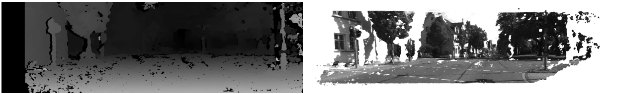
(a) The calculated disparity map with SGBM algorithm in KITTI dataset (b) The reconstructed 3D scene map with the absolute depth information
