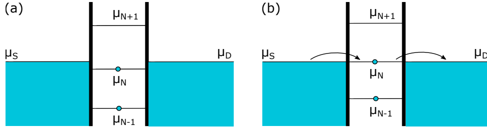
Figure 3.2 – Energy diagram of a single quantum dot system in the Coulomb blockade regime. Two tunnel barriers connect the quantum dot with the source and drain electron reservoirs. (a) The transport through the system is blocked. The next unoccupied energy level in the dot lies higher than the electrochemical potential of the source, so that \mu_N < \mu_D and \mu_{N+1} > \mu_S , and as a result no electron can tunnel through the dot. The system is in Coulomb blockade. (b) The transport through the system is activated. The electrochemical potential of the quantum dot is between the electrochemical potential of the source and drain, so that \mu_S > \mu_N > \mu_D , and electrons tunnel through the dot one by one.
