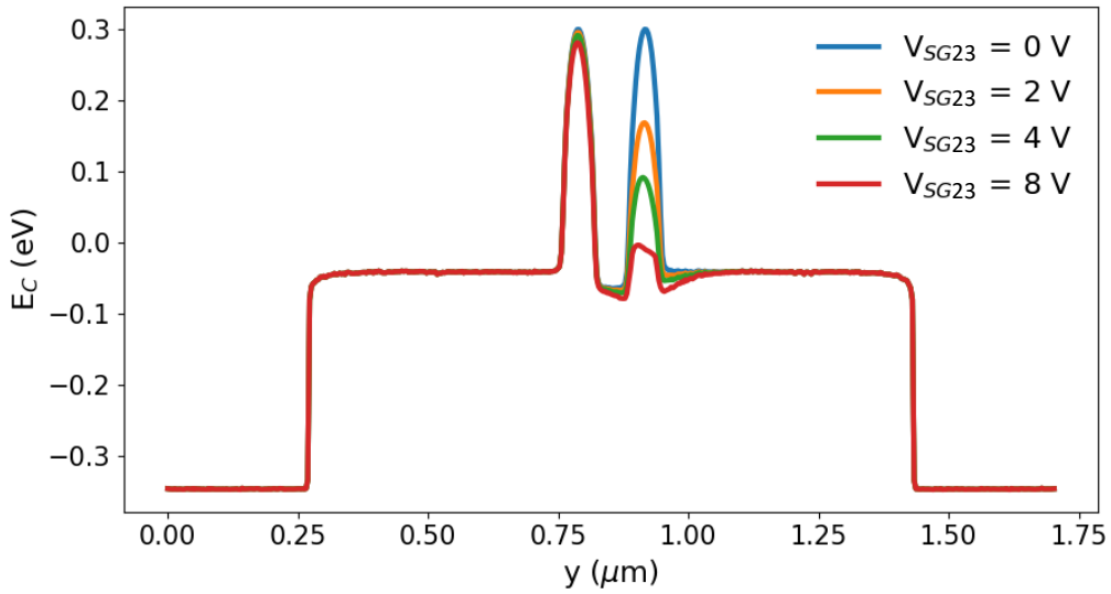
Figure 6.4 – Simulated conduction band edge using the QTCAD simulation software. Linecut taken at 1 \text{ \AA} below the top gate oxide into the conduction channel parallel to the transport. A 2DEG at the Si/SiO 2 interface is observed, along with the ability to tune the potential barrier height by applying the appropriate voltages to the lateral gates. A voltage sweep is performed on the gate SG3 and SG4 simultaneously with the back gate grounded. The voltage applied to the gates FGT and FGB is equal to 1 V, to the rest of the side gates 8 V, and to the DOT gate 1.2 V. The zero of energy corresponds to the Fermi level.
