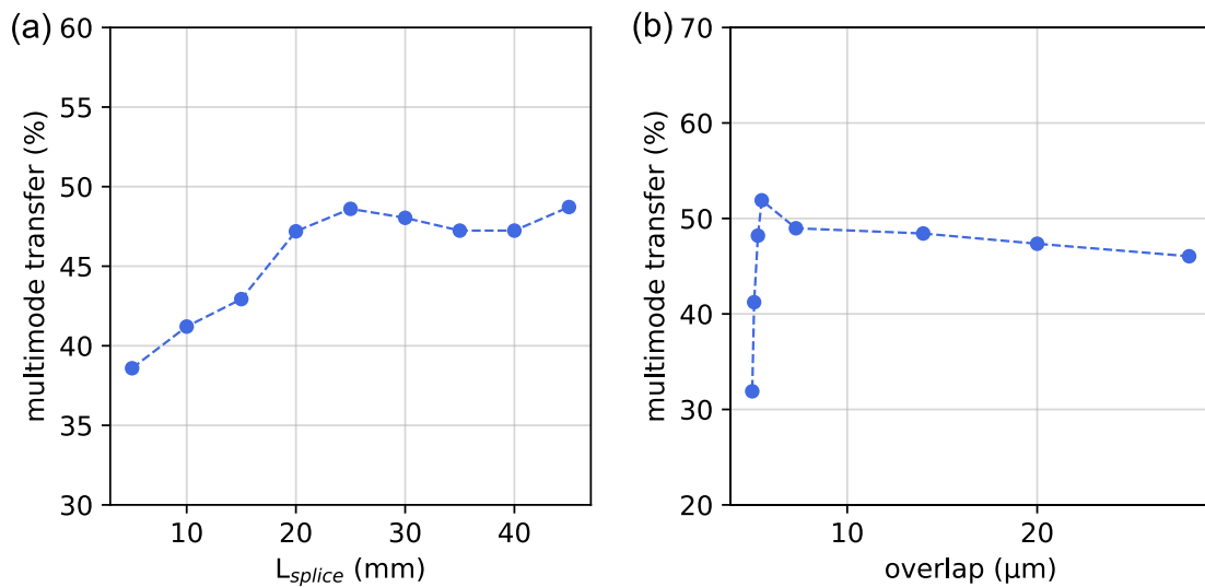
Figure 5.10: Measured multimode transfer of a HC-DCFC with a 300 \mu\text{m} outer diameter DC-HCF and a 500 \mu\text{m} outer diameter borosilicate MMF as a function of (a) the coupler length L_{splice} and (b) the overlap parameter \delta .
