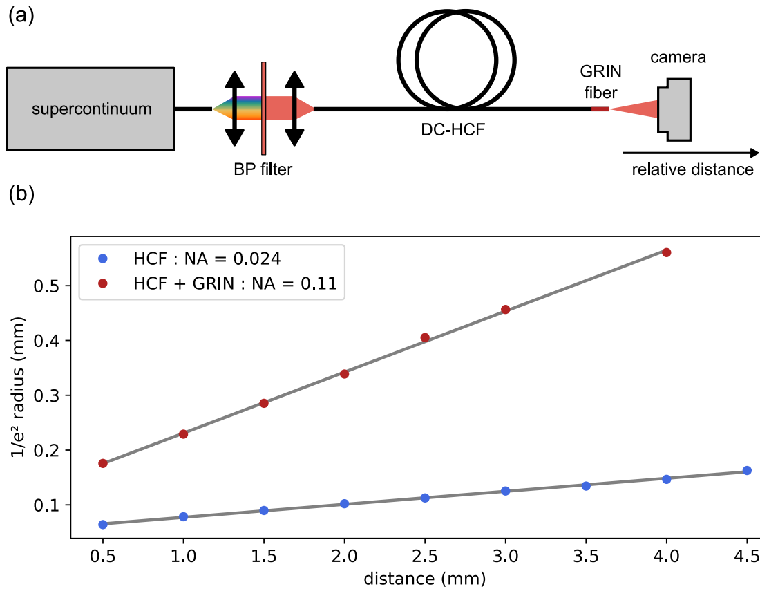
Figure 3.10: (a) Schematic representation of the setup used to measure the NA of the DC-HCF with a GRIN lens spliced at its distal end. (b) Measured 1/e^2 radius as a function of the relative camera position at \lambda = 920 \text{ nm} and for the DC-HCF with (red) and without (blue) the GRIN lens.
