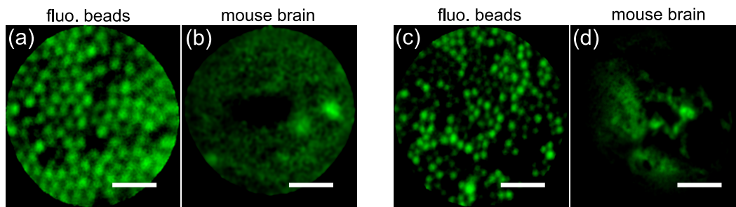
Figure 3.23: 2PEF imaging comparison of the endoscope based on a (a, b) bead or (c, d) GRIN functionalization. Scale bars are respectively: (a) 10 \mu\text{m} , (b) 25 \mu\text{m} , (c) 20 \mu\text{m} and (d) 40 \mu\text{m} . Excitation average power on the samples are respectively: (a) 18 \text{ mW} , (b) 34 \text{ mW} , (c) 10 \text{ mW} and (d) 28 \text{ mW} . Images are recorded with a 2 FPS acquisition rate and averaged over 5 images.
