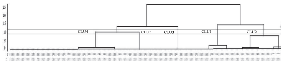
Figure 2-13 Dendrogram result from clustering farms according to the values of the variables in 2010
