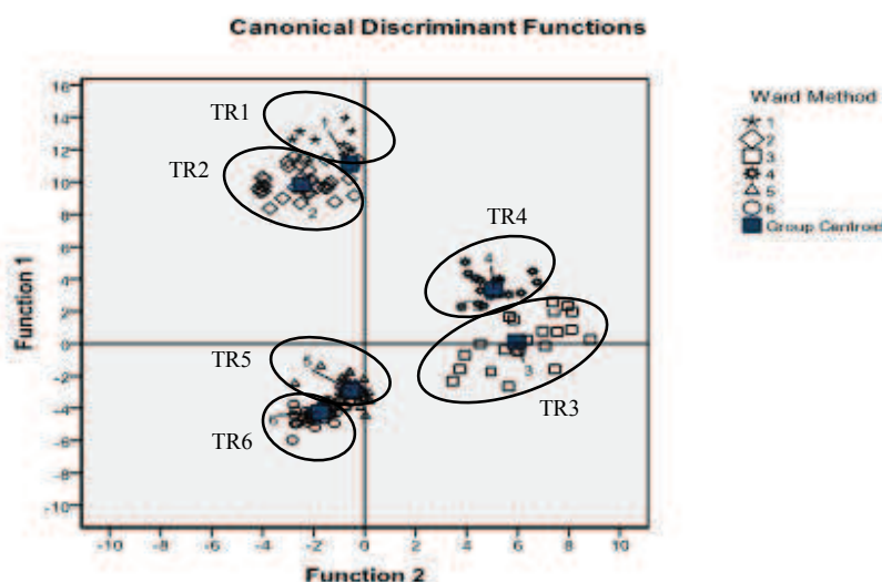
Figure 2-12 Canonical discrimination functions of six-farm trajectories
