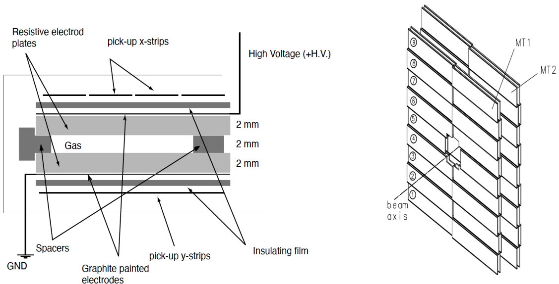
Figure 2.5: (left) Schematic cross-section view of a resistive-plate chamber. (right) Layout of the two trigger stations. Figures extracted from the technical design report [41].
