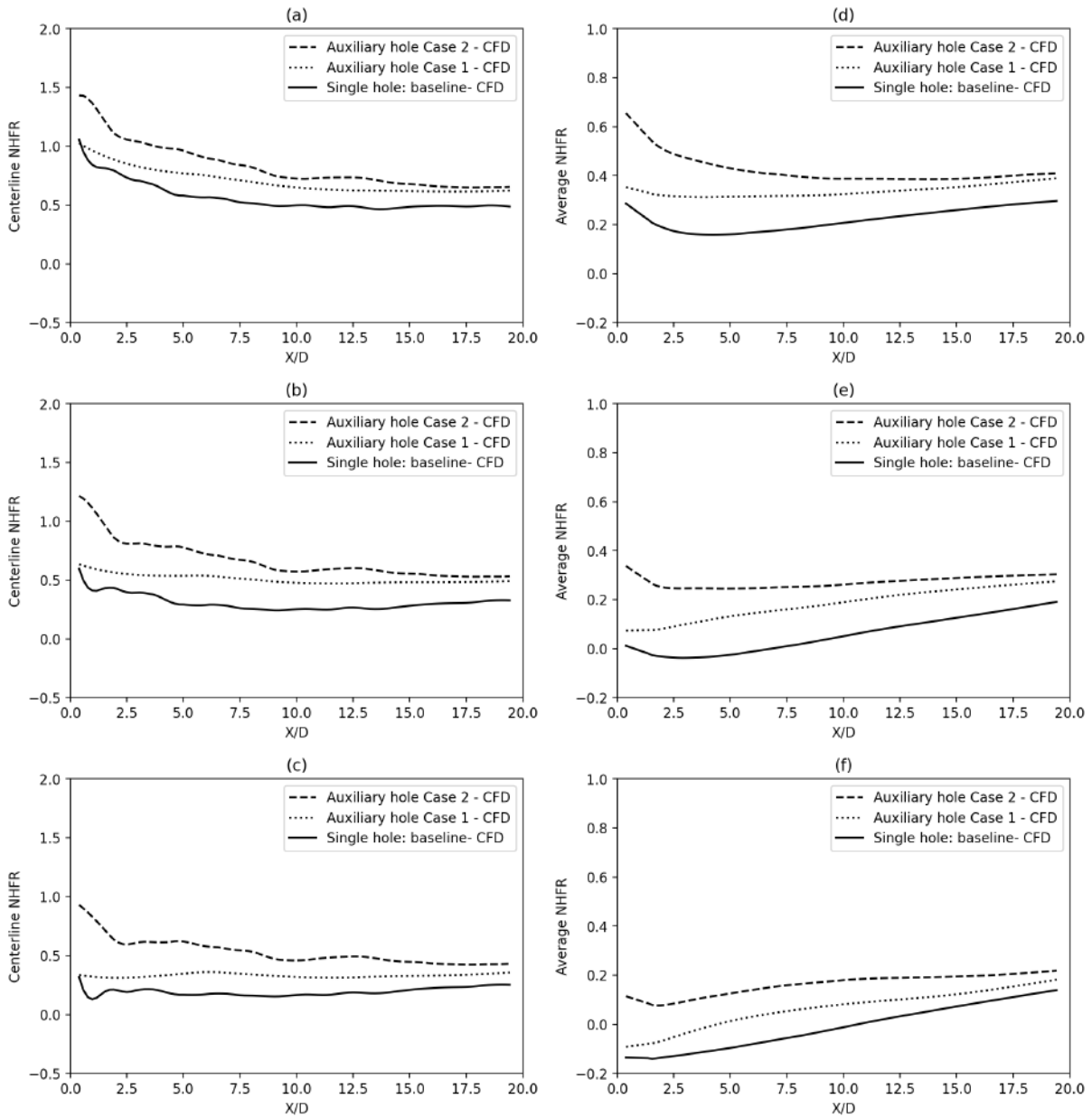
Figure 3.13: Evolution of centerline (a-c) and laterally averaged NHFR (d-f) values along the longitudinal axis (X-axis) for various blowing ratios. (a,d) M=0.65 (b,e) M=1 (c,f) M=1.25
