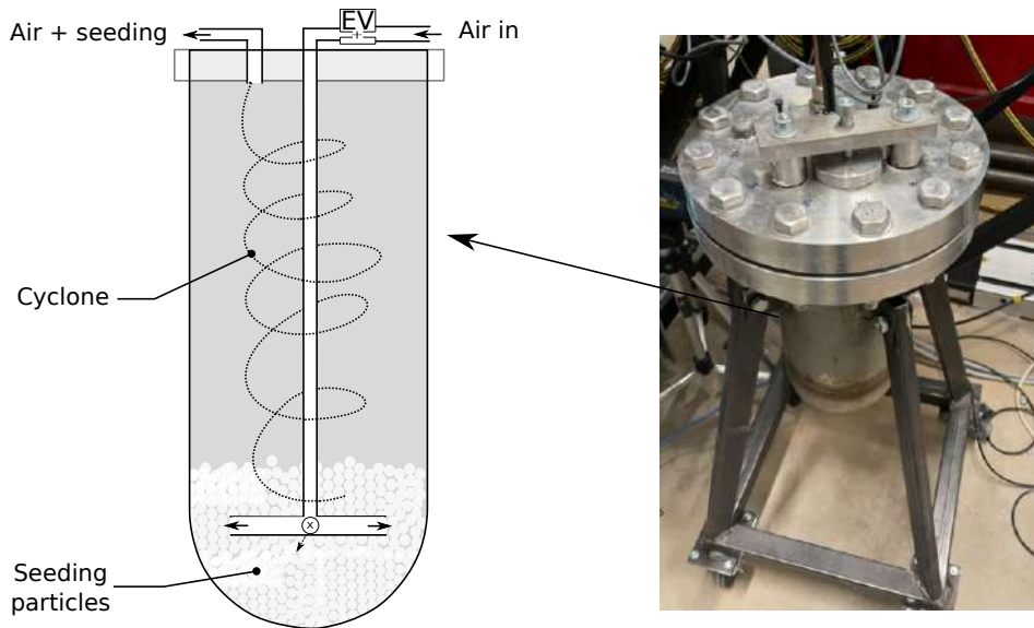
Figure 5.10: Picture showing the seeding chamber with supports.
