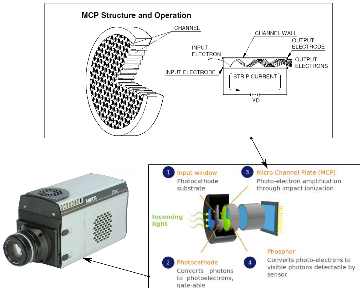
Figure 5.27: Andor iStar sCMOS camera: Depiction of various parts in the intensifier and the functioning of Micro Channel Plate.
