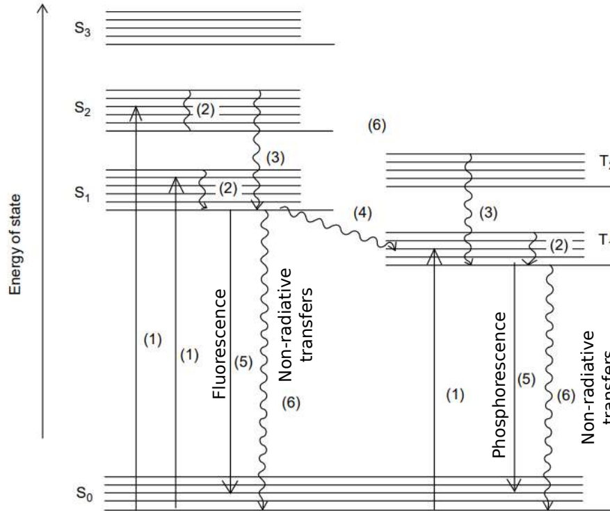
Figure 4.3: The Jablonski diagram to represent the transitions between the energy states of an electron. (1) light absorption, (2) vibrational relaxation, (3) internal conversion (IC), (4) intersystem crossing (ISC), (5) radiative transition, and (6) non-radiative transition Shigeo Shionoya (2006)
