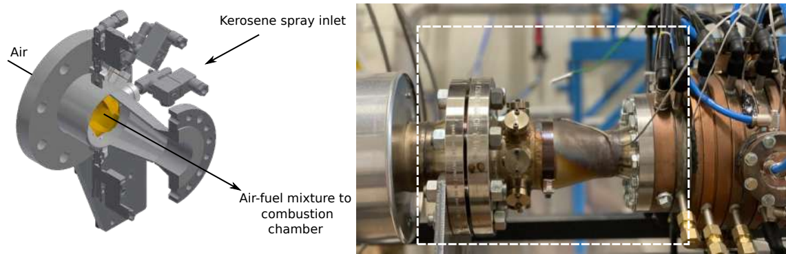
Figure 5.6: CAD view of the premix chamber with the injectors. Right picture shows the actual view of the pre-mix chamber
