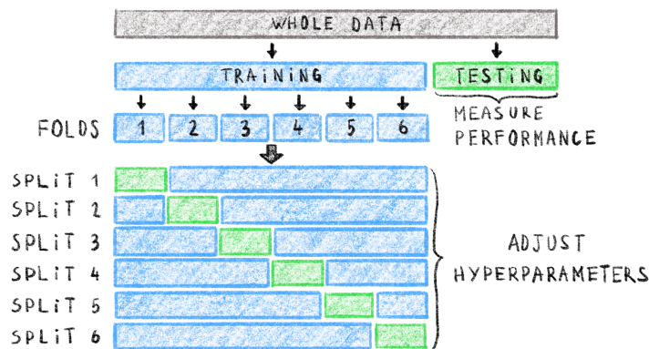
Figure 4.2.: Example of data splits into training, testing and validation sets with 6-fold cross-validation.
