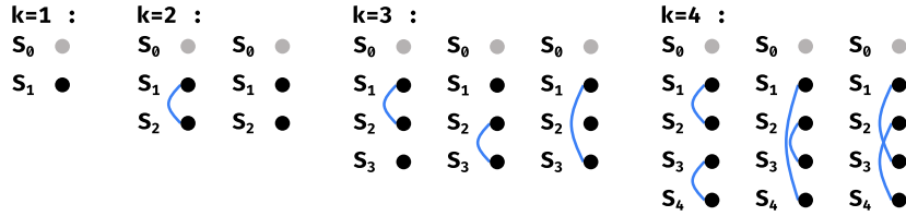
Figure 3.2.: SSR equivalence classes for a fixed partition of the inputs.
