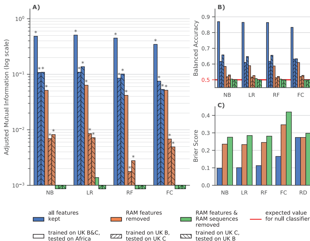
Figure 6.1.: Classifier Performance on UK and African datasets.
