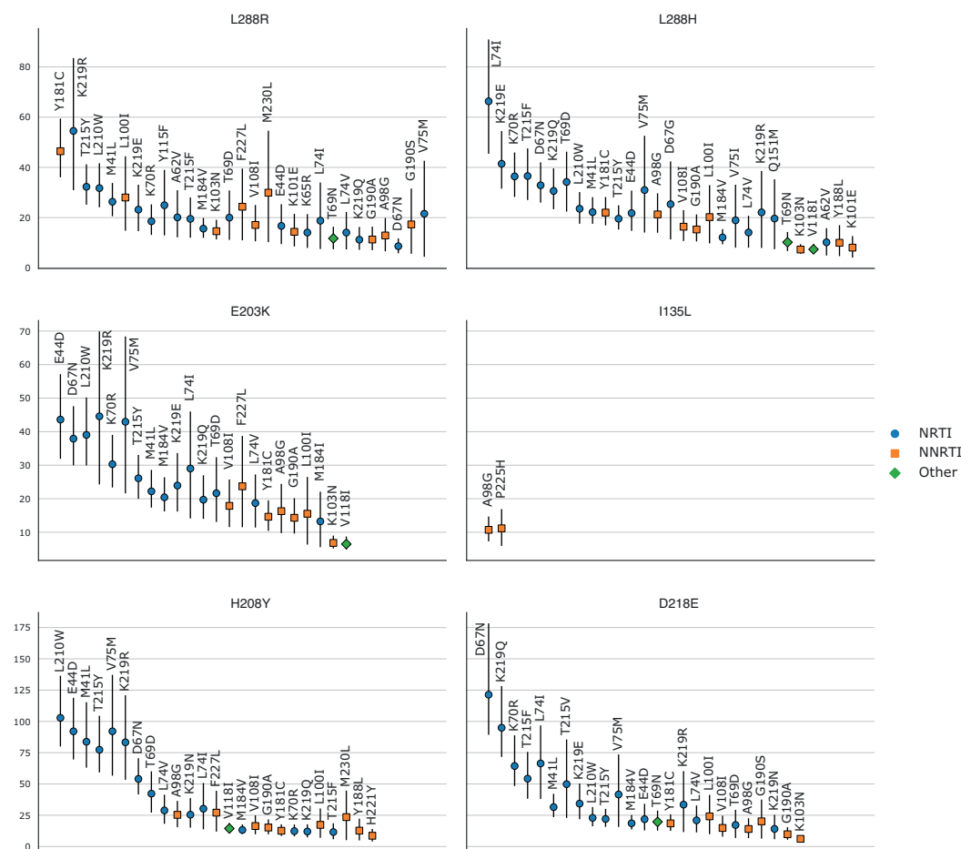
Figure 6.3.: Relative risk of the new mutations with regards to known RAMs on the UK dataset.
