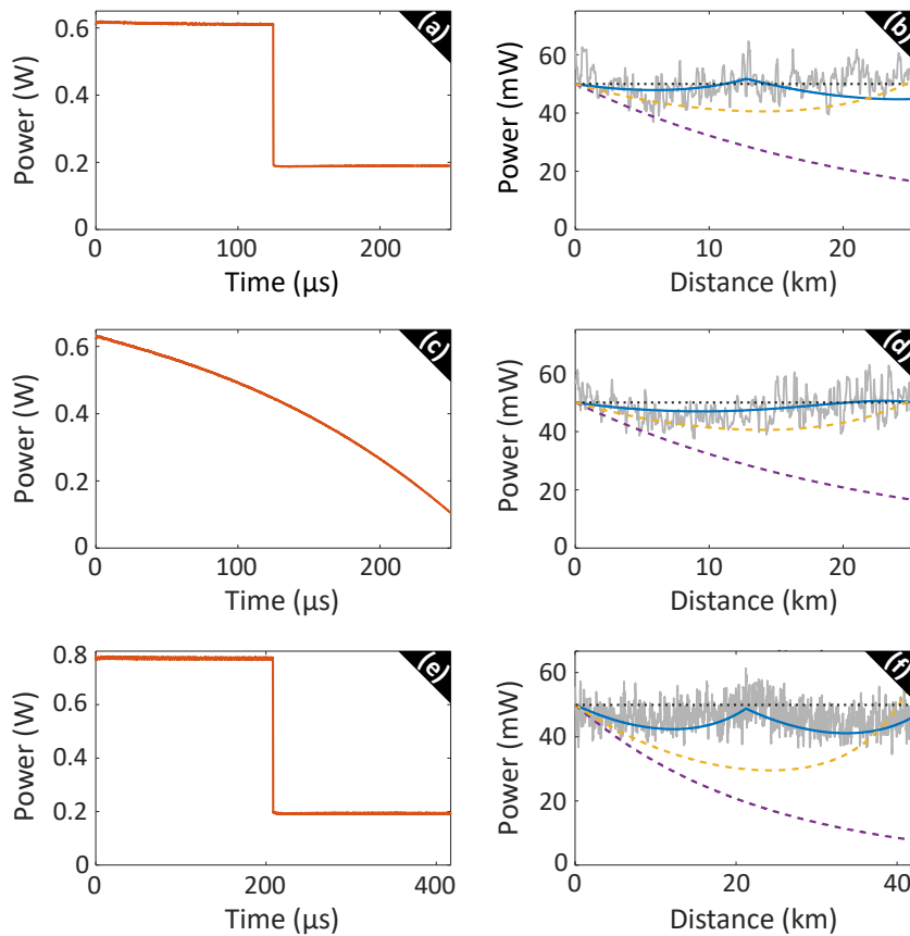
Figure C.3: (a)-(c)-(e) Experimental Raman pump pulse power profiles. (b)-(d)-(f) Corresponding power evolution of the amplified signal from experiments (grey solid line) and numerics (blue solid line). The dashed purple lines, the dashed yellow lines and the black dotted lines account for the Raman pump off, a constant Raman pump power and the propagation in a transparent fiber respectively.
