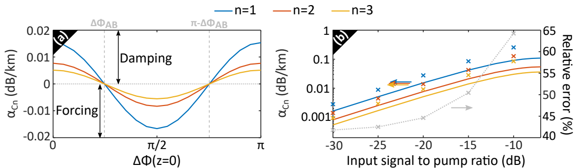
Figure 6.2: Evolution of \alpha_{cn} from the 3WM model Hamiltonian for n = \{1, 2, 3\} as a function of (a) the initial relative phase with \frac{P_s(z=0)}{P_p(z=0)} = -20 dB, and (b) the input signal to pump ratio with \Delta\Phi(z = 0) = 0 . In addition to the 3WM model (solid lines), \alpha_{cn} are calculated from damping NLSE numerics and displayed in (b) (crosses), with the corresponding relative error (grey crosses and dotted line). The other parameters are the same as in Fig. 6.1.
