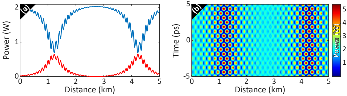
Figure 7.6: Coherently-driven MI in DOFs. (a) Power evolution of the pump (solid blue line) and signal (solid red line) along the fiber length. (b) Power space-time profile. Parameters: \beta_{2,avg} = \pm 2 \text{ ps}^2/\text{km} , \beta_{2,amp} = 1.5 \text{ ps}^2/\text{km} , \gamma = 5 \text{ W}^{-1}\text{km}^{-1} , L = 1 \text{ km} , Z = 100 \text{ m} , P_p(z=0) = 2 \text{ W} , \frac{P_{s,i}(z=0)}{P_p(z=0)} = -20 \text{ dB} , f_m = 802 \text{ GHz} and \Delta\Phi(z=0) = \frac{\pi}{2} .
