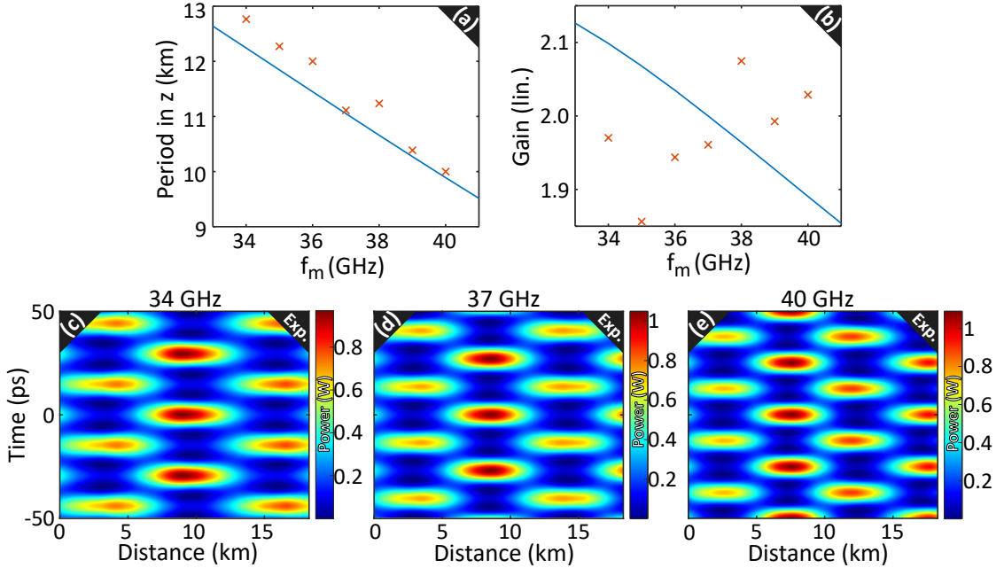
Figure 4.8: Evolutions according to f_m of (a) the spatial period and (b) the gain. Experimental data are displayed in oranges crosses and analytical ones in solid blue lines. Experimental space-time evolutions of the power for (c) f_m = 34 GHz ( \omega_m = 2.024 ), (d) f_m = 37 GHz ( \omega_m = 2.202 ) and f_m = 40 GHz ( \omega_m = 2.381 ).
