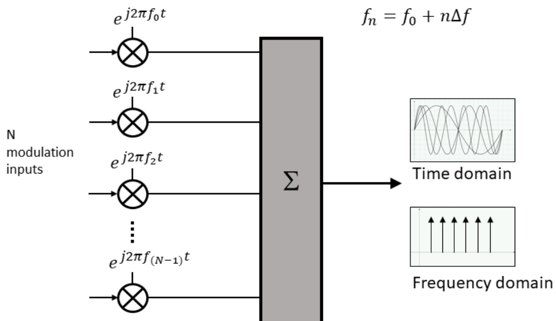
FIGURE 1.13: OFDM modulator.
