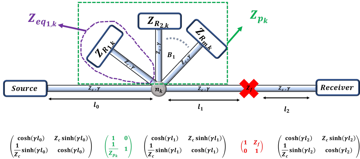
FIGURE 1.8: Cascaded ABCD-matrices.
