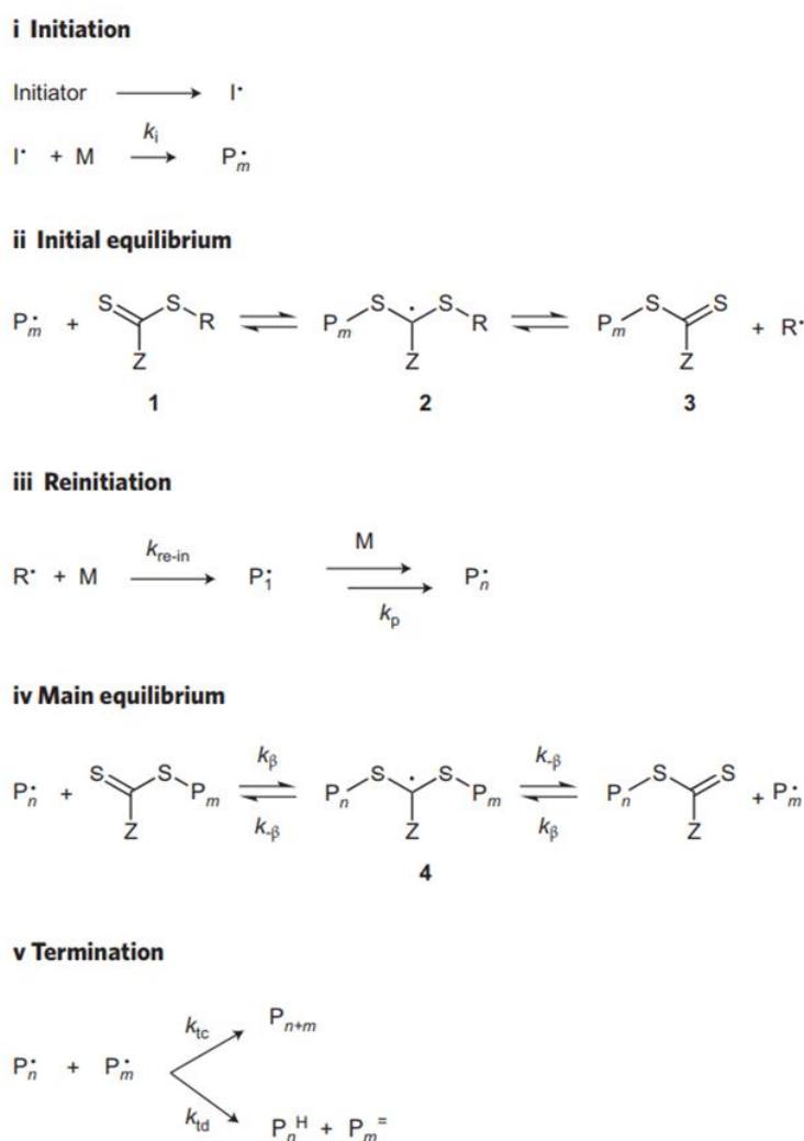
Figure 1.15. Mechanism of RAFT-polymerization based on M. Semsarilar et al. Reprinted by permission from ref. 110 Copyright 2019, Springer Nature.
