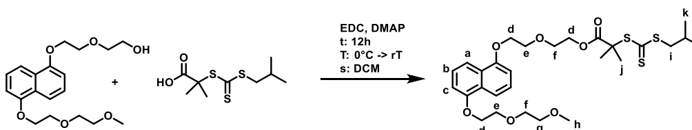
Figure 2.36. Reaction conditions for the synthesis of Napht-CTA with respective 1 H-NMR annotations.
