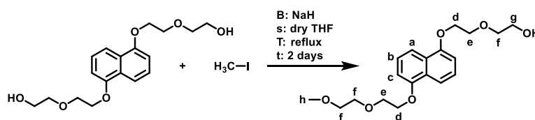
Figure 2.35. Synthetic scheme for the synthesis of NaphtOMe with respective 1 H-NMR annotations.
