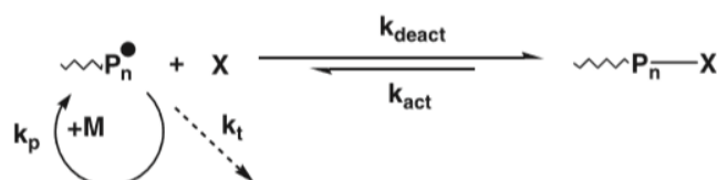
Figure 1.12. Deactivation/activation process of the growing polymer chain controlled via stable radicals. Reprinted from ref. 102 Copyright 2019, with permission from Elsevier.
