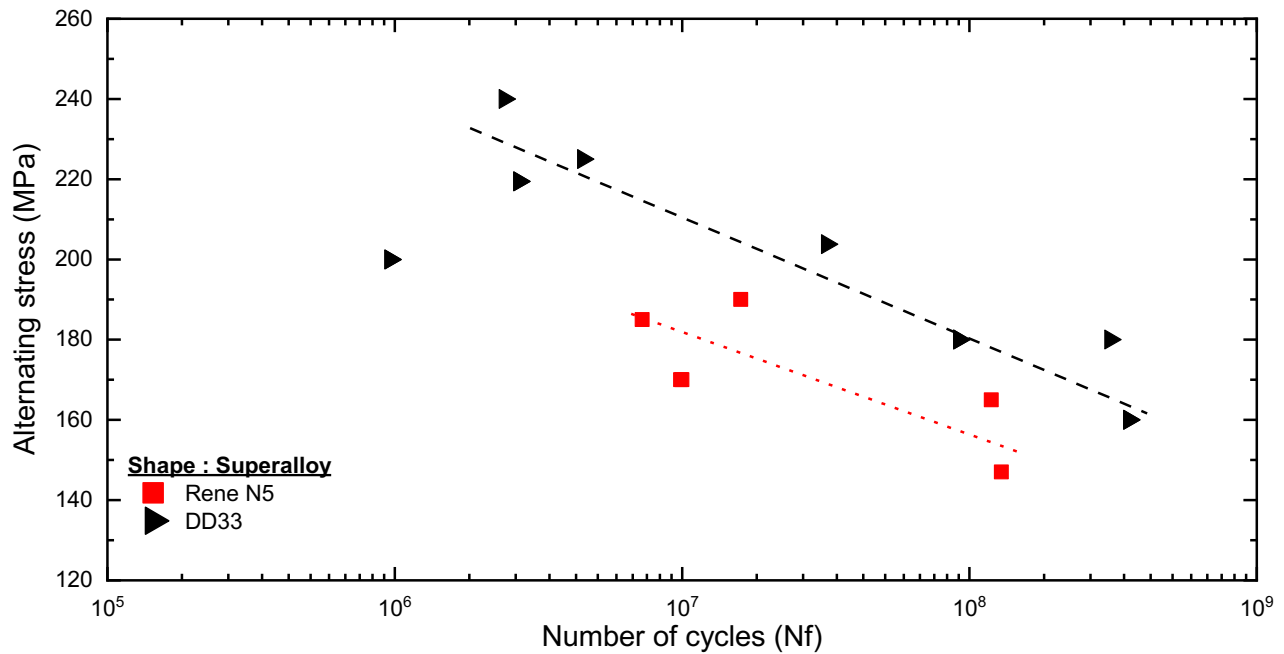
Figure A-1 S-N diagram for 1,000 °C, R_e = -1 , and f = 20 kHz gathering the results from the samples machined from the DD33 and Rene N5 Bridgman solidified rods. The alternating stress is plotted as a function of the number of cycles to failure.
