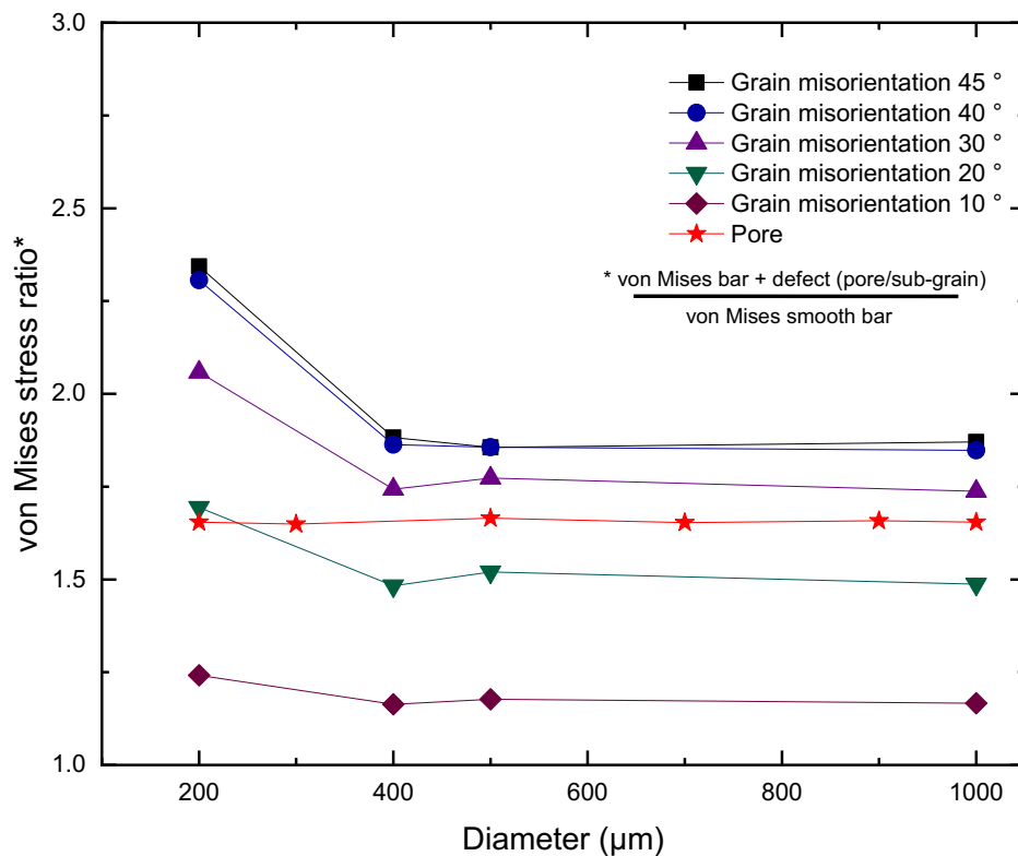
Figure III-14 Finite element results using the Abaqus software for a spherical grain having a diameter between 200 - 1,000 \mu\text{m} and primary misorientation ( \theta ) in the range of 10 - 45^\circ , and a spherical casting pore designed with diameter between 200 - 1,000 \mu\text{m} .
