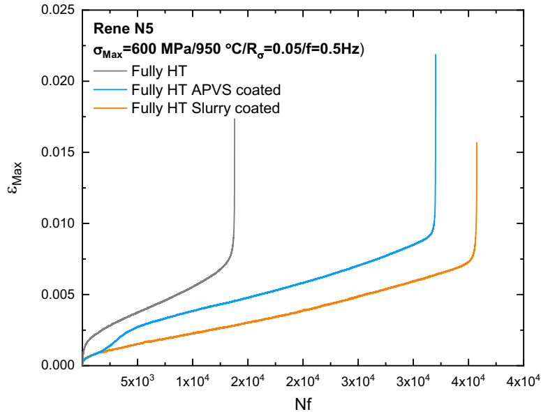
Figure IV-14 Evolution of the maximum mechanical strain as a function of the number of cycles for the Rene N5 superalloy at \sigma_{Max}=600 MPa/950 °C, R_\sigma = 0.05 , and f = 0.5 Hz, with and without a NiAl bond coat.
