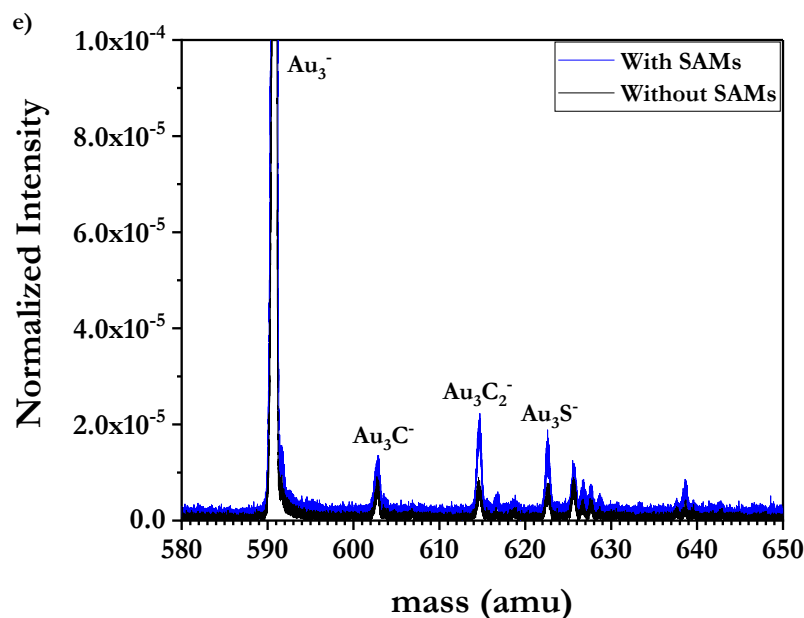
Figure 34. Mass spectra of precleaned Au functionalized with Im-C 11 -SH SAMs and adsorbed Rh(III) (blue line), and precleaned non-functionalized Au with adsorbed Rh(III) (black line). [Rh] init = 9.7 \mu M, [HCl] = 0.55 M. (a) Mass range of 200 – 290 amu showing characteristic peaks of RhCl 3 - , RhCl 4 - and RhCl 5 - clusters. (b) Mass range of 206 – 216 amu showing zoomed-in ions of RhCl 3 - clusters and their interference with other ions. (c) Mass range of 242 – 252 amu showing zoomed-in ions of RhCl 4 - clusters and their interference with other ions. (d) Mass range of 400 – 480 amu showing characteristic peaks of Rh 2 Cl 7 - and Rh 3 Cl 4 H - clusters. (e) Mass range of 580 – 650 amu showing a characteristic peak of Au 3 S - clusters important for the calculation of the coverage of Au with Im-C 11 -SH SAMs.
