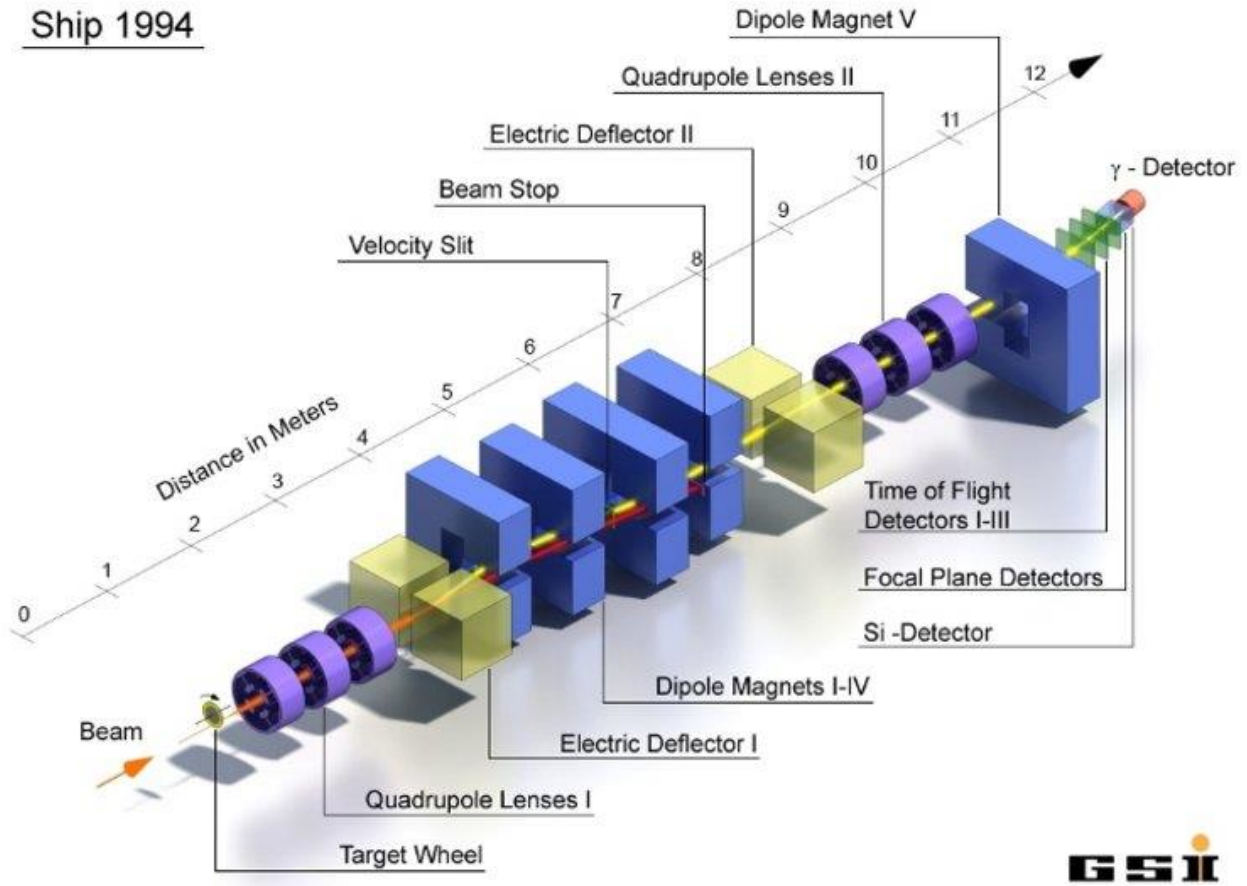
Figure 3. The schematic diagram of the velocity filter SHIP setup in its 1994 modified version. Reprinted from ref. [23].
