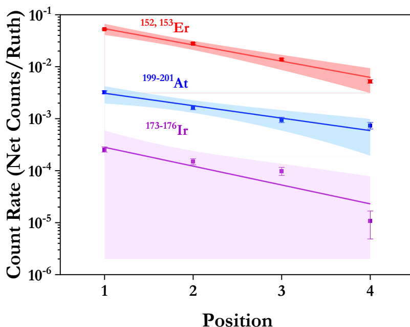
Figure 48. The count rate of ^{152,153}\text{Er} (red squares), ^{199-201}\text{At} (blue squares), and ^{173-176}\text{Ir} (purple squares) as a function of the detector position. The data were fitted using Eq. 22, the offset was set to zero. Shades represent 95% confidence bands.
