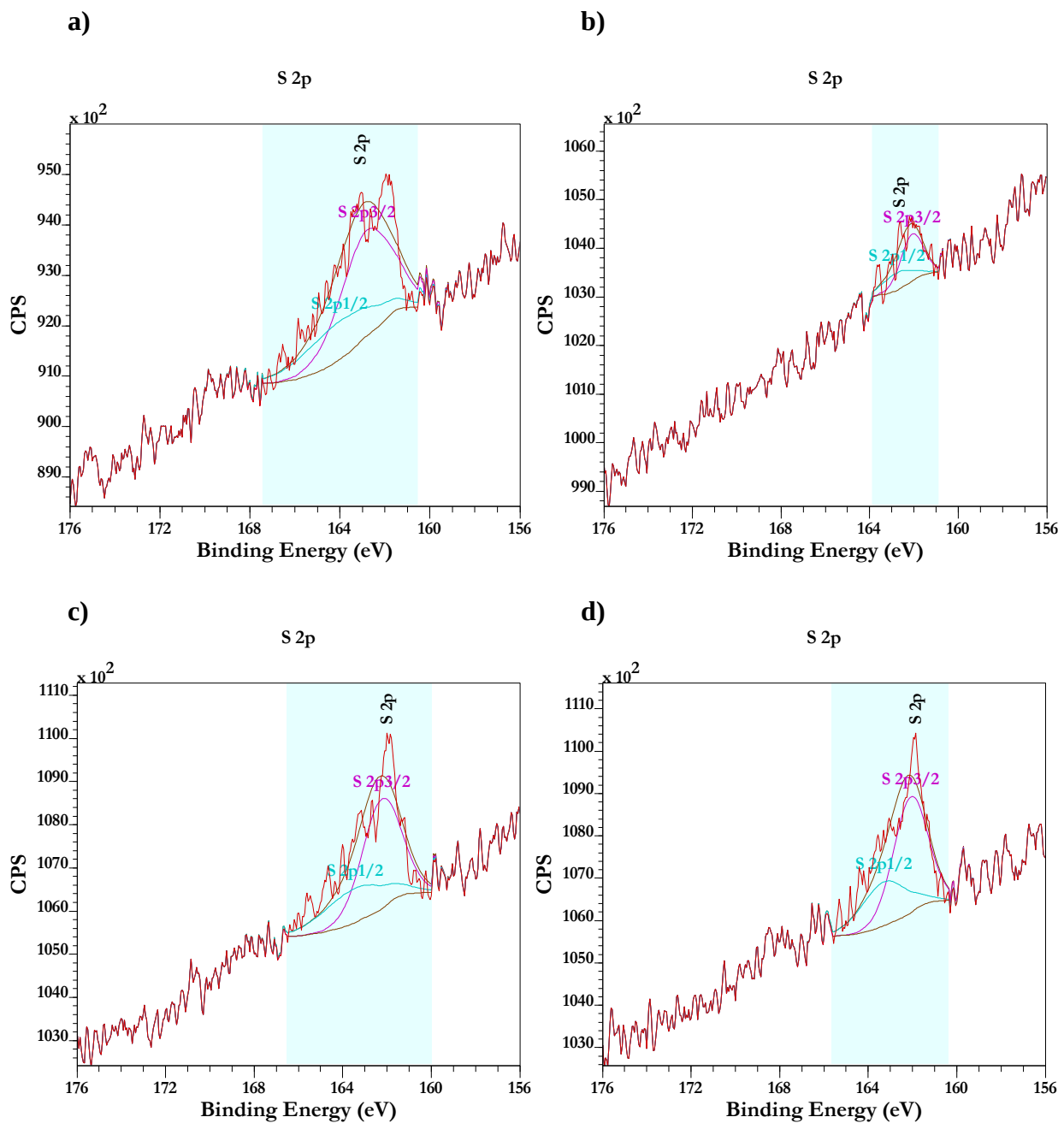
Figure 29. Sulfur 2p XPS for Im-C 11 -SH SAMs on precleaned Au; one SAMs deposition: (a) the freshly prepared SAMs; (b) SAMs removed using the liquid-UVPO treatment; (c) the freshly prepared sample stored for two weeks; (d) the freshly prepared sample stored for one month.
