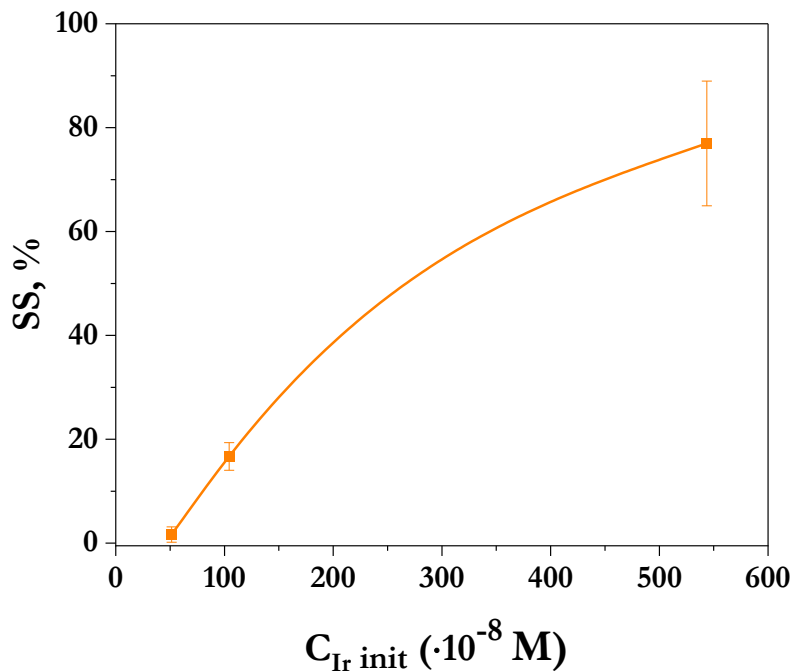
Figure 36. The surface saturation of Im-C 11 -SH SAMs with Ir(IV) as a function of the initial Ir(IV) concentration in 0.55 M HCl solutions. The line is drawn to guide the eye.
