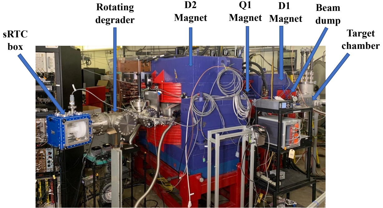
Figure 17. The AGGIE heavy element separator. Blue arrows show its main components.
