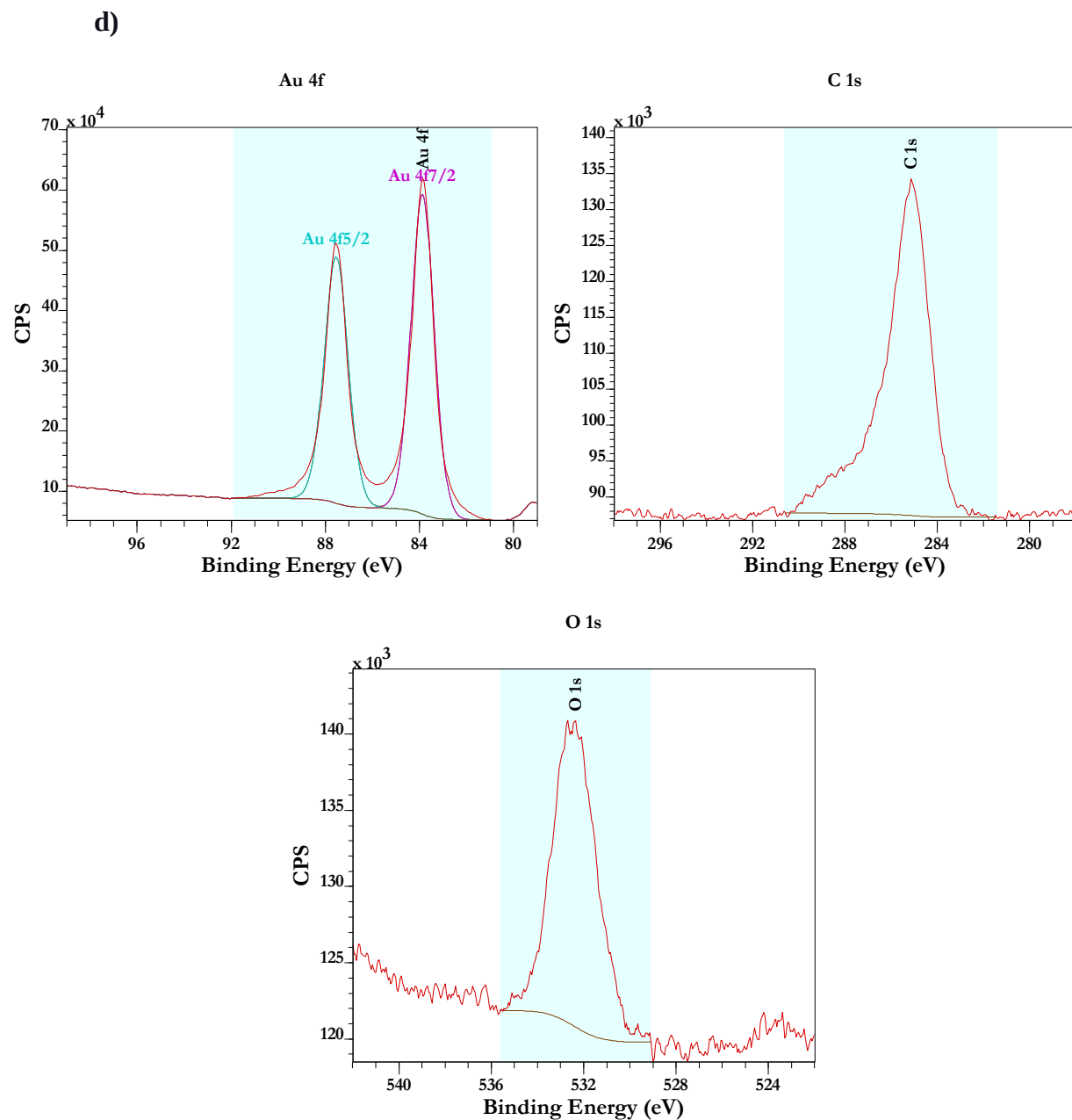
Figure A1. Gold 4f, carbon 1s, and oxygen 1s XPS for Im-C 11 -SH SAMs on precleaned Au; one SAMs deposition: (a) the freshly prepared SAMs; (b) SAMs removed using the liquid-UVPO treatment; (c) the freshly prepared sample stored for two weeks; (d) the freshly prepared sample stored for one month.
