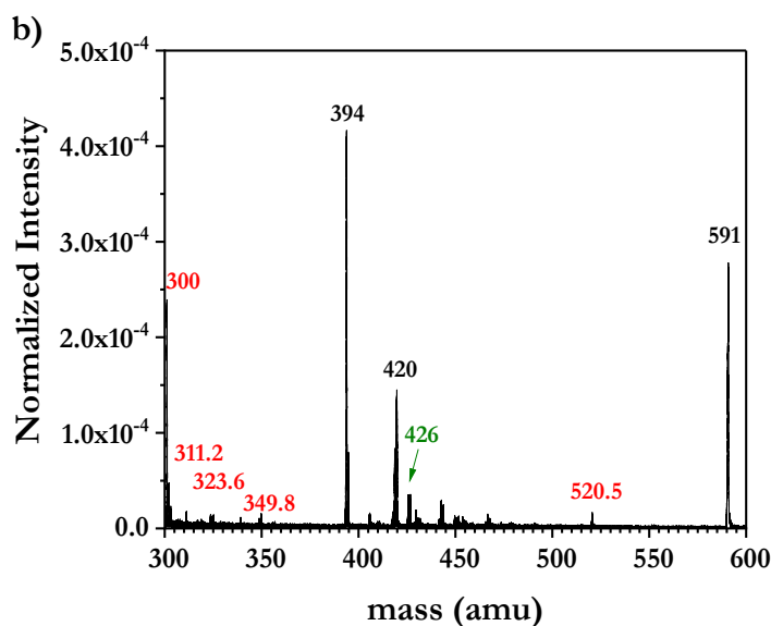
Figure 27. (a) Mass spectrum of non-precleaned Au functionalized with Im- \text{C}_{11} -SH SAMs deposited from a 1.6 mM ethanolic thiol solution during the first deposition. (b) Mass spectrum of pre-cleaned Au functionalized with Im- \text{C}_{11} -SH SAMs deposited from a 5 mM ethanolic thiol solution during the second deposition. Mass range of 300-600 amu.
