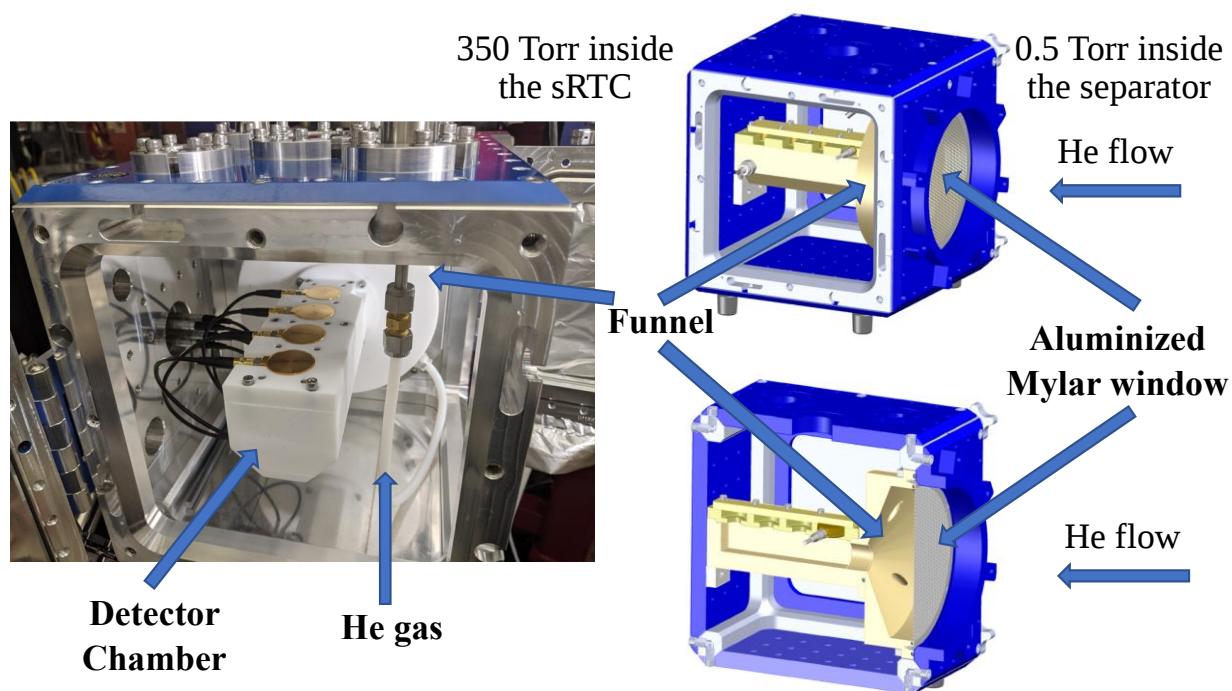
Figure 18. The left panel shows circular, gold-colored detectors installed inside the sRTC. The right panel shows schematic images of the sRTC including its cross-sectional view.
