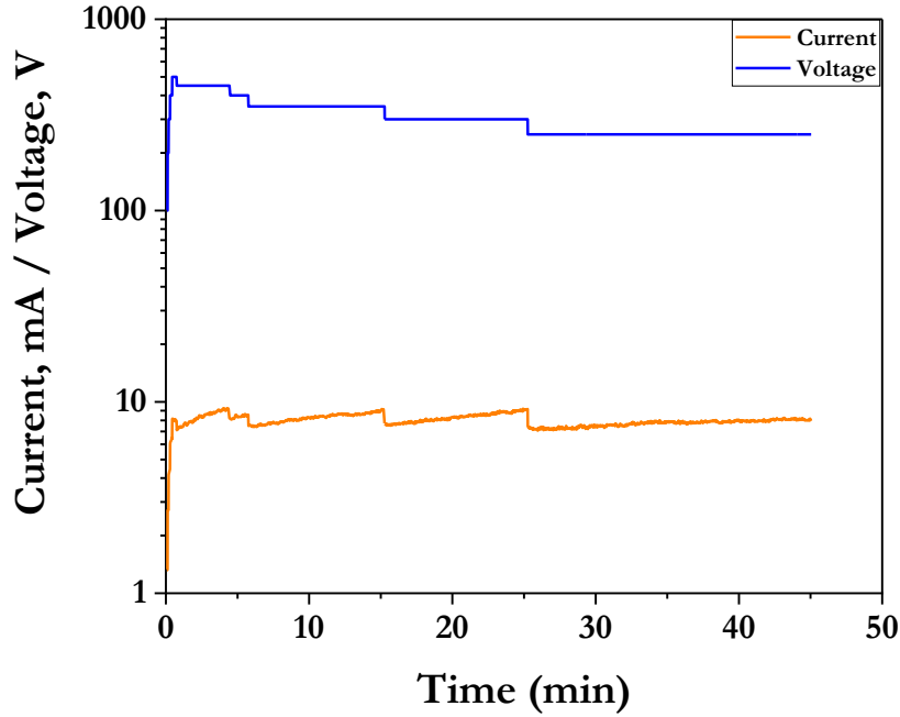
Figure 16. Current (orange curve) and voltage (blue curve) as a function of time.
