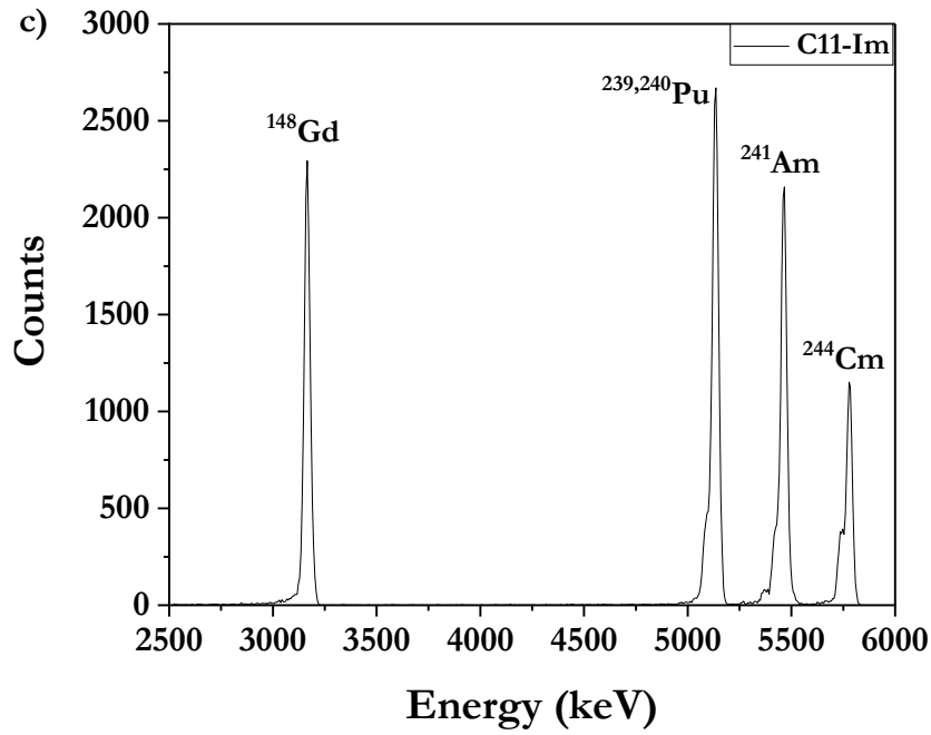
Figure 51. Alpha spectra of a four-peak alpha source collected on (a) the Bare Si; (b) the Si+Au; (c) the C11-Im detectors to measure their resolution.
