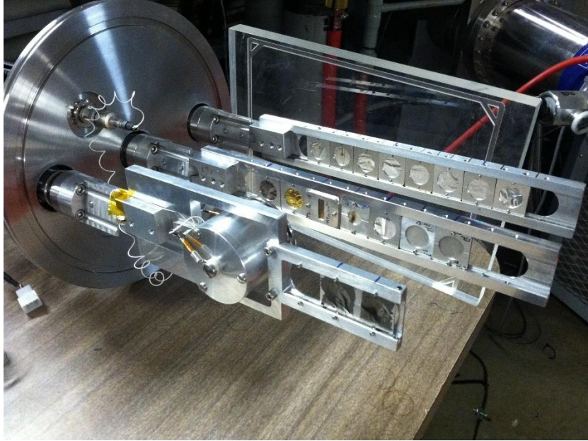
Figure 13. From top to bottom: degrader, target, and Faraday cup ladders. Reprinted from ref. [113].
