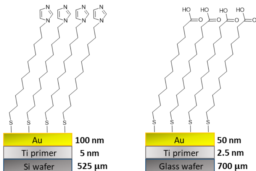
Figure 10. Schematic diagram of the substrates investigated in this study. All chips were 10 mm × 10 mm.
