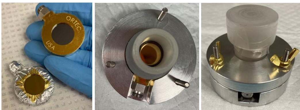
Figure 20. Silicon and gold-coated silicon detectors (left image), “chimney” placed onto the gold-coated silicon detector (center image), and the sealed “chimney” (right image).
