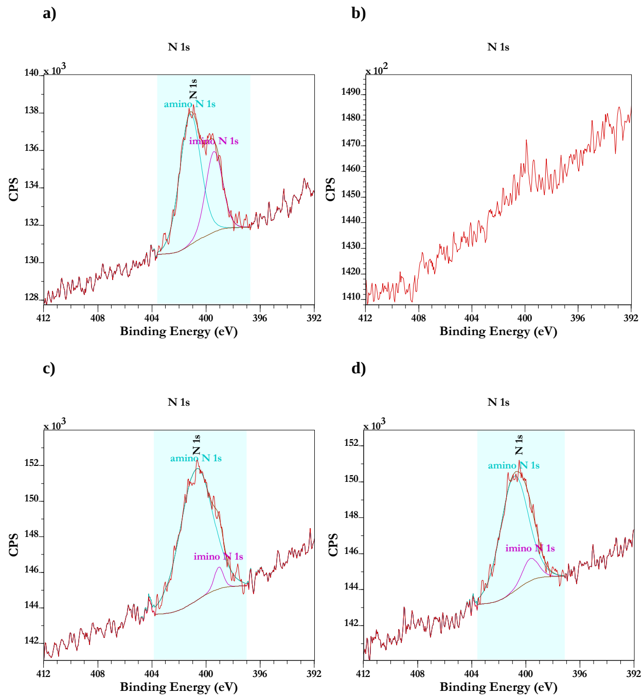
Figure 30. Nitrogen 1s XPS for Im-C 11 -SH SAMs on precleaned Au; one SAMs deposition: (a) the freshly prepared SAMs; (b) SAMs removed using the liquid-UVPO treatment; (c) the freshly prepared sample stored for two weeks; (d) the freshly prepared sample stored for one month.
