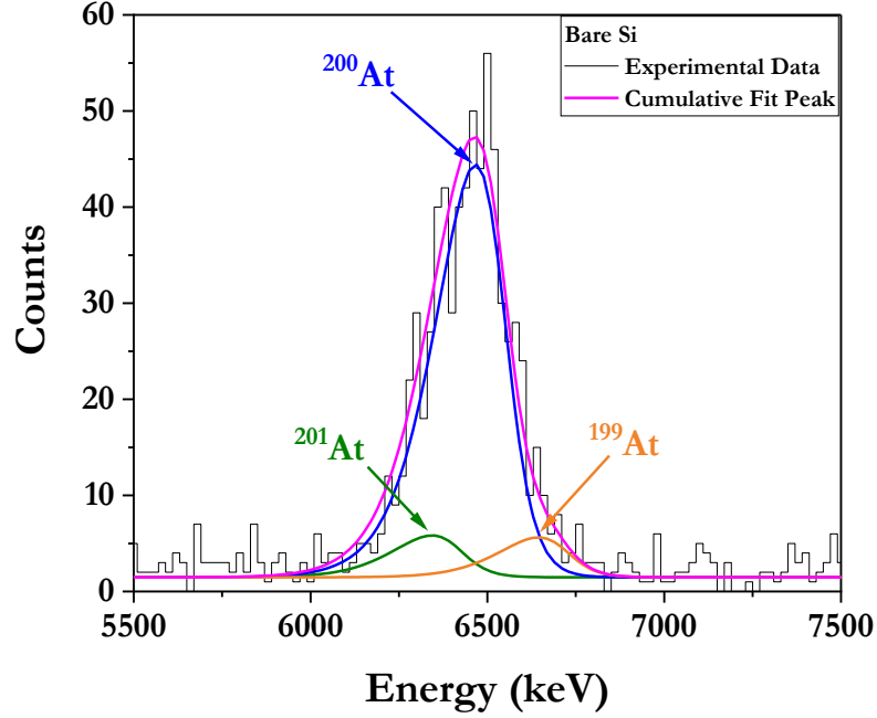
Figure 40. ^{199-201}\text{At} calibration spectrum (black histogram) collected on the vertical Bare Si detector with the rotating degrader at 90 degrees. Bin width: 20 keV. The peaks were fitted using Eq. 13.
