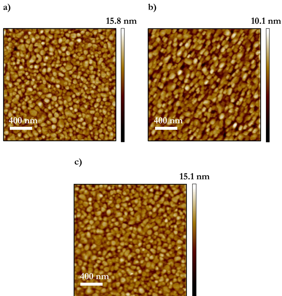
Figure 24. AFM images ( 2 \times 2 \mu\text{m} ) of (a) pure precleaned Au, (b) Im-C 11 -SH SAMs on precleaned Au (the first deposition), (c) Im-C 11 -SH SAMs on precleaned Au (the second deposition).
