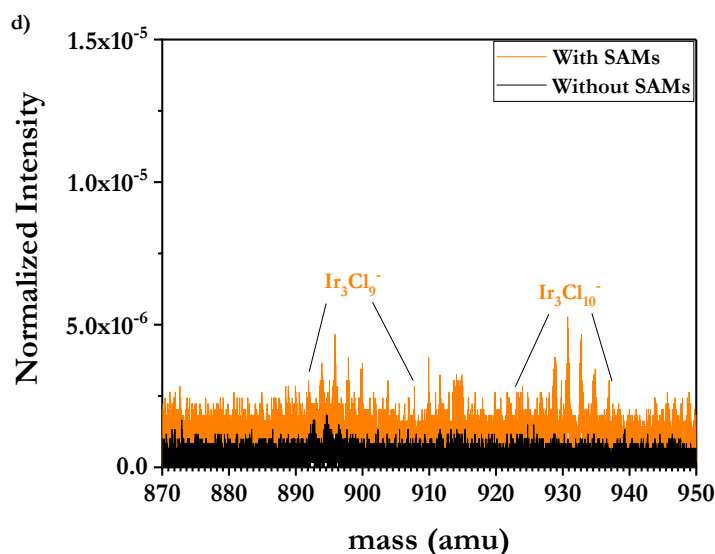
Figure 35. Mass spectra of precleaned Au functionalized with Im-C 11 -SH SAMs and adsorbed Ir(IV) (orange line), and precleaned non-functionalized Au with adsorbed Ir(IV) (black line). [Ir] init = 5.2 \mu M, [HCl] = 0.55 M. (a) Mass range of 280-440 amu showing characteristic peaks of IrCl 3 - and IrCl 4 - clusters. (b) Mass range of 521.5 – 571.5 amu showing characteristic peaks of Ir 2 Cl 4 - and Ir 2 Cl 5 - clusters. (c) Mass range of 588 – 650 amu showing characteristic peaks of Ir 2 Cl 6 - and Ir 2 Cl 7 - clusters. (d) Mass range of 870 – 950 amu showing characteristic peaks of Ir 3 Cl 9 - and Ir 3 Cl 10 - clusters.
