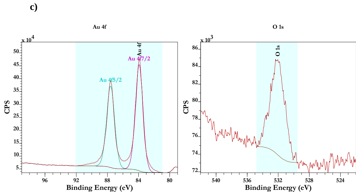
Figure A2. Gold 4f and oxygen 1s XPS for MDDA SAMs on precleaned Au; one SAMs deposition: (a) the freshly prepared SAMs; (b) the freshly prepared sample stored for one week; (c) the freshly prepared sample stored for one month.
