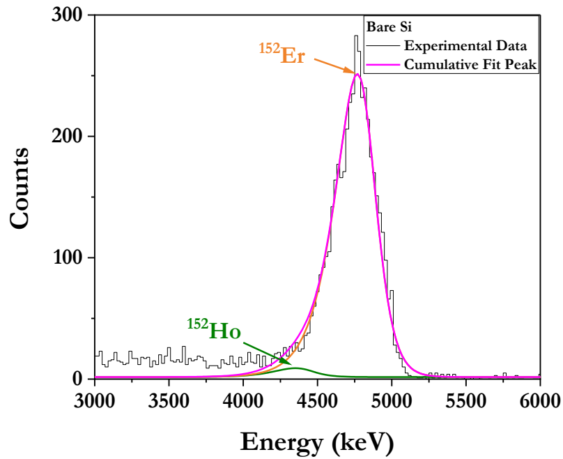
Figure 39. ^{152}\text{Er} calibration spectrum (black histogram) collected on the vertical Bare Si detector with the rotating degrader at 80 degrees. Bin width: 20 keV. The peaks were fitted using Eq. 13.
