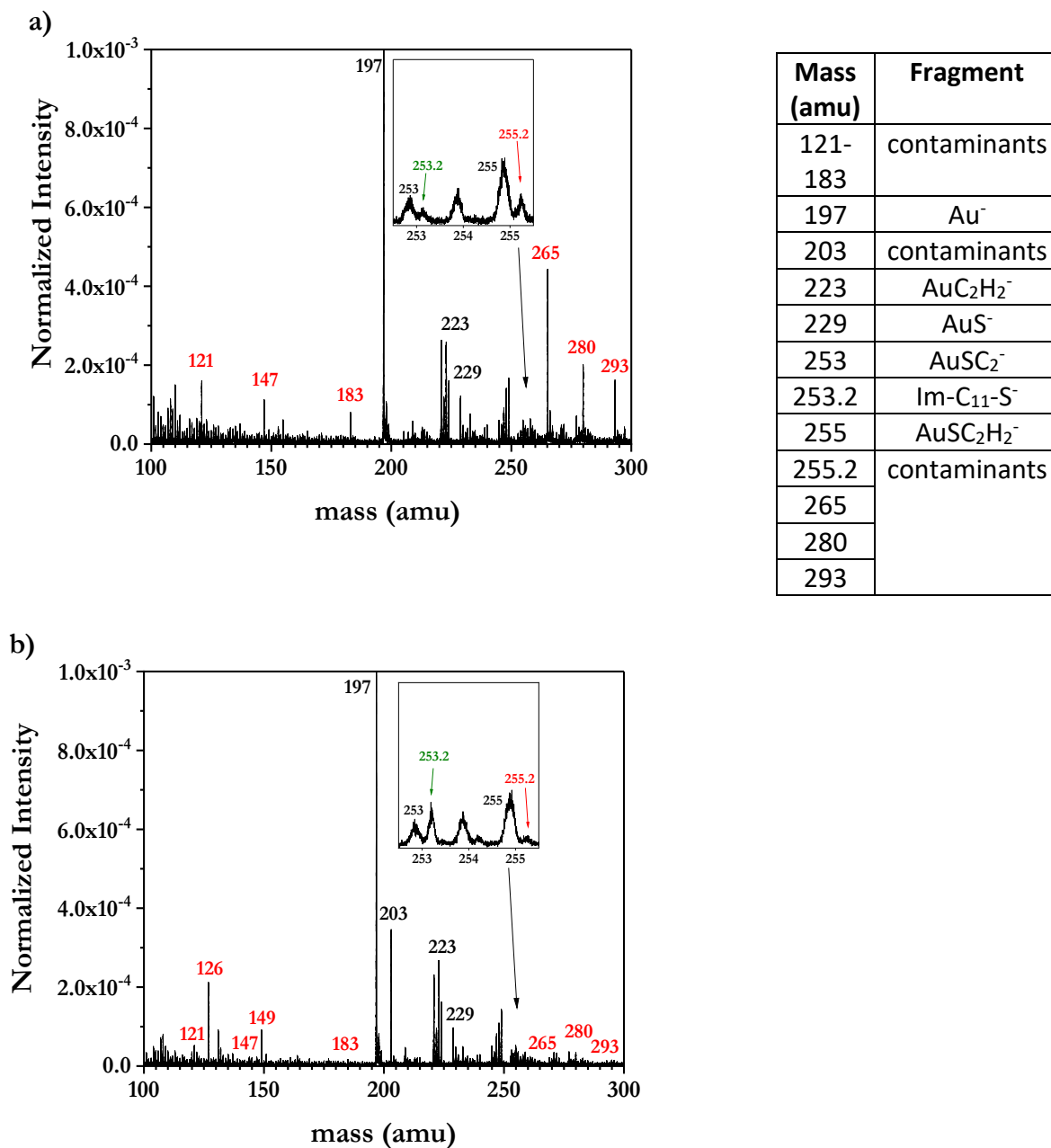
Figure 26. (a) Mass spectrum of non-precleaned Au functionalized with Im-C 11 -SH SAMs deposited from a 1.6 mM ethanolic thiol solution during the first deposition. (b) Mass spectrum of precleaned Au functionalized with Im-C 11 -SH SAMs deposited from a 5 mM ethanolic thiol solution during the second deposition. Mass range of 100-300 amu.
