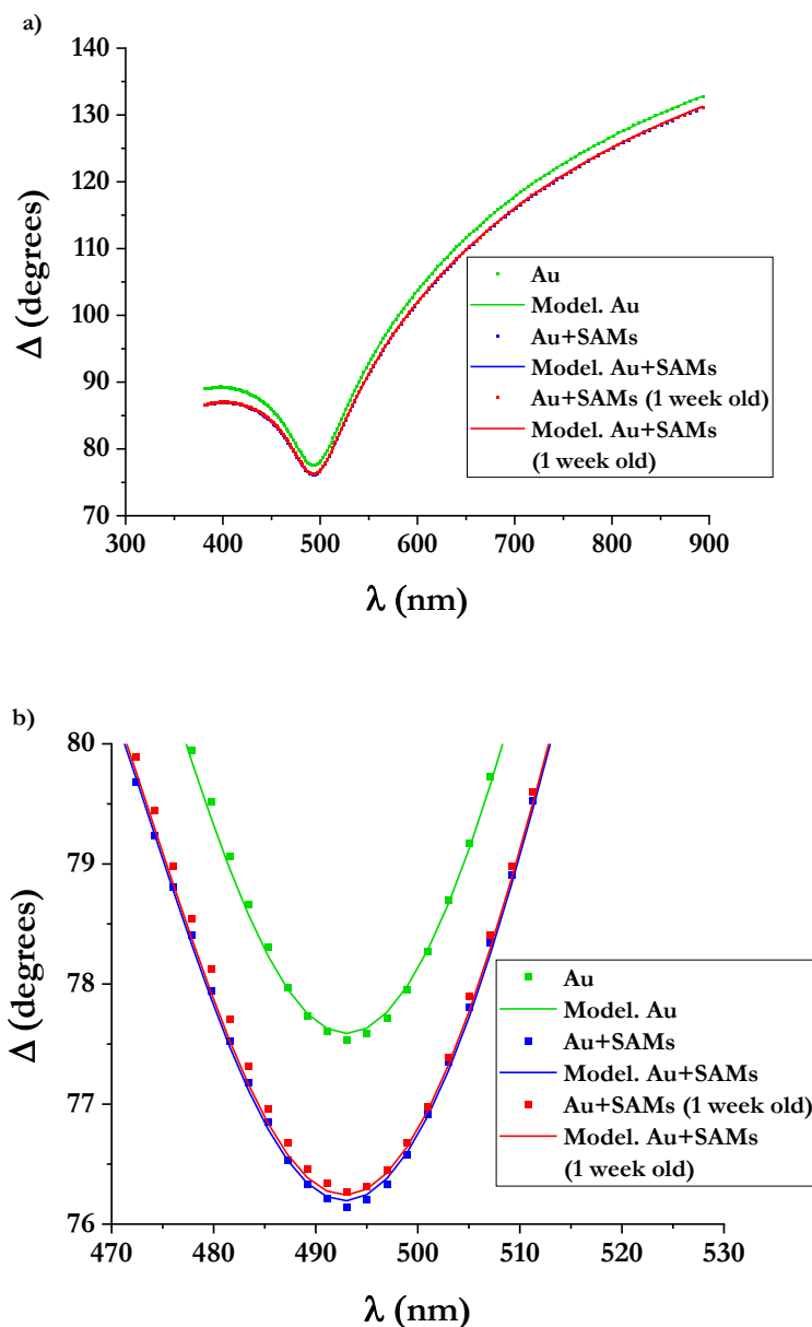
Figure 33. Delta as a function of wavelength: a) full scale; b) zoomed-in region of low delta values. Measured (square symbols) and modeled (solid curves) data for bare precleaned gold (green), freshly deposited Im-C 11 -SH SAMs on precleaned Au (blue), Im-C 11 -SH SAMs on precleaned Au after one week of storage (red). The B-spline layer was used to fit the bare precleaned gold data, n=1.50 . The Cauchy layer was used to fit the Im-C 11 -SH SAMs data, n=1.450 .
