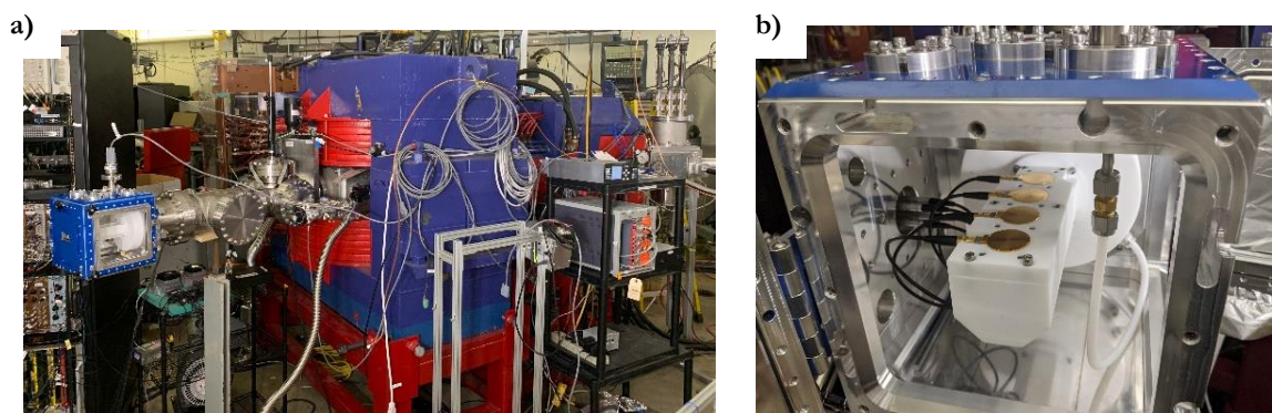
Figure 4 (a) The sRTC installed on the AGGIE separator. (b) The detectors are installed inside the sRTC.
