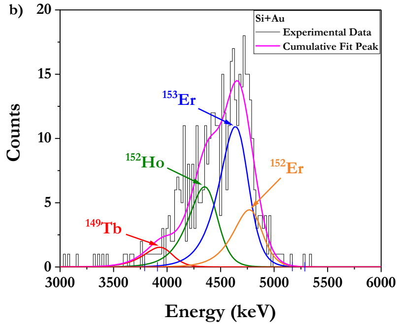
Figure 42. ^{152,153}\text{Er} spectra (black histograms) collected on: (a) the Bare Si detector, (b) the Si+Au detector in configuration A with the rotating degrader at 55 degrees. Bin width: 20 keV. The peaks were fitted using Eq. 13.
