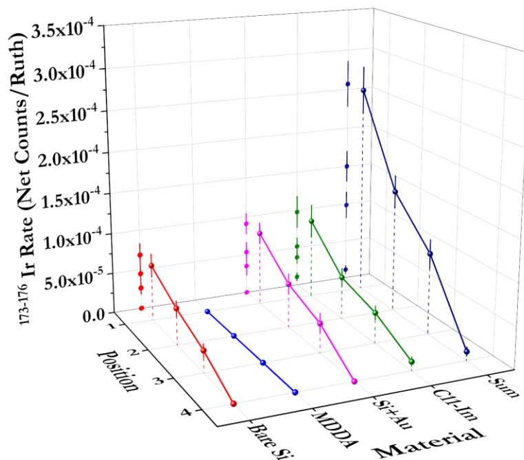
Figure 47. 3D plot of the ^{173-176}\text{Ir} rate as a function of the detector position and material. All rotating degrader angles summed up.
