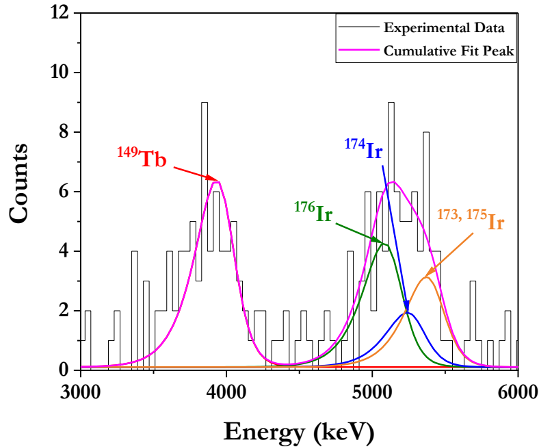
Figure 41. Sum of ^{173-176}\text{Ir} spectra collected on the Bare Si, the Si+Au, the C11-Im detectors in configuration D, and the Bare Si, the Si+Au detectors in configuration A (black histogram). All rotating degrader angles have been summed up. Bin width: 40 keV. The peaks were fitted using Eq. 13.
