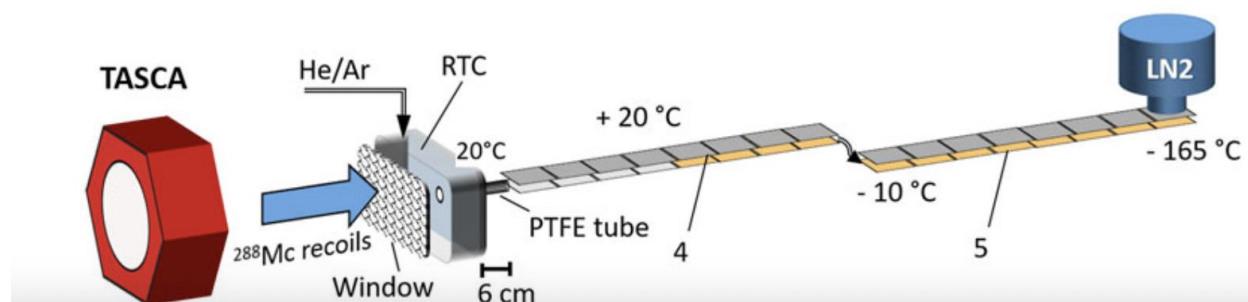
Figure 6. The experimental setup used in thermochromatography experiments performed for Nh chemistry studies at GSI. Reprinted from ref. [4].
