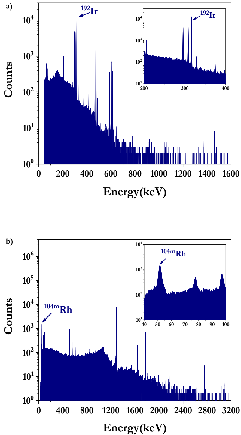
Figure 37. Gamma-ray spectra of (a) ^{192}\text{Ir} and (b) ^{104\text{m}}\text{Rh} as measured with an HPGe detector showing full energy photopeaks at 316.51 keV and 51.42 keV, respectively. The insets of the spectra show the positions of the named photopeaks.
