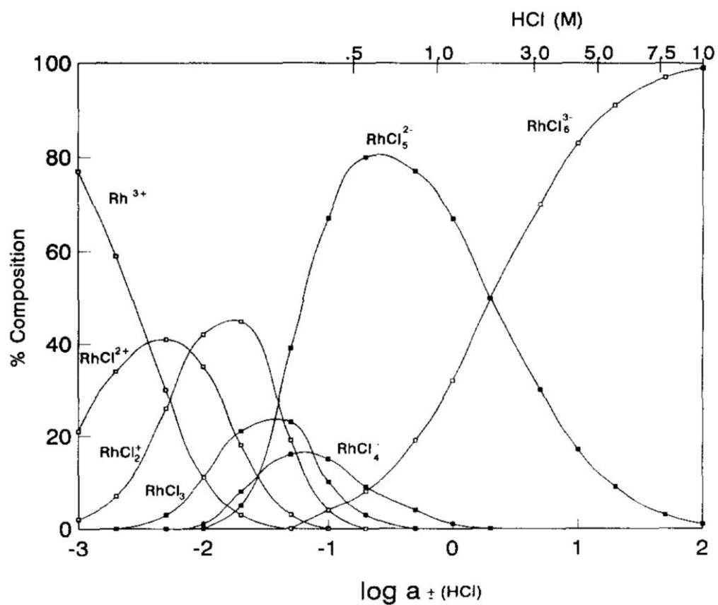
Figure 7. The speciation diagram for Rh(III) in HCl solutions with different concentration. Figure used with permission from ref. [49].
