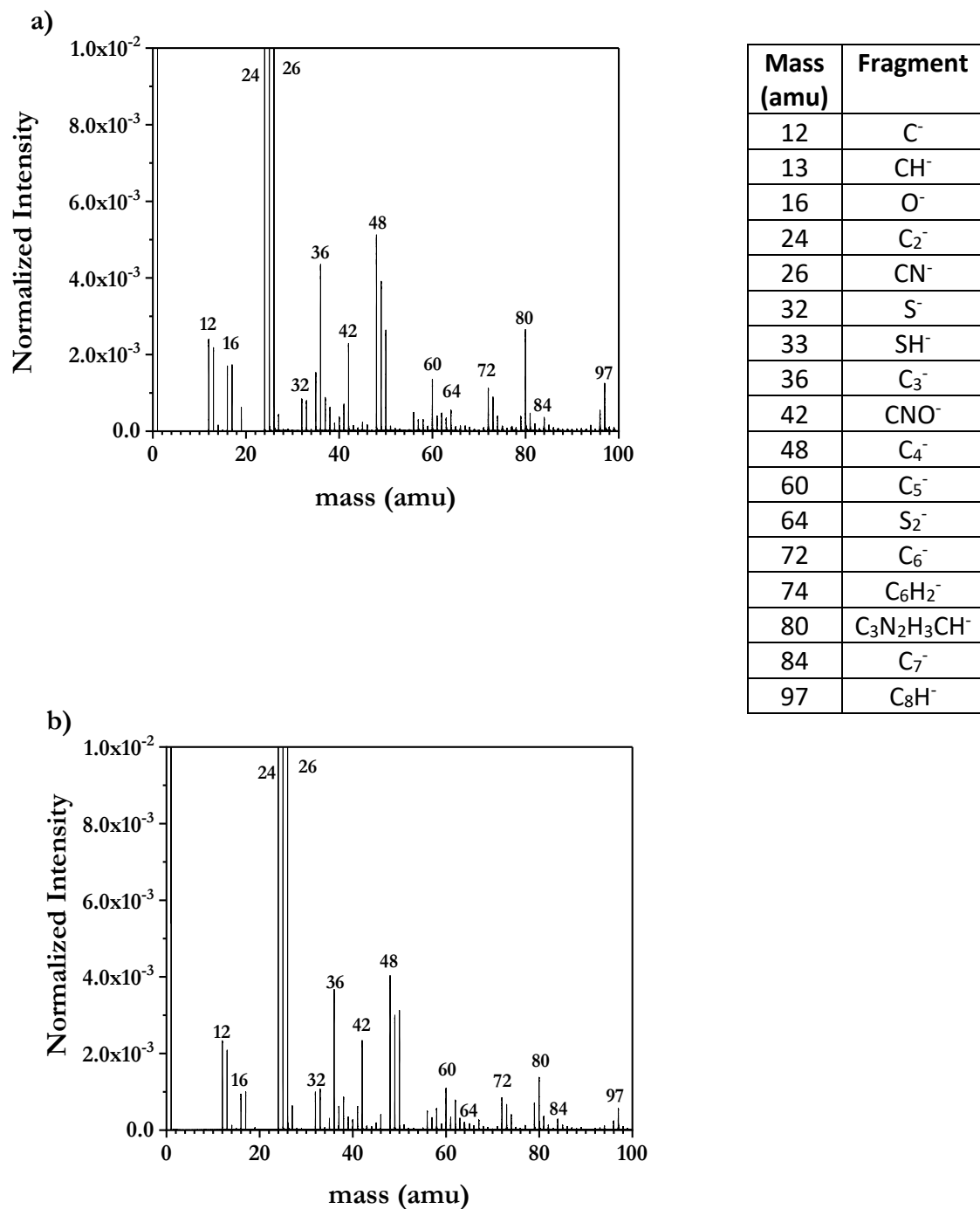
Figure 25. (a) Mass spectrum of non-precleaned Au functionalized with Im-C 11 -SH SAMs deposited from a 1.6 mM ethanolic thiol solution during the first deposition. (b) Mass spectrum of precleaned Au functionalized with Im-C 11 -SH SAMs deposited from a 5 mM ethanolic thiol solution during the second deposition. Mass range of 0-100 amu.
