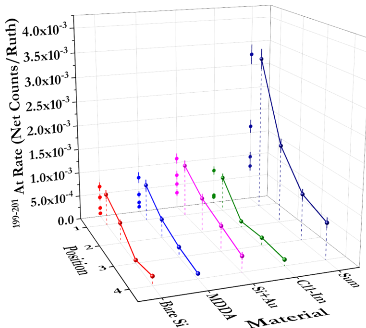
Figure 45. 3D plot of the ^{199-201}\text{At} rate as a function of the detector position and material. The rotating degrader was set to 45 degrees.
