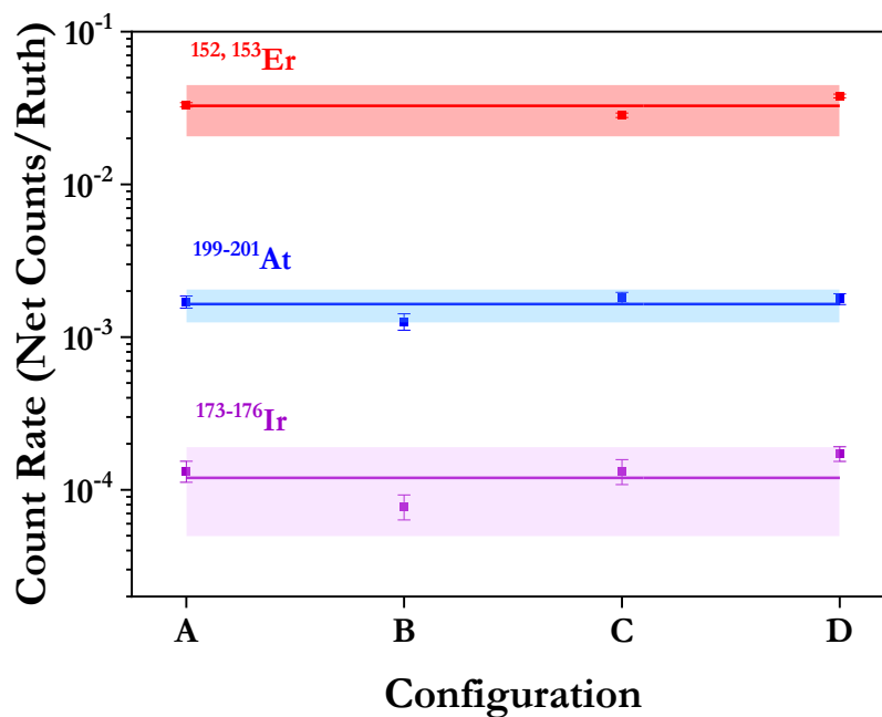
Figure 49. The count rate of ^{152,153}\text{Er} (red squares), ^{199-201}\text{At} (blue squares), and ^{173-176}\text{Ir} (purple squares) as a function of the detector configuration. The data were fitted using the linear function with the slope set to zero. Shades represent 95% confidence bands. ^{152,153}\text{Er} rate at configuration B is an outlier and was not included in calculations.
