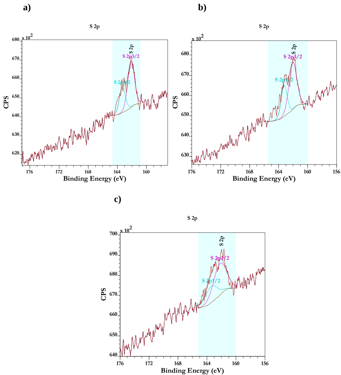
Figure 31. Sulfur 2p XPS for MDDA SAMs on precleaned Au; one SAMs deposition: (a) the freshly prepared SAMs; (b) the freshly prepared sample stored for one week; (c) the freshly prepared sample stored for one month.
