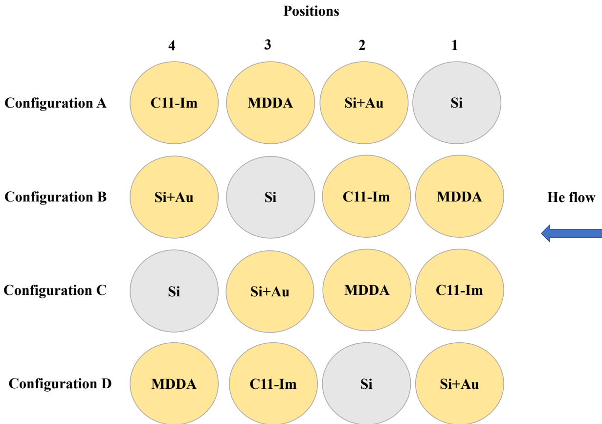
Figure 38. A schematic diagram of four configurations tested during the experiment. The blue arrow shows the entrance of the sRTC.
