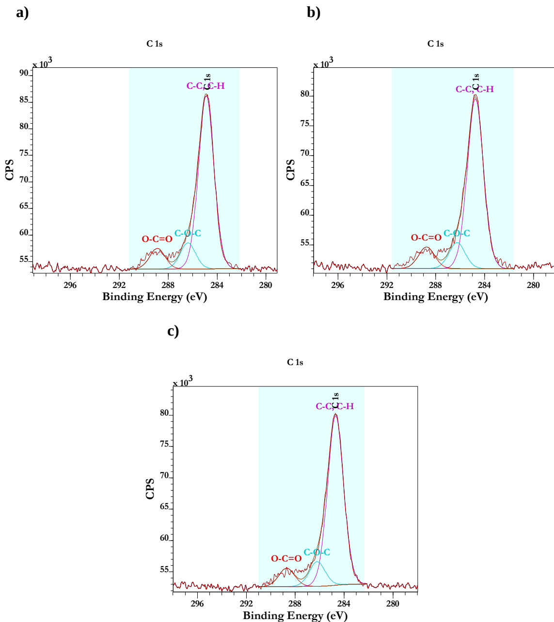
Figure 32. Carbon 1s XPS for MDDA SAMs on precleaned Au; one SAMs deposition: (a) the freshly prepared SAMs; (b) the freshly prepared sample stored for one week; (c) the freshly prepared sample stored for one month.
