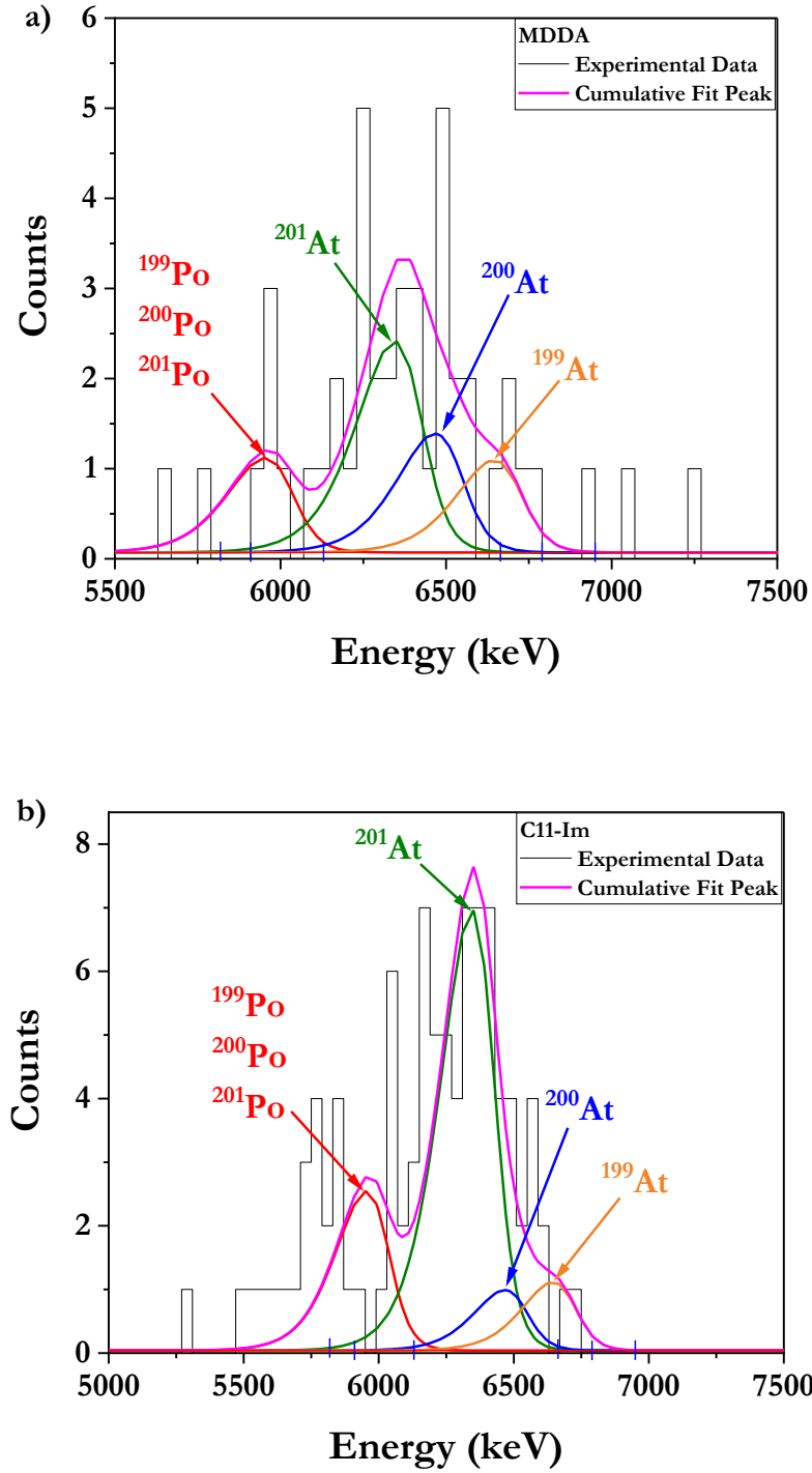
Figure 44. ^{199-201}\text{At} spectra (black histograms) collected on: (a) the MDDA detector, (b) the C11-Im detector in configuration C with the rotating degrader at 45 degrees. Bin width: 40 keV. The peaks were fitted using Eq. 13.
