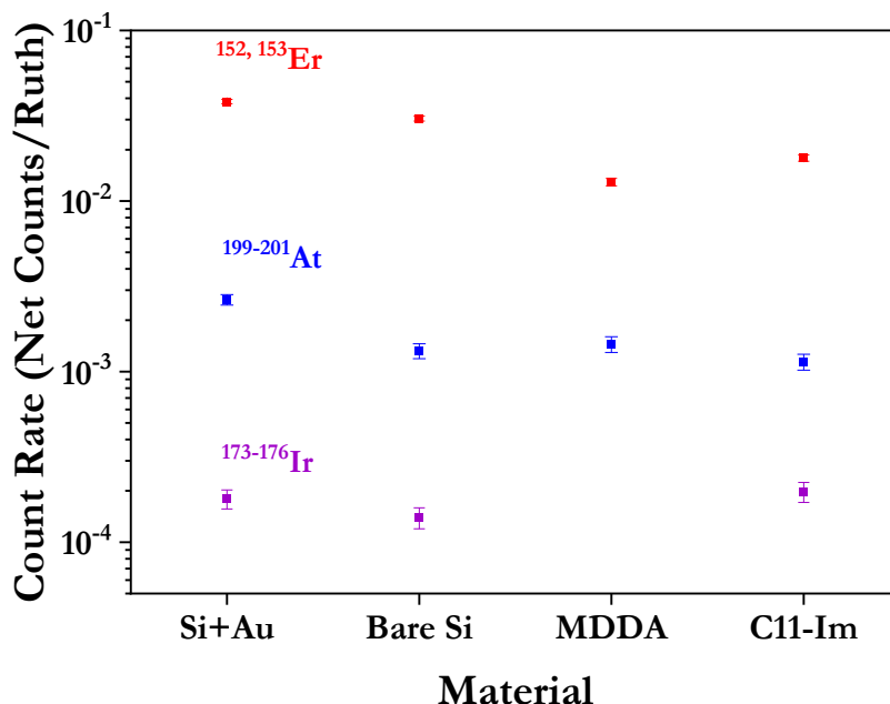
Figure 50. The count rate of ^{152, 153}\text{Er} (red squares), ^{199-201}\text{At} (blue squares), and ^{173-176}\text{Ir} (purple squares) as a function of the detector material. Due to low statistics, ^{173-176}\text{Ir} count rate on the MDDA detector could not be determined.
