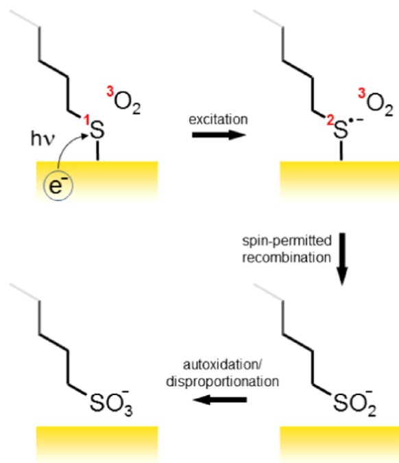
Figure 21. The SAMs photooxidation mechanism. Reprinted with permission from R. Yan, A. Terfort, and M. Zharnikov, J. Phys. Chem. C 125 , 1855 (2021). Copyright 2022 American Chemical Society.
