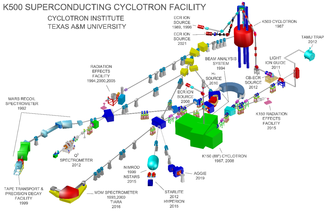
Figure 11. A scheme of the normal conducting K150 cyclotron used in this study, and the superconducting K500 cyclotron.
