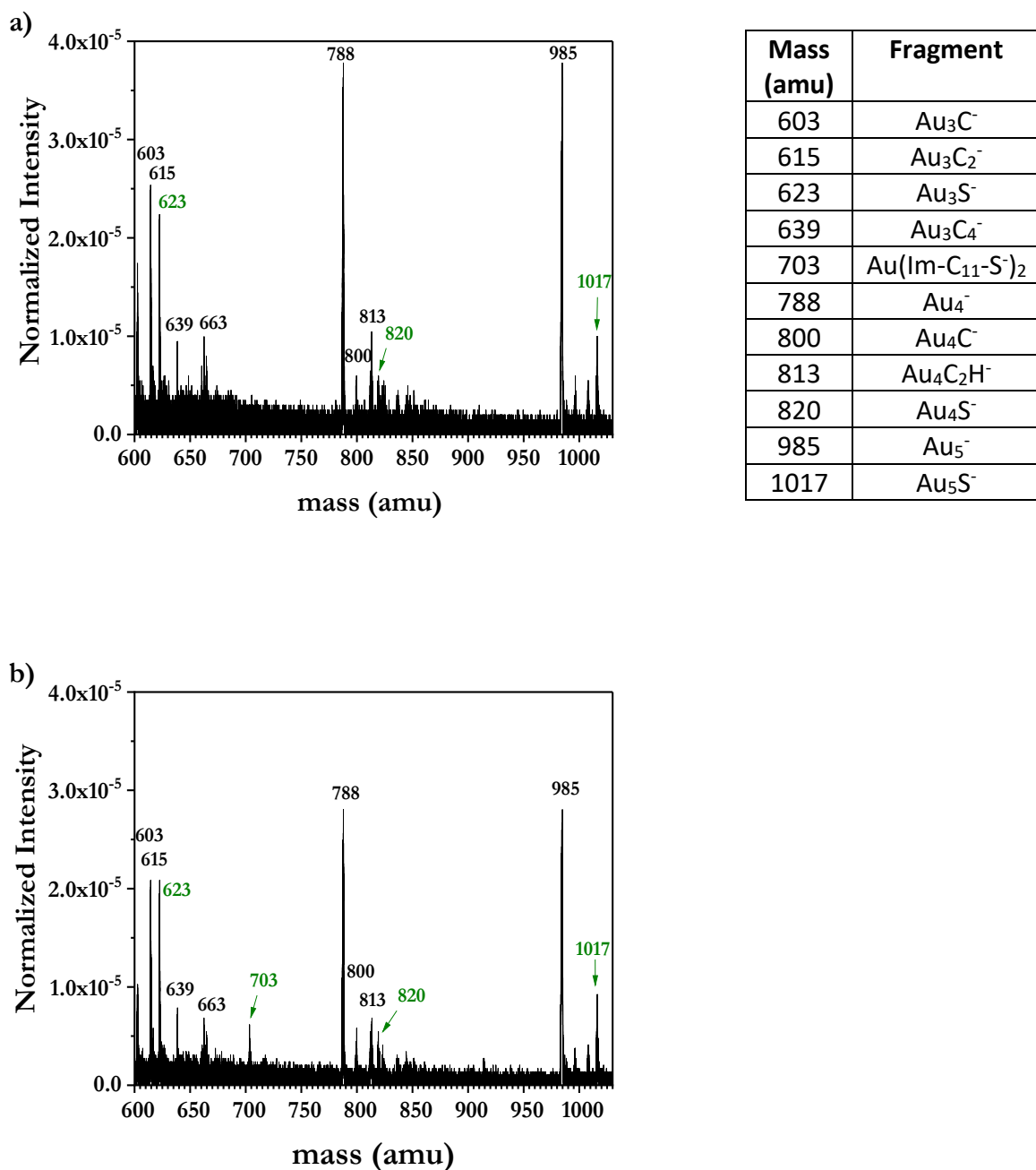
Figure 28. (a) Mass spectrum of non-precleaned Au functionalized with Im-C 11 -SH SAMs deposited from a 1.6 mM ethanolic thiol solution during the first deposition. (b) Mass spectrum of pre-cleaned Au functionalized with Im-C 11 -SH SAMs deposited from a 5 mM ethanolic thiol solution during the second deposition. Mass range of 600-1030 amu.
