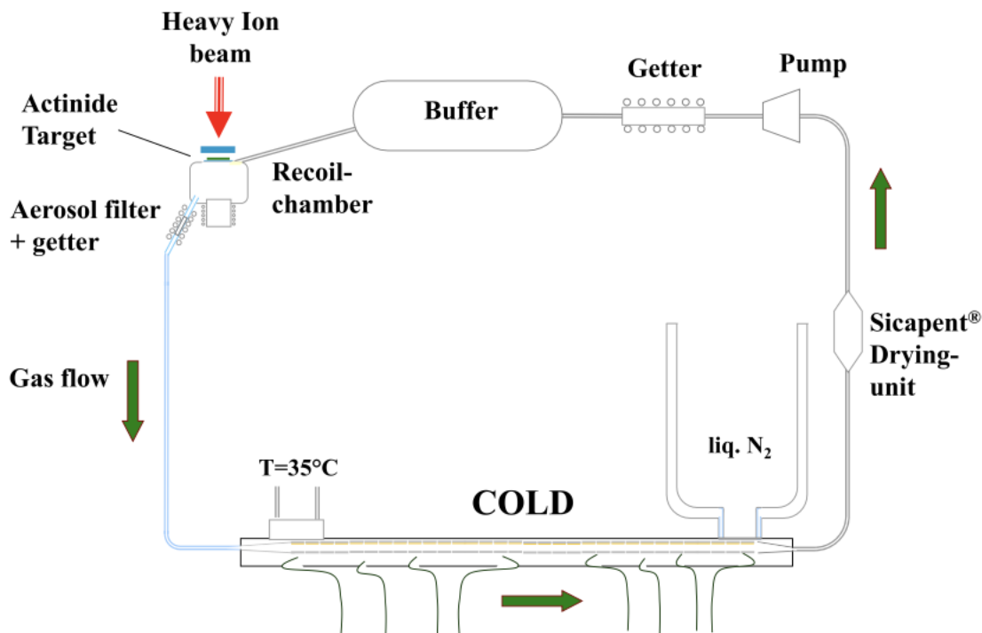
Figure 5. The experimental setup used in thermochromatography experiments performed for Cn chemistry studies at FLNR. Illustration used with permission from ref. [37].
