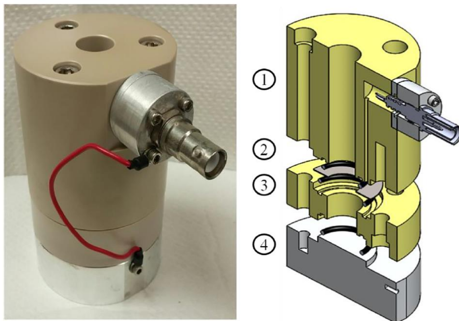
Figure 15. Electrodeposition cell used in this study to make the ^{141}\text{Pr}_2\text{O}_3 400 \mu\text{g}/\text{cm}^2 target. (1) The main body made of polyetheretherketone (PEEK); (2) platinum anode; (3) PEEK centerpiece; (4) aluminum cathode. Figure used with permission from ref. [117].
