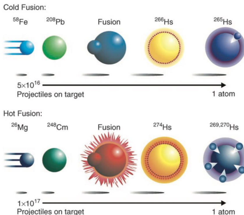
Figure 2. Schematics of cold- and hot-fusion reaction mechanisms with examples of the ^{208}\text{Pb}(^{58}\text{Fe}, n)^{265}\text{Hs} and the ^{248}\text{Cm}(^{26}\text{Mg}, 4-5n)^{269-270}\text{Hs} reactions, respectively. Figure used with permission from ref. [8].
