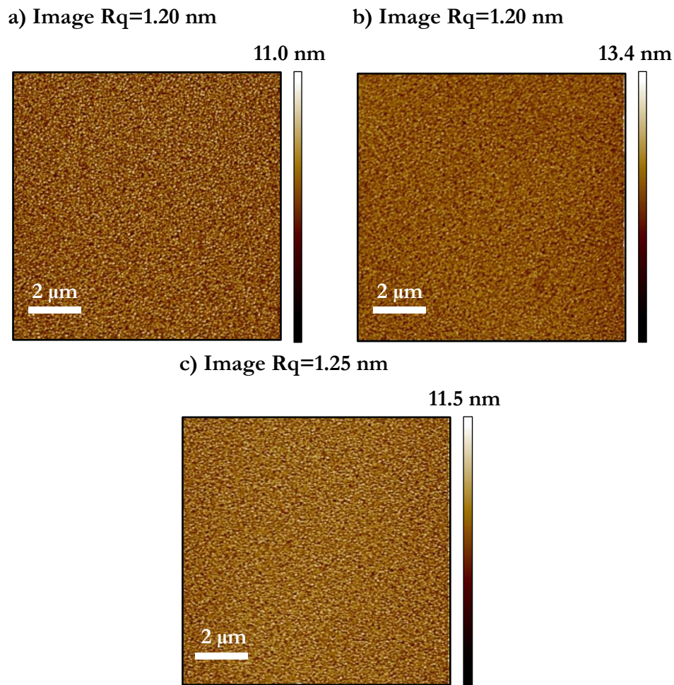
Figure 23. AFM images ( 10 \times 10 \mu\text{m} ) of (a) pure precleaned Au, (b) Im-C 11 -SH SAMs on precleaned Au (the first deposition), (c) Im-C 11 -SH SAMs on precleaned Au (the second deposition).
