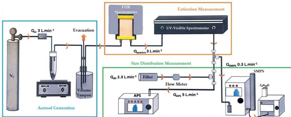
Figure 56 Experimental apparatus parts: aerosol generation, extinction measurement, and size distribution measurement (Reproduced from Deschutter, 2022 ).
