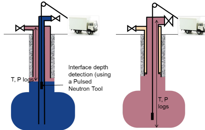
Figure 14. Cavern and main monitoring equipment required during an in situ mass balance. Wireline runs are needed to measure a temperature log along the test fluid, and deduce the density of the test fluid. On the left, only the top portion of the well is filled with the test fluid (gas – usually nitrogen – or liquid hydrocarbon) down to an interface, whose depth also has to be measured during the run. On the right, in the gas cavern MIT, the test fluid is the stored gas.
