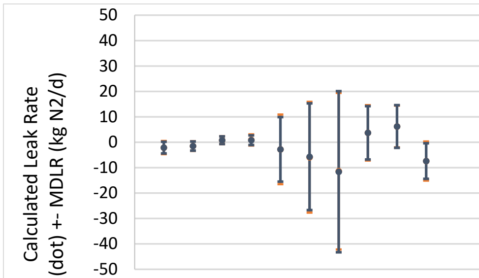
Figure 32. Calculated Leak Rate (dot) +/- the MDLR (line) for 10 Nitrogen-Brine MITs interpreted by Geostock using the in-situ mass balance method. Two uncertainty propagation methods are used: 1 st order (orange) and Monte Carlo (blue). From Réveillère (2019).
