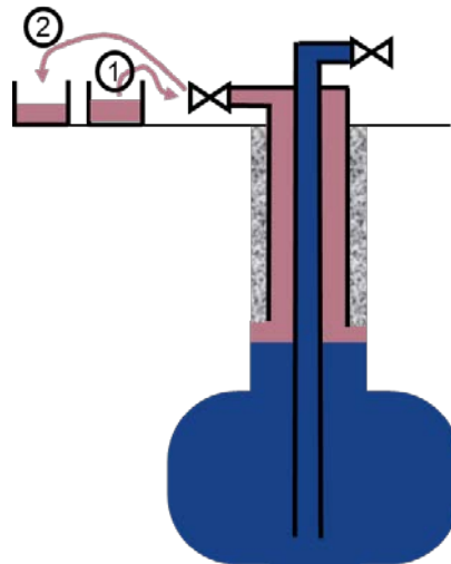
Figure 20. Cavern and main monitoring equipment during a Liquid-Liquide Interface MIT interpreted by an above-ground balance method.
