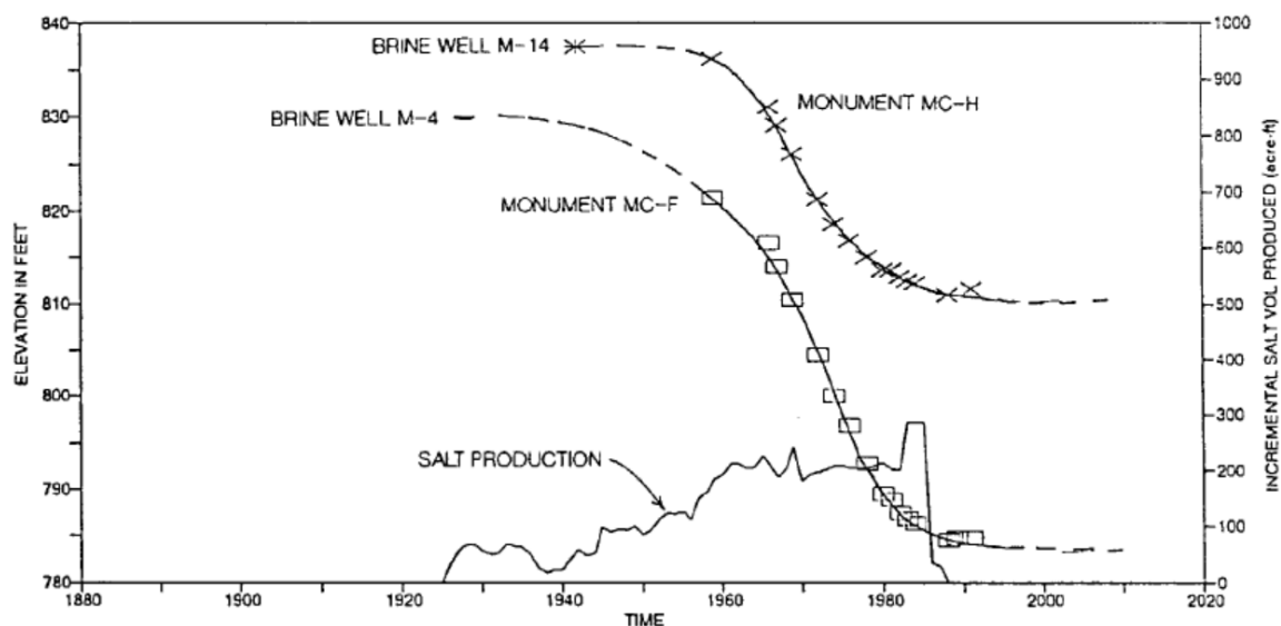
Figure 7: Subsidence salt production on the Tully Valley brinefield. Details can be found in Walker et al., 1993, from which this figure is taken.
