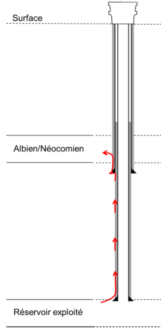
Figure 24: Microannulus leakage scenario considered in Vernoux and Manceau (2017)
