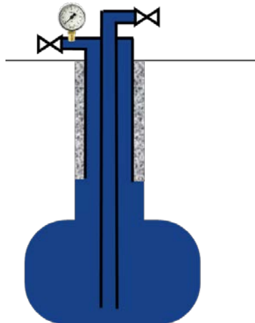
Figure 12. Cavern and main monitoring required during an hydraulic test interpretation
