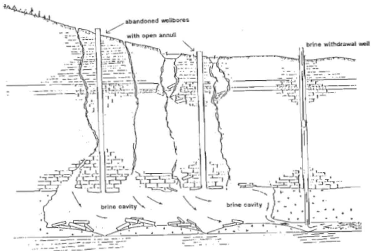
Figure 8 : schematic illustration of the Wild brining mining method applied at Tully valley. Brine cavity is recharged by groundwater through a flow in intentionally open wellbores (after the casings have been pulled out), as well as fracture associated with subsidence. Brine is probably produced using air lift. From Stanford (1996).
