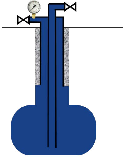
Figure 29. Cavern and monitoring used during a hydraulic test and during a Pressure Observation Test (POT)
