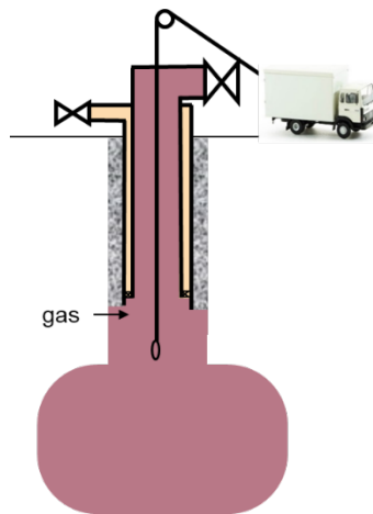
Figure 30. Cavern and monitoring used during an in-situ mass balance interpretation of a gas cavern MIT
