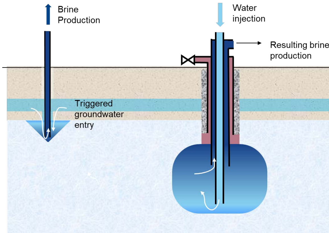
Figure 4: Left: early leaching through « Wild brining », leaching process is controlled by brine pumping out. It triggers a groundwater flow into the cavern. Right: modern solution mining, with a cemented well down to the salt formation, a blanket fluid preventing the leaching to rise above it. The leaching process is controlled by water injection. Here direct leaching is depicted; water being injected through the inner string at the bottom of the cavern. Reverse leaching with water injection in the annulus is possible too.
