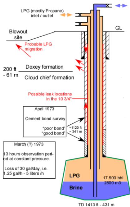
Figure 11 : Elk city blow out. Schematic of the leakage scenario (in red) and summary of the post-incident investigations (left, from Réveillère et al., 2018) and of the results of the LPG blow out – without ignitio - at the surface (right, from Fay, 1973)
