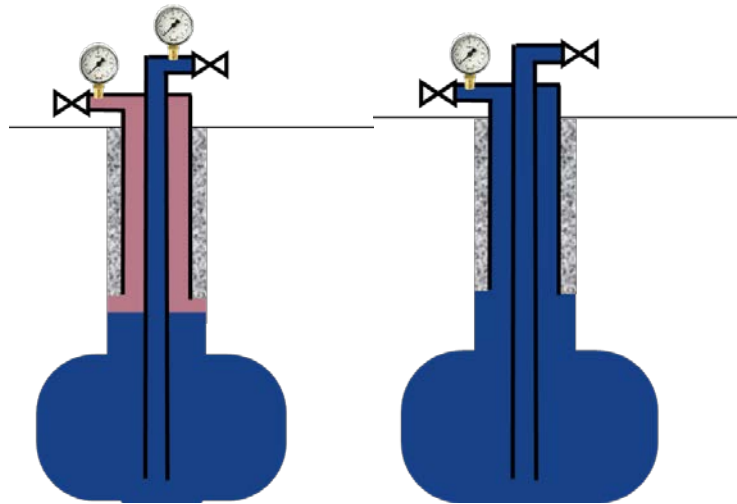
Figure 15. Cavern and main monitoring equipment during a POT. In the most referenced cases, POT is done with an oil-brine interface lowered down to below the casing shoe. But it could also be done with a cavern fully filled with brine, or with nitrogen instead of oil.
