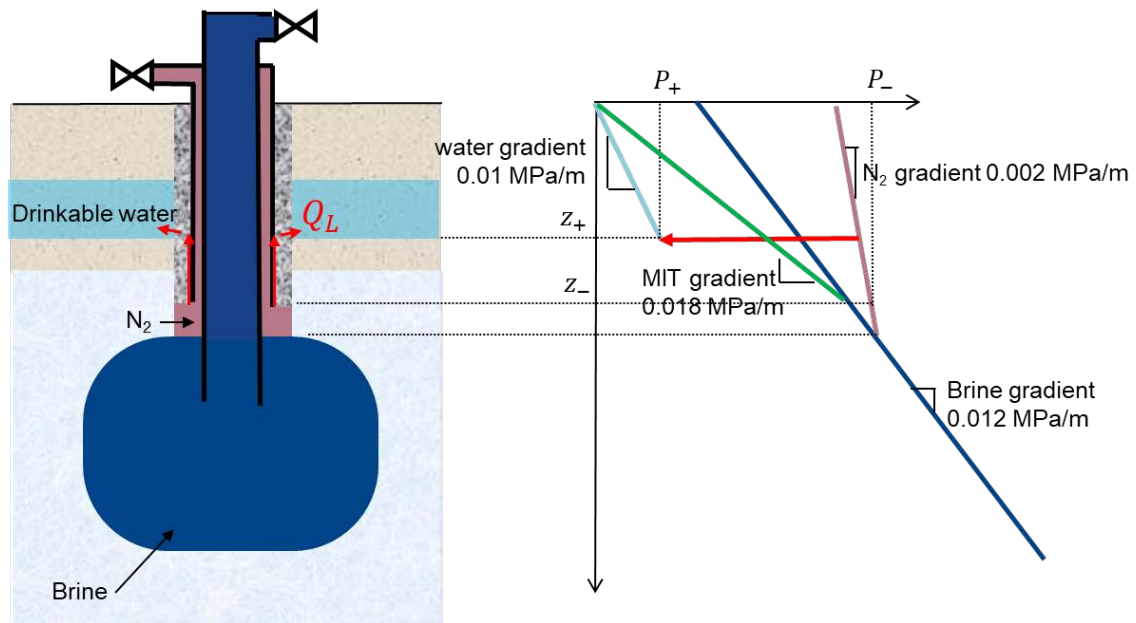
Figure 25: pressure profiles in the cavern and surrounding groundwater, and MIT test pressure gradient (in green). The microannulus leakpath is represented in red in the left diagram, and the driving force of it by the red arrow in the right figure.
