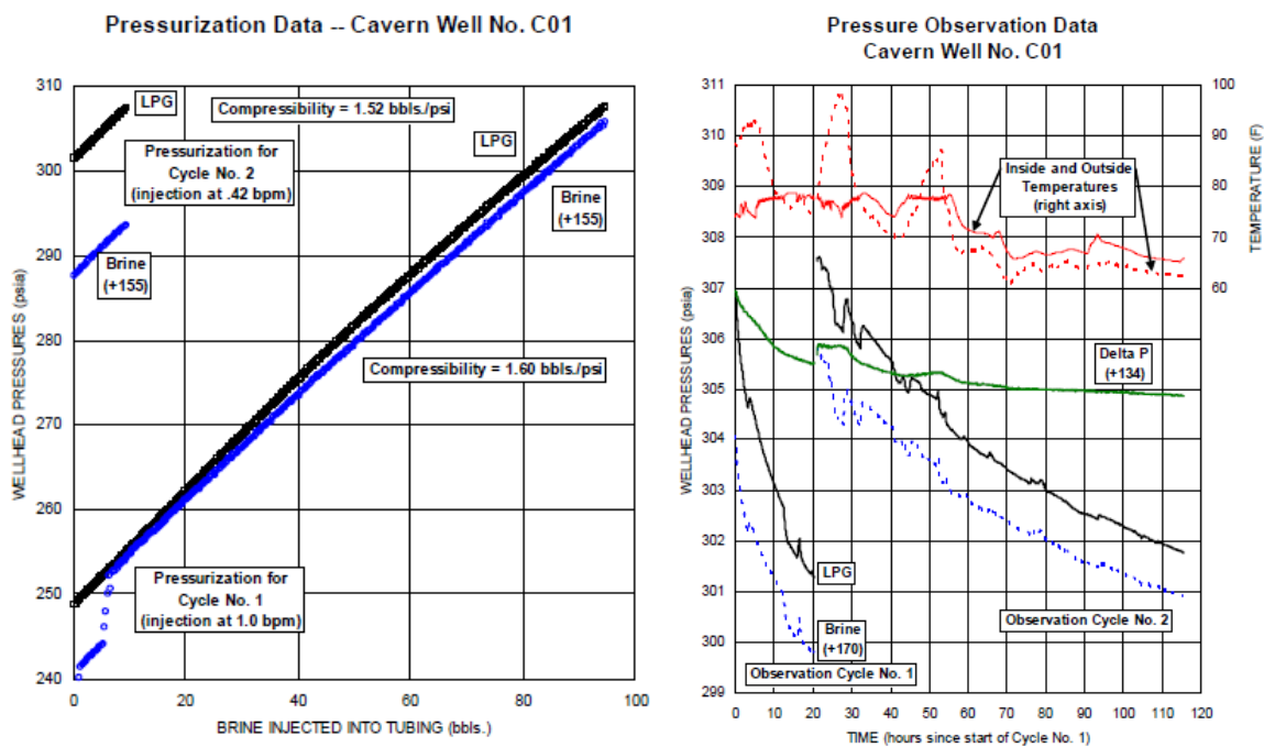
Figure 15. Left: the cavern compressibility is measured during the pressurisation 10 Right: Pressure decay during the test 11 . From Thiel and Russel, 2004.
