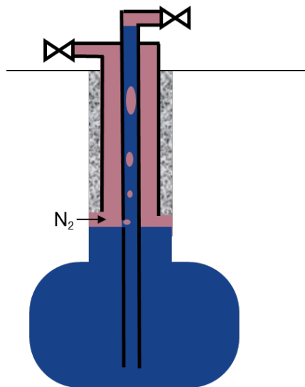
Figure 20. Cavern and main monitoring equipment during a nitrogen-brine MIT interpreted by an in-situ compensation method.
