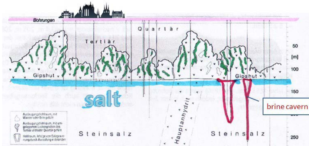
Figure 2: Section of a salt dome with 2 caverns without salt roof (in red contour) due to uncontrolled wild brining. From Crostogino and Wilke (2014)
