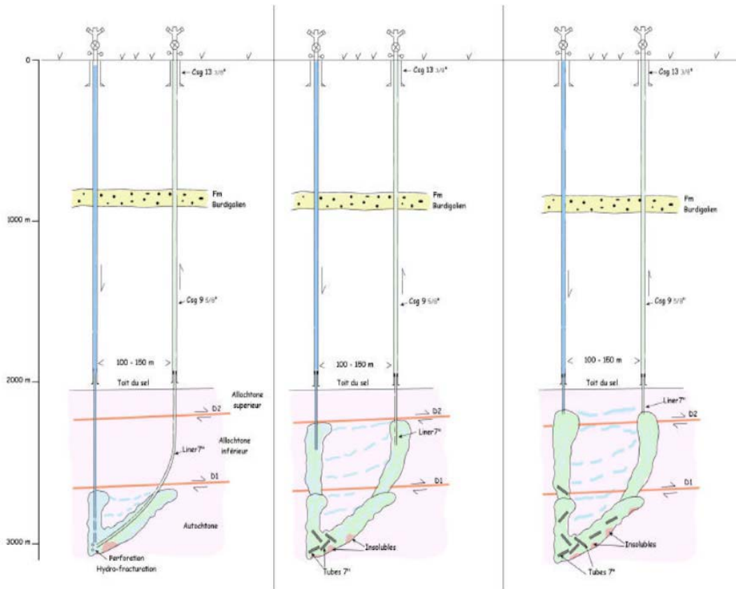
Figure 10: Schematic cross section of subsequent phases of salt leaching in Vauvert, France, by means of a doublet. Water injected in the well on the left circulated through cracks in the salt, dissolving it, and is produced by the well on the right. From Duquesnoy et al., 2013.
