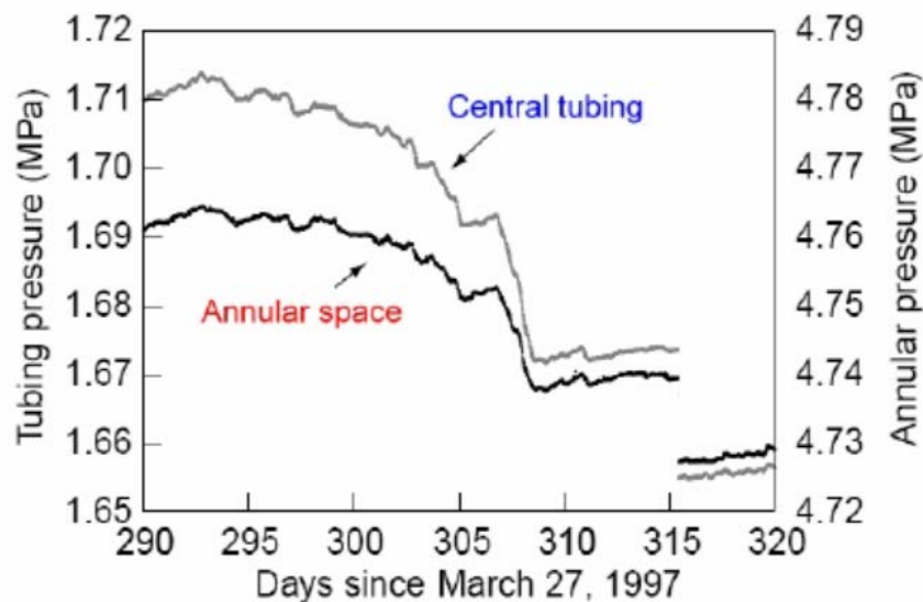
Figure 17. Annular Space and Tubing Pressure During a Well Leak. The two curves are parallel before Day 293 (no leak) and after Day 315 (leak repaired). Not in between, due to a surface leak at the wellhead. From Van Sambeek et al. (2005)
