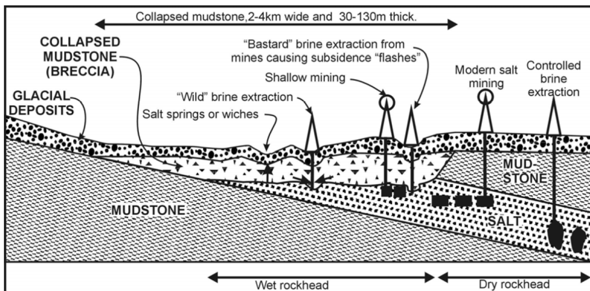
Figure 6: Cross-section through a typical Cheshire Triassic salt area showing past and present brine production techniques. From Cooper (2002)
