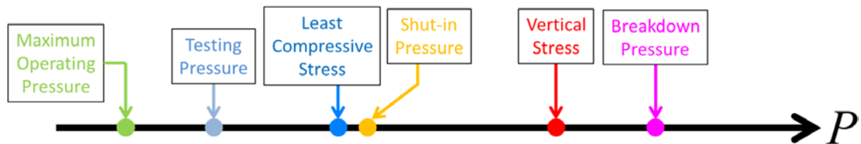
Figure 21: The testing pressure is selected above (or equal to) the Maximum Operating Pressure, and significantly smaller than the least compressive stress. From Bérest et al., 2020.
