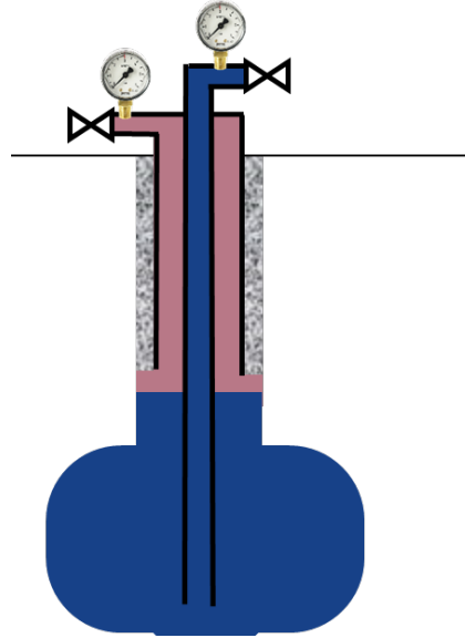
Figure 34. Cavern and monitoring used during a Pressure Difference Observation Test (PDO)
