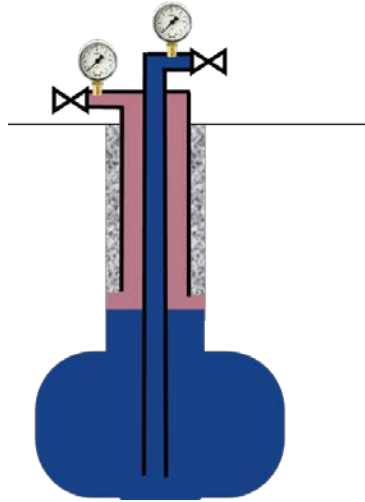
Figure 19. Cavern and main monitoring equipment during a PDO.
