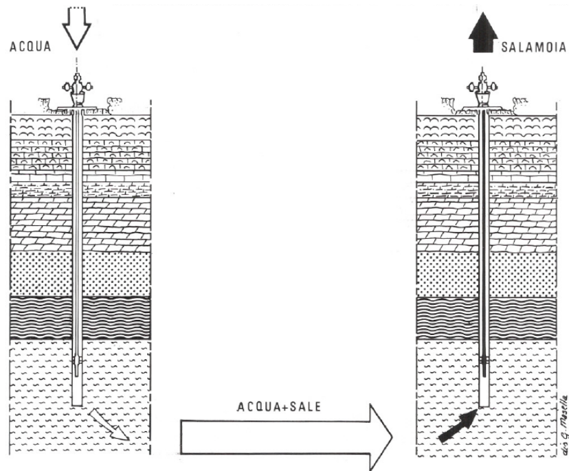
Figure 9. Schematic of the multiple wells brining method used from 1970 to 1986 at Belvedere di Spinello. From Gisotti, 1992.
