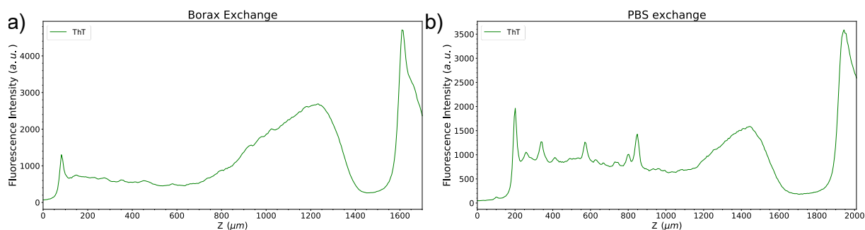
Figure S7: Diffusion of a Fmoc-FFpY solution ( 1 \text{ mg.mL}^{-1} , 25 \text{ mM} Borax buffer, \text{pH } 9.5 ) through an AP-HPMC hydrogel and monitoring by CLSM the fluorescence emission of ThT over time and depth within the host material ( \lambda_{ex} = 450 \text{ nm} ; \lambda_{em} = 482 \text{ nm} ). The AP-HPMC host hydrogel was first brought in contact with a large amount of (a) Borax buffer ( \text{pH } 9.5 ) or (b) Phosphate buffer (PBS, \text{pH}=7.6 ), before the diffusion of the Fmoc-FFpY solution.
