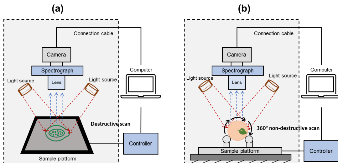
Fig. 16. The destructive (a) and non-destructive (b) HSI scanning methods to detect the heterogeneity of F&V.
