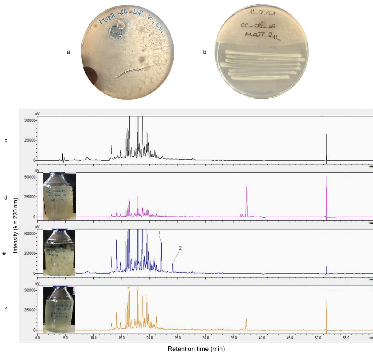
Figure 6. Antibiosis and chromatograms of mono-cultures and co-culture extracts. (a) bacterial/fungal antibiosis on isolation plate; (b) solid co-culture of bacterium and fungus isolated; HPLC chromatogram of (c) liquid culture medium EtOAc crude extract (d) Pseudomonas gessardii liquid culture EtOAc crude extract (e) Neurospora retispora liquid culture EtOAc crude extract (f) P. gessardii and N. retispora liquid co-culture EtOAc crude extract. Peaks corresponding to compounds 1-2 are missing in co-culture.
