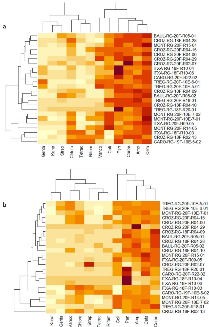
Figure 4. Heatmaps on the antibiotic resistance coefficient. Heatmaps were performed on the lsmeans obtained by running a liner-mixed model on the antibiotic resistance coefficient and by controlling for the block and replication effect. (a) heatmap on the antibiotic coefficients obtained when strains were inoculated at the stationary phase; (b) heatmap on the antibiotic coefficients obtained when strains were inoculated at the exponential phase. Name of the tested strains are reported in the y-axis antibiotics are reported in the x-axis. Abbreviations: Genta = gentamicin, Kana = kanamycin, Vanco = vancomycin, Chlora = chloramphenicol, Tetrac = tetracycline, Rifam = rifampicin, Strep = streptomycin, Coli = colistin, Pen = penicillin G, Carbe = carbenicillin, Amp = ampicillin, Cefa = cefalexin.
