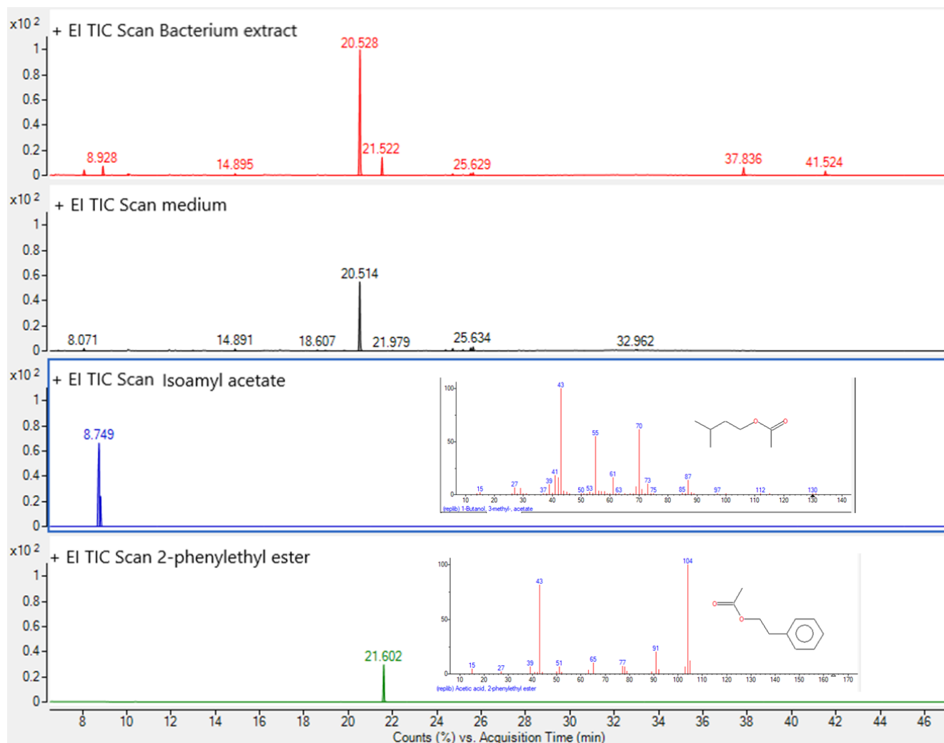
Figure 1 GC-MS total ion chromatograms (TIC) using electron impact (EI) ionization of (A) SPME extraction of P. etheri fermentation broth's head space; B) SPME extraction of GYM Streptomyces medium's head space; (C) isoamyl acetate standard; (D) 2-phenylethyl ester standard. Peaks: (1) isoamyl acetate, (2) 2-phenylethyl ester, (3) and (4) unidentified sesquiterpenes. Peaks 1 and 2 were identified after comparison of their mass spectrum with those of NIST 17 and after injection of the analytical standards.
