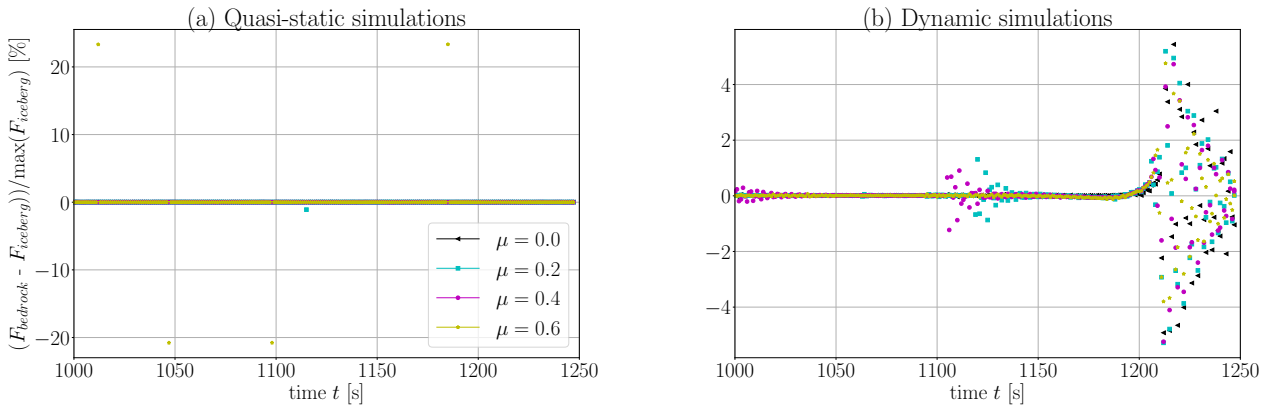
Figure 4.17: Relative difference between the external force applied on the terminus and the force transmitted in the bedrock (F_{iceberg} - F_{bedrock})/\max(F_{iceberg}) for a top-out capsized, a grounded glacier, a Weertman coefficient of 5 \cdot 10^9 Pa s/m, and for a Coulomb friction coefficient of \mu = [0, 0.2, 0.4, 0.6] .
