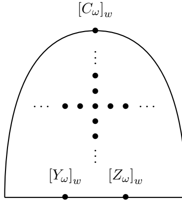
Figure 3.7: The Wadge order on D_w(\Sigma_1^0)(\mathcal{P}\omega) .
