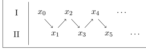
Figure 2.1: A run of the Gale-Stewart game G_{[T]}(A) .
