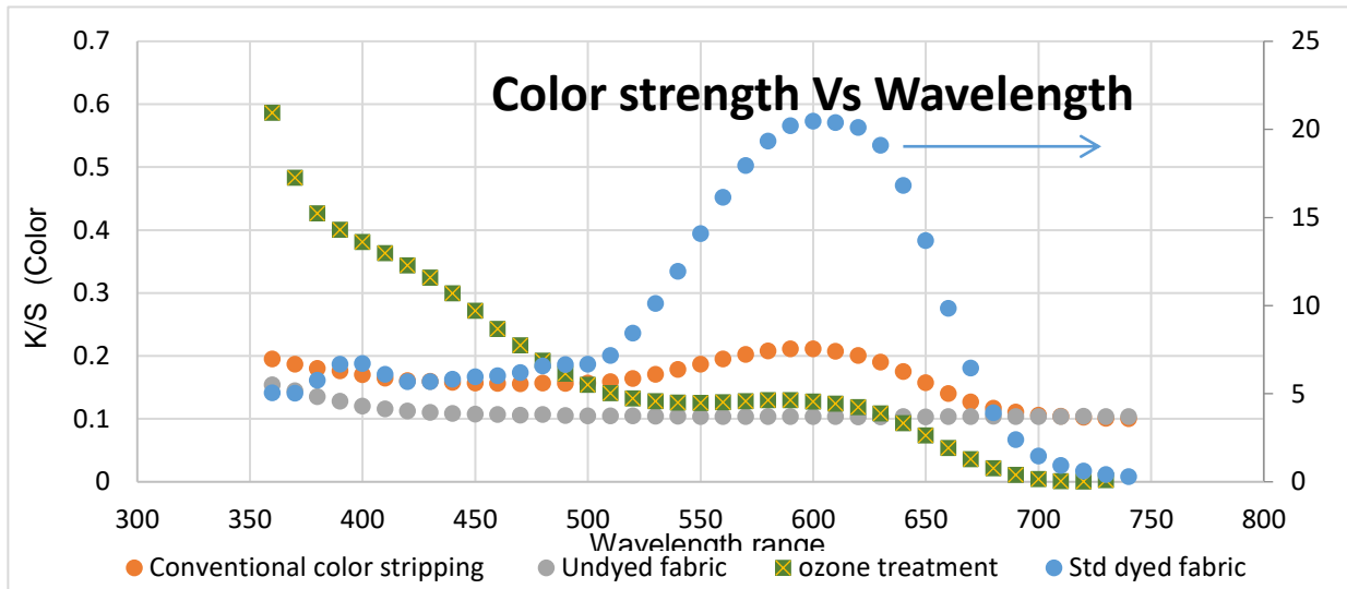
Figure 4. 2 K/S spectral curves of stripped fabric (ozone treated, conventional method) compared to that of the dyed cotton fabric.
