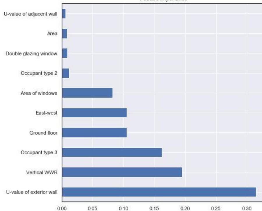
Figure 5-5 : Feature importance analysis results on ground and middle floor of KM7_5 assuming input parameters do not interact each other
