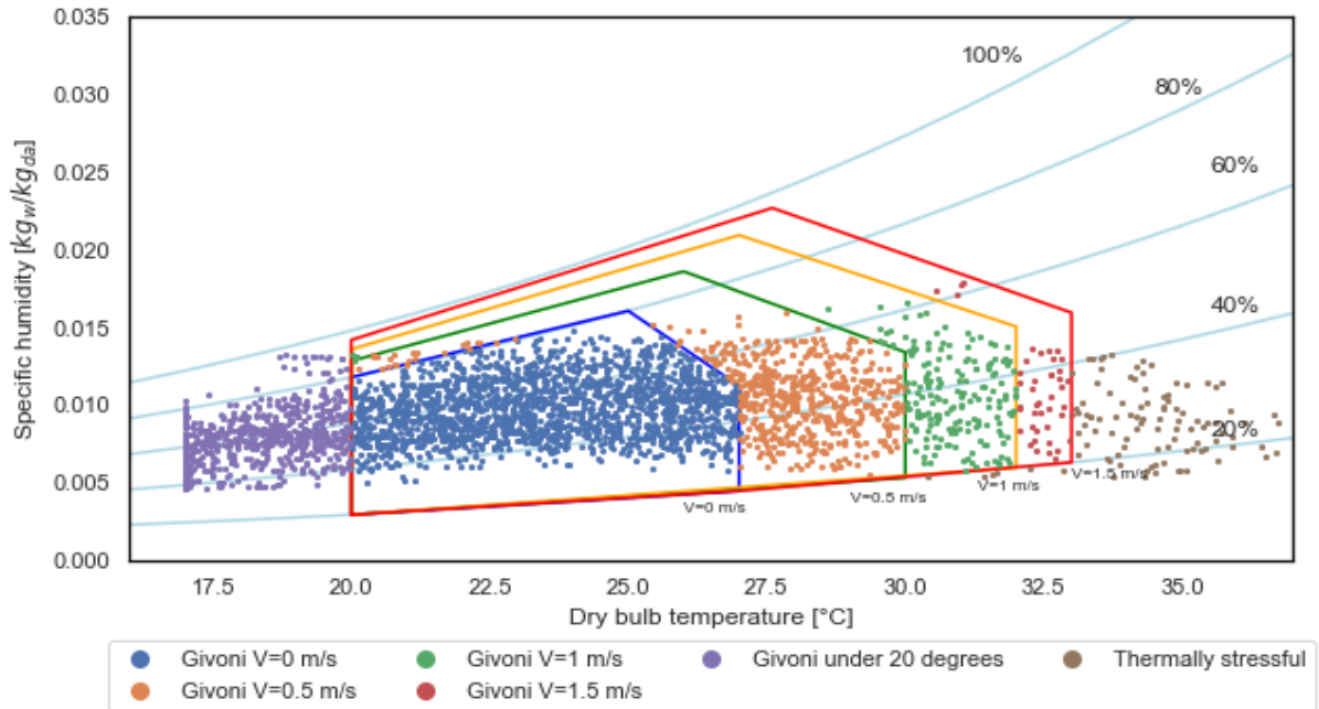
Figure 4-9 : Psychometric chart and Givoni bioclimatic design polygons
