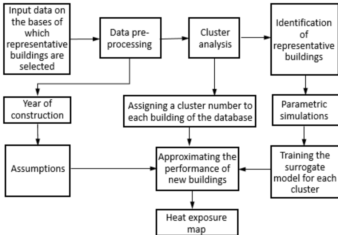
Figure 5-18 : Implementation of surrogate model process
