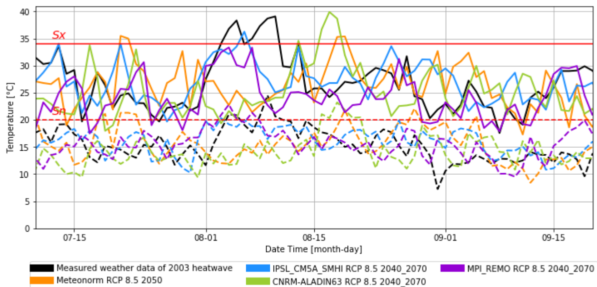
Figure 3-11: Maximum and minimum daily temperatures of weather files plotted alongside heatwave meteorological indicator thresholds
