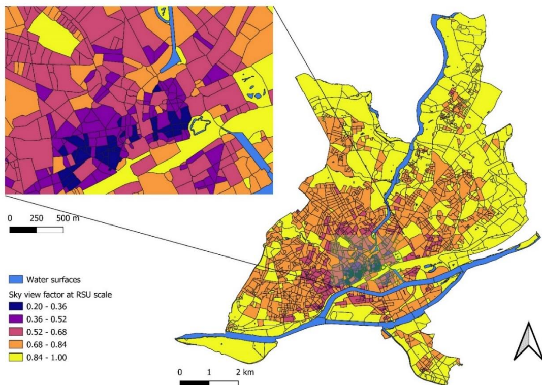
Figure 2-9 : Average sky view at RSU scale
