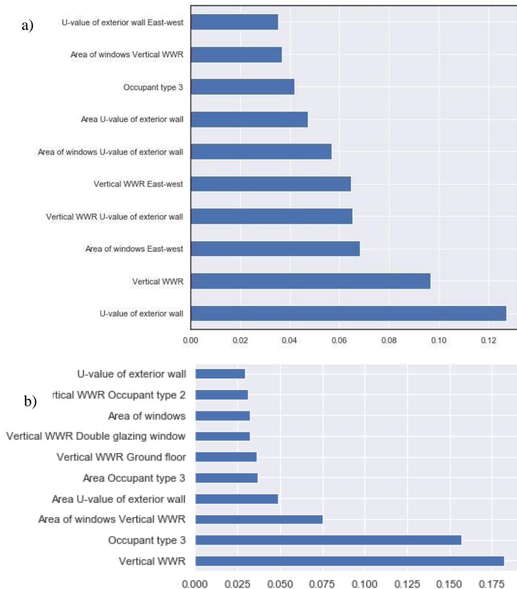
Figure 5-7 : Feature importance analysis results on combined input parameters for a): KM7_5 and b): KM7_6
