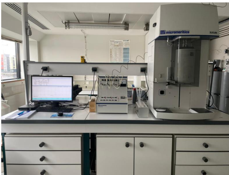
Fig. A.4 3-flex micromeritics apparatus for N 2 adsorption/desorption analysis
