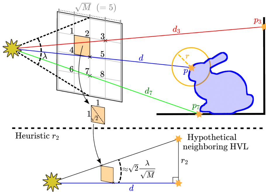
Figure 5.7: Diagram of the proposed heuristics to compute the radius of the HVL.
