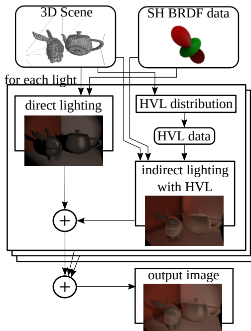
Figure 5.4: Overview of the HVLs rendering pipeline. The inputs are a 3D scene with dynamic objects and lights, along with precomputed BRDF spherical harmonics coefficients. For each primary light of the scene, direct lighting is computed using SH framework. Indirect lighting starts with the distribution of HVLs from primary lights, followed by the gathering of HVLs contributions at each pixel. This pipeline allows using parametric like measured BRDF at the same cost.
