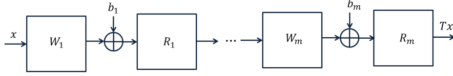
Figure 2.1: m -layered feed-forward neural network architecture. For the i^{th} -layer, W_i is the linear weight operator, b_i the bias vector, and R_i the activation operator.
