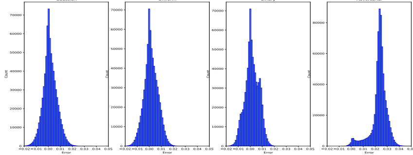
Figure 3.5: Error distribution of random attacks and proposed adversarial attack on industrial dataset for perturbation level of 2 \times 10^{-1} for \ell_2 attack.
