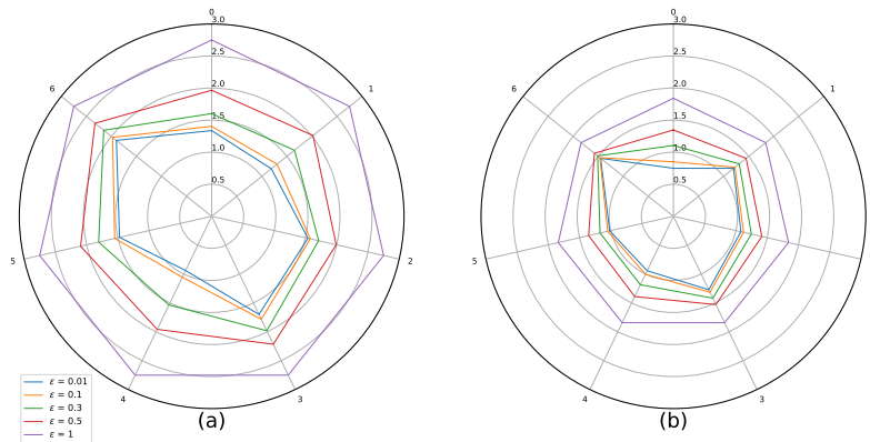
Figure 4.7: Sensitivity w.r.t. to each input on Auto MPG dataset. Effect of adversarial training. a) Standard training: Lipschitz constant = 2.75, MAE = 0.05, b) Adversarial training: Lipschitz constant = 1.84, MAE = 0.042.
