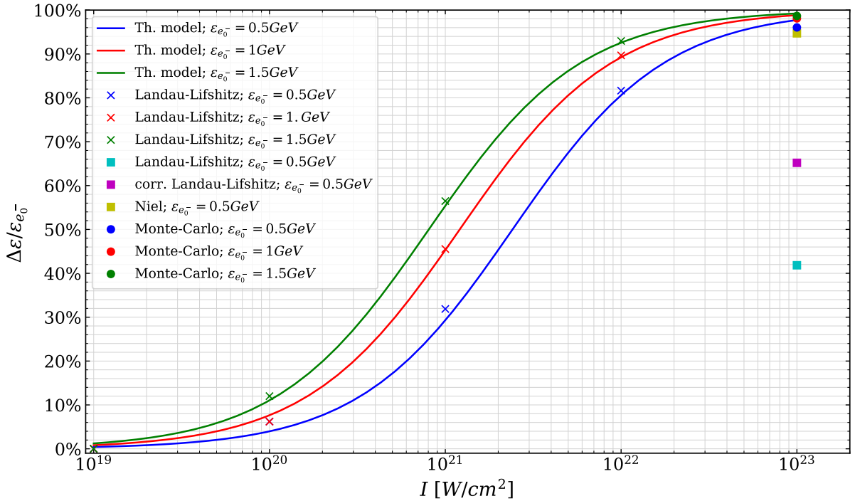
Figure 5.2: Electron energy loss vs laser intensity as obtained from 2D PIC simulations. The continuous lines (blue - \epsilon_e^- = 0.5 GeV, red - \epsilon_e^- = 1 GeV, green - \epsilon_e^- = 1.5 GeV) represent the theoretical scaling from Eq.(5.1). The simulation results are represented as follows: the continuous Landau-Lifshitz model - crosses (blue - \epsilon_e^- = 0.5 GeV, red - \epsilon_e^- = 1 GeV, green - \epsilon_e^- = 1.5 GeV); for I = 10^{23} W/cm 2 : continuous Landau-Lifshitz model - azure square, corrected Landau-Lifshitz model - magenta square, stochastic Niel model - yellow square and stochastic Monte Carlo model - circles (blue - \epsilon_e^- = 0.5 GeV, red - \epsilon_e^- = 1 GeV, green - \epsilon_e^- = 1.5 GeV).
