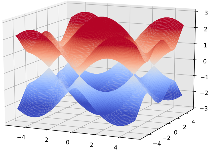
Figure 3.2 – The Wallace model. The dispersion relation is invariant with respect to the rotation by \pi/3 about the origin. We observe conical singularities, Dirac points, at the vertices of the Brillouin zone \Gamma^* .
