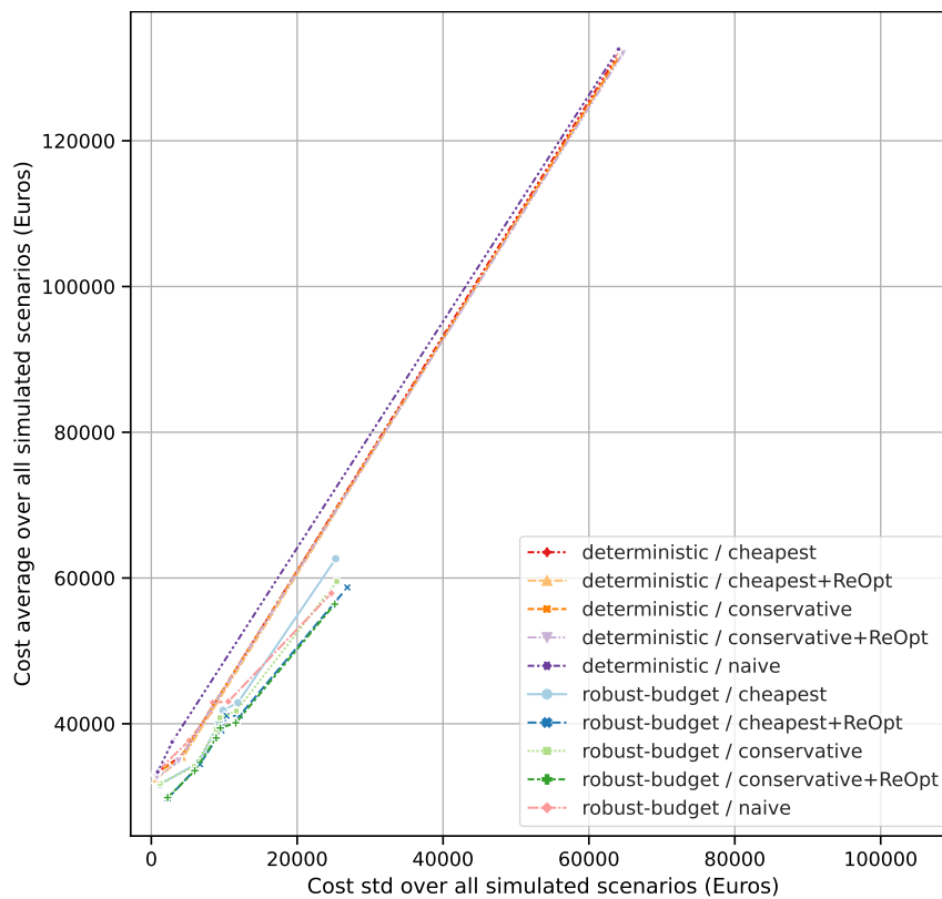
Figure 2.2 – Winter instance: daily cost std and cost average obtained with simulations of cheapest, cheapest+ReOpt, conservative, conservative+ReOpt and naive policies, based on either deterministic or robust budget models with \Phi = 0\%, 50\%, 100\% and \Gamma = 0\%, 20\%, 40\%, 60\%, 80\%, 100\% , respectively.
