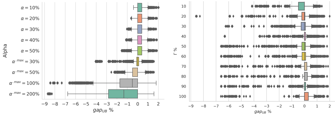
Figure 3.8 – Box plots of gap_{UB}\% values for instance group Taillard 20 \times 5 , grouped by instance alpha (left) and by \Gamma\% (right), based on all solution values obtained by GRASP and C&CG methods. Considers all C&CG solutions, optimal or not. All GRASP solution values were obtained from 50 independent executions of GRASP.
