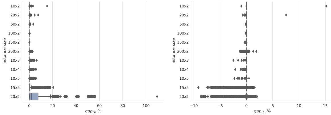
Figure 3.6 – Box plots of GRASP gap_{LB}\% (left plot) and gap_{UB}\% (right plot) values, grouped by instance size, compared to the lower and upper bounds obtained by the C&CG method, respectively. Considers all C&CG solutions, optimal or not.
