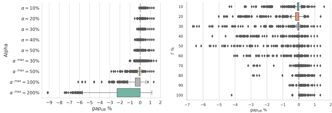
Figure 3.7 – Box plots of gap_{UB}\% values for instance group Ying 15 \times 5 , grouped by instance alpha (left) and by \Gamma\% (right), based on all solution values obtained by GRASP and C&CG methods. Considers all C&CG solutions, optimal or not. All GRASP solution values were obtained from 50 independent executions of GRASP.
