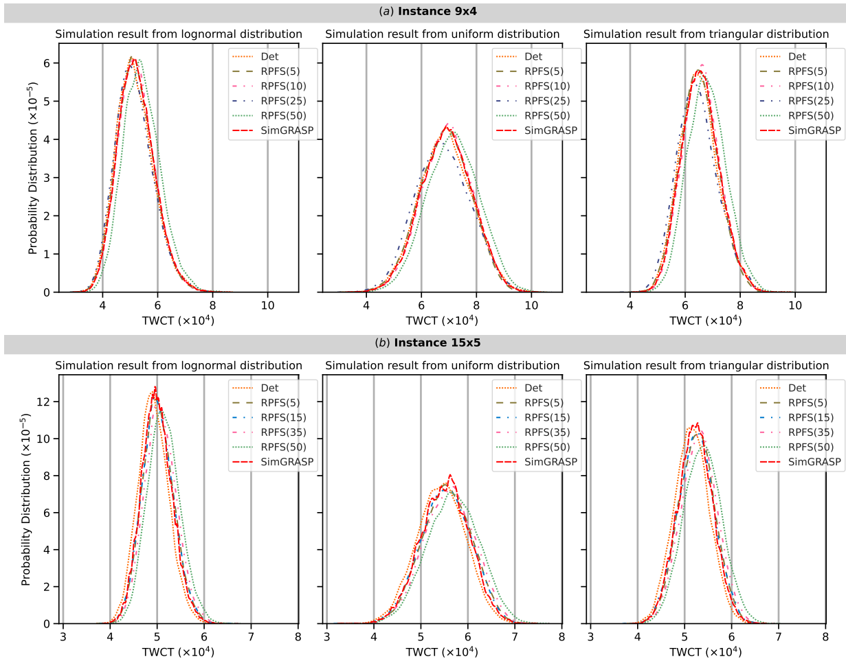
Figure 4.3 – Probability distributions of TWCT value for RPFSS( \Gamma ), Det and SimGRASP solutions, according to simulation results from lognormal, triangular, and uniform distributions for uncertain processing times.
