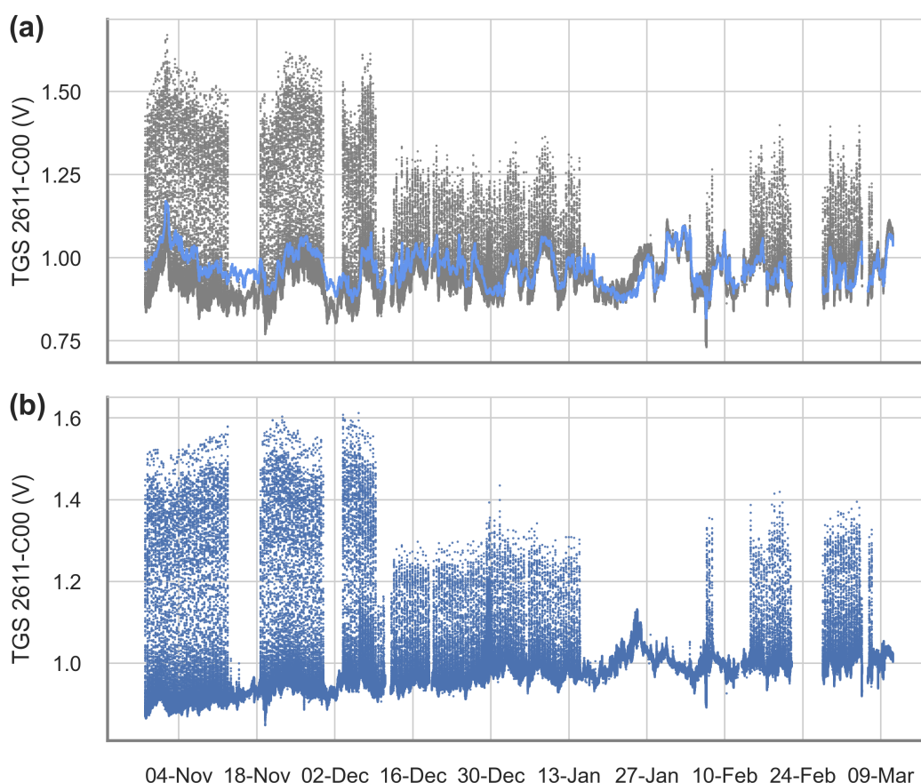
Figure B.2: Derived contribution and correction of water vapor for the Figaro TGS 2611-C00. (a) The raw voltage signal (gray) and the derived cross-sensitivities to H_2O (blue). (b) The cross-sensitivity corrected signal.
