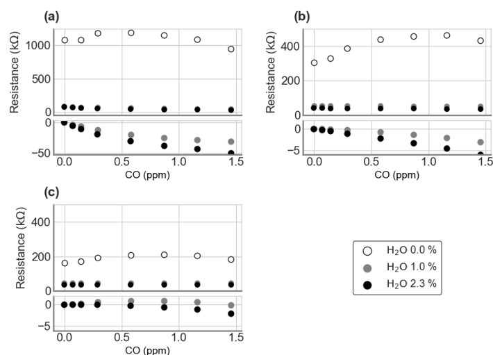
Figure 2.2: Measured sensitivity of Figaro ® sensors (a) TGS 2600, (b) TGS 2611-C00 and (c) TGS 2611-E00 to CO, at different humidity levels. Upper plots show the measured resistance, while lower plots show the contribution to the resistance due to CO.
