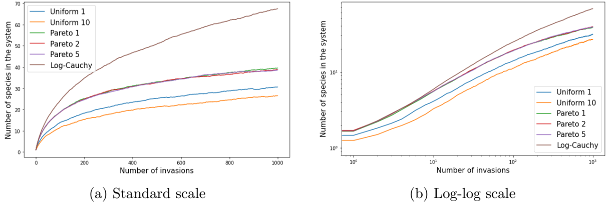
Figure 4.3.9: Representation of the species richness of the assembly as a function of the invasions for different distributions. The curve is derived using Monte Carlo simulations by computing P = 2000 times the algorithm 2 and averaging the number of persistent species. In panel (a) the plot corresponds to the standard case, whereas panel (b) is the same plot using log-log scale.
