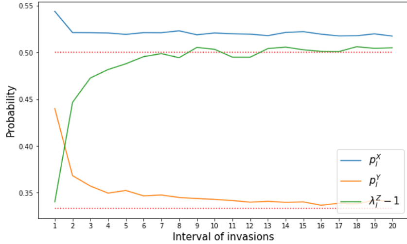
Figure 4.3.6: Representation of the parameters (p_l^X, p_l^Y, \lambda_l^Z - 1) as a function of interval of invasions. A interval of invasions i \in [1, 20] corresponds to [100(i-1), 100i] . In this example, the sequential invasion process count n = 2000 invasions in total and c_{new} is sampled from a uniform distribution \mathcal{U}([0, 1]) . Each interval l provides an estimator of the parameters. The red dotted horizontal lines are indicators plotted respectively at 1/3 and 1/2.
