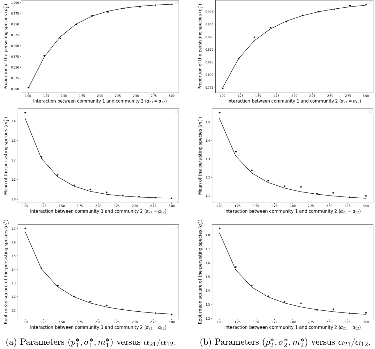
Figure 3.3.1: Comparison between the theoretical solutions (p_1^*, p_2^*, \sigma_1^*, \sigma_2^*, m_1^*, m_2^*) of (3.20)-(3.25) and their empirical Monte Carlo counterpart (the star marker) as functions of the off-diagonal block interaction strength \alpha_{12}/\alpha_{21} . The left column is associated to the properties of Community 1. The right column is associated to the properties of Community 2. Matrix B has size n = 100 and the number of Monte Carlo experiments is 500. The parameters are \boldsymbol{\mu} = \begin{pmatrix} 0 & 0 \\ 0 & 0 \end{pmatrix} , \boldsymbol{\alpha} = \begin{pmatrix} 3 & \alpha_{12} \\ \alpha_{21} & \sqrt{2} \end{pmatrix} , \boldsymbol{\beta} = (\frac{1}{2}, \frac{1}{2}) . When off-diagonal block interaction \alpha_{12}^{-1}, \alpha_{21}^{-1} increases, the number of persisting species p^* decrease but their variance \sigma^* and mean m^* increase.
