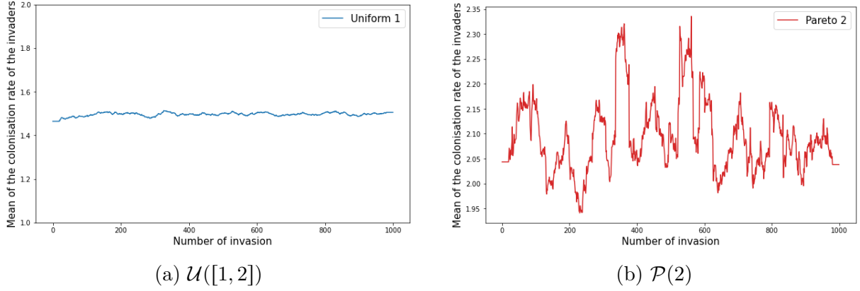
Figure 4.D.2: Representation of a moving average on the colonization rates of the invaders for a sequential invasion process of size n = 1000 . A Monte Carlo experiment is realized P = 100 times by getting times series of the moving average curve on the colonization values and average the time series of P sequential invasion process. In Fig. (a), the plot corresponds to the uniform distribution \mathcal{U}([1, 2]) . In Fig. (b), the plot corresponds to the Pareto distribution with parameter a = 2 .
