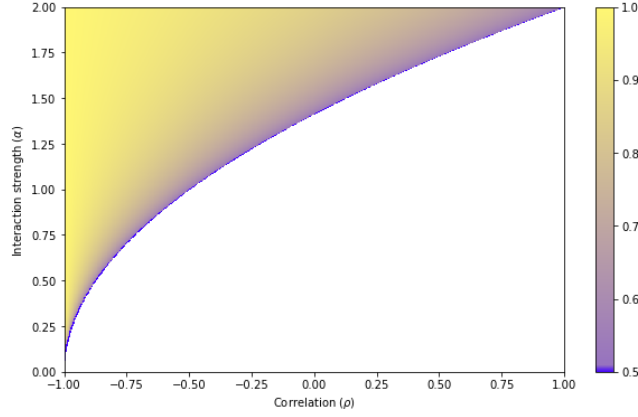
Figure 2.2.2: Representation of the set of admissible parameters \mathcal{A} by a heat map. The set \mathcal{A} given by (2.7) yields the existence of a unique (random) globally stable equilibrium \mathbf{x}^* . The x -axis corresponds to \rho , the y -axis to \alpha and the intensity of the color \mu .
