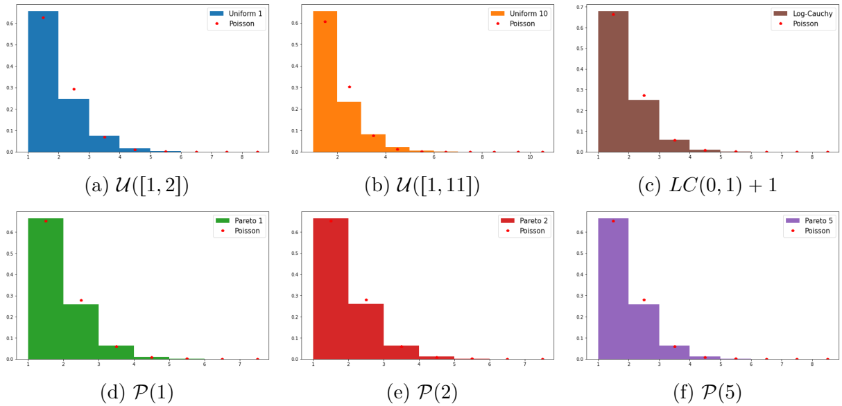
Figure 4.3.13: Histogram of the number of extinctions for a fixed number of invasion trials n = 1000 computed for a large number of sequential invasion process P = 500 . The red point corresponds to the Poisson distribution with a estimated mean.
