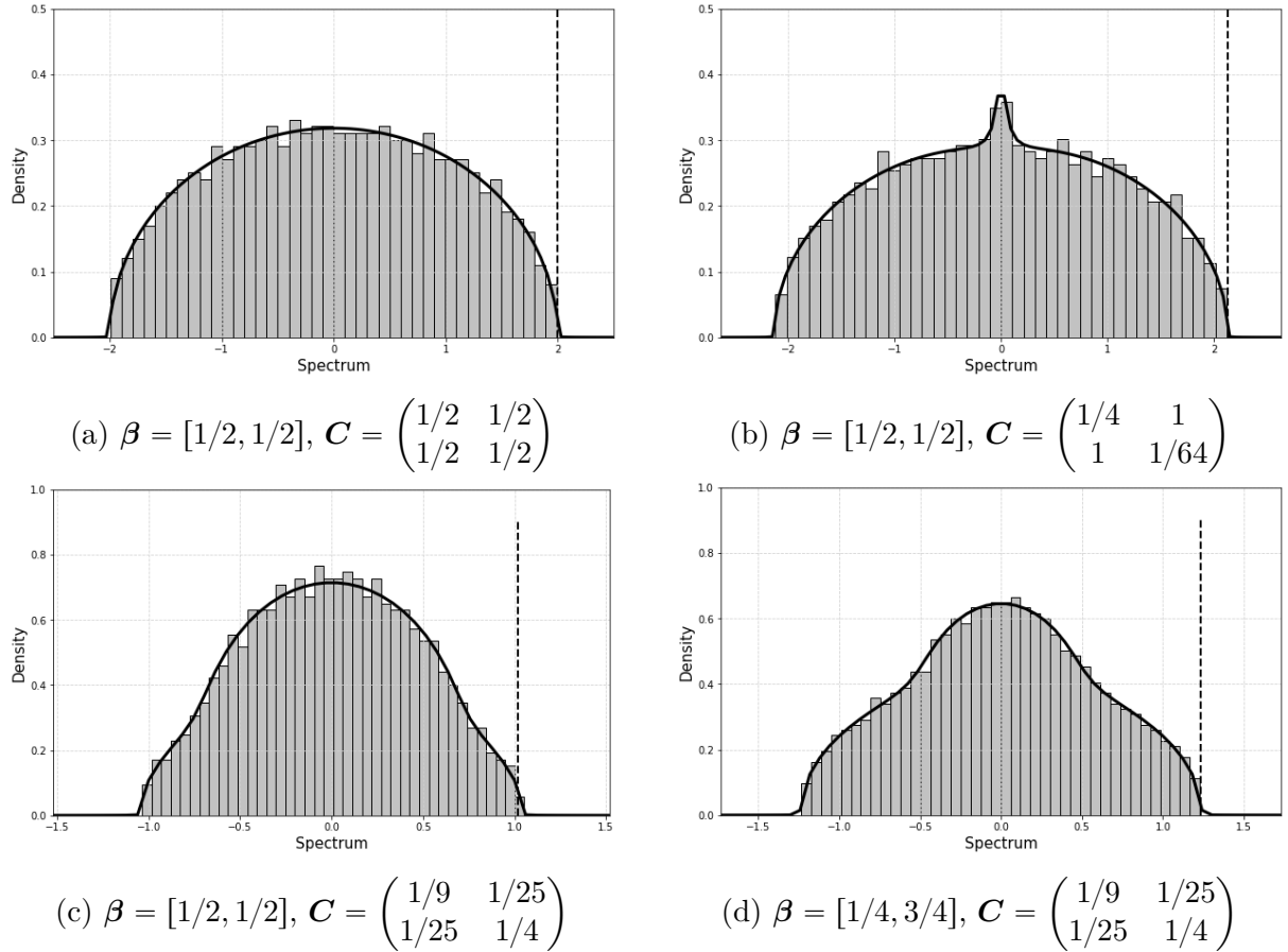
Figure 3.4.4: Spectrum (histogram) of the Hermitian random matrix B^S + (B^S)^\top ( n = 1000 ), condition on (\beta, \mathbf{C}) are given in each sub-figures. The solid line represents the distribution of the spectrum computed by the numerical approach. The dashed vertical line indicates the upper bound of the largest eigenvalue of B + B^\top given by 2\|S\|_2^{1/2} .
