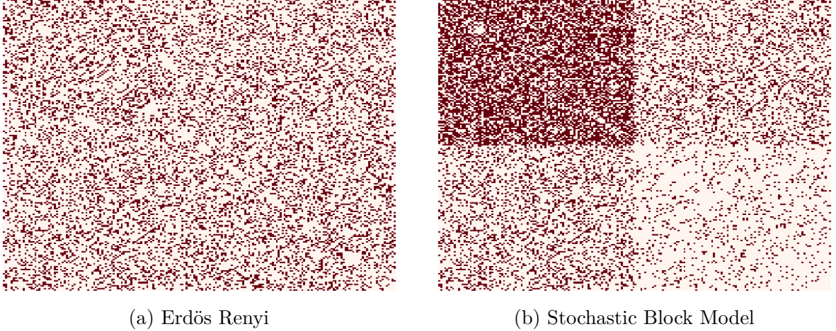
Figure 3.4.1: Representation of an adjacency matrix of the interactions of an ecosystem of size n = 200 . In Fig (a), an Erdős Renyi graph of parameter \mathcal{G}(200, 0.25) is illustrated. In Fig (b) a graph of a symmetric Stochastic Block model of parameter P = \begin{pmatrix} 0.6 & 0.25 \\ 0.25 & 0.1 \end{pmatrix} . A red colored cell indicates S_{k\ell} = 1 , on the contrary, a white colored cell indicates that there is no interaction S_{k\ell} = 0 .
