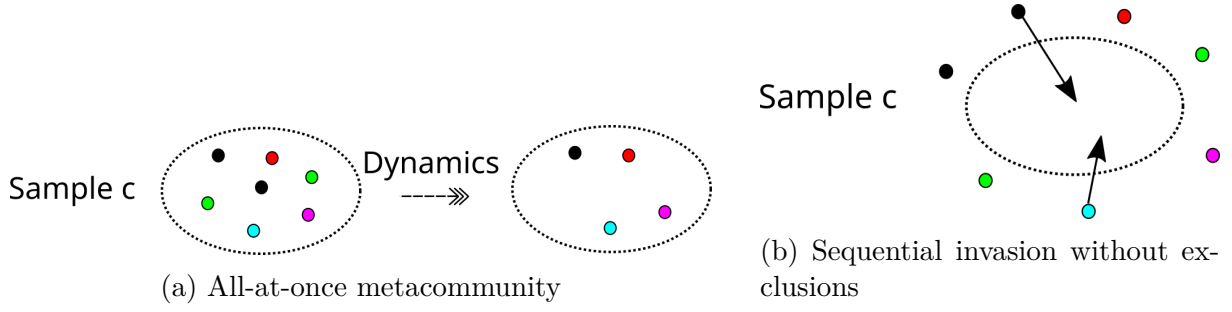
Figure 4.1.3: Diagrams of the two types of construction of the model (4.2) dynamics are represented for a ecosystem. The ellipse corresponds to the habitat and the points corresponds to the species. In Fig. (a), standard dynamics is shown. In Fig. (b), the assembly dynamics is represented with an invasion of each species.
