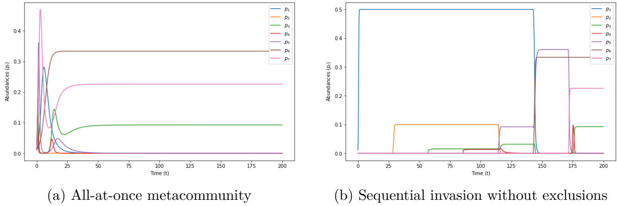
Figure 4.1.4: The two types of construction of the model (4.2) dynamics are represented for a ecosystem of 7 species ( n = 7 ). In Fig. (a), all-at-once metacommunity is shown with a starting pool of 7 species with random initial conditions. The abundance or habitat proportion of each species as a function of time is displayed. In Fig. (b), the sequential invasion without exclusions is represented with an invasion of each species at a regular time interval.
