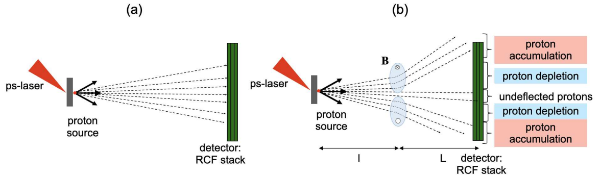
Figure 2.7: Principle of the proton radiography. (a) Protons are created via TNSA thanks to a ps- high-intensity laser. They have straight trajectories in absence of external electromagnetic fields (and if the beam density is not too high). (b) When protons encounter a region with an electromagnetic field (in this example, a magnetic torus), they are deflected. With respect to the unperturbed case, on the detector there will be zones with higher proton concentration and zones with lower.
