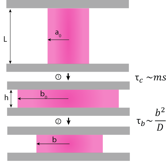
Figure 3.4: Schematic of the different stages of deformation of a cylindrical gel upon fast compression as depicted by Eq.3.47. Two stages and their associated timescales are depicted. (1) Compression of the gel at constant volume. (2) Shrinking of the gel.
