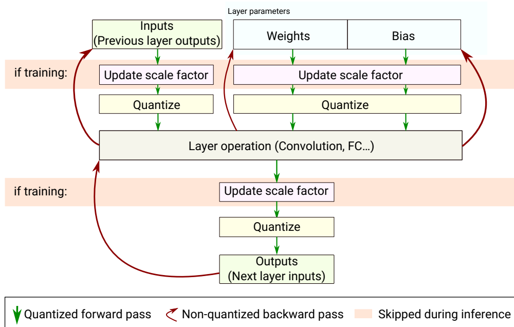
Figure 3.2: Quantization-aware training.
