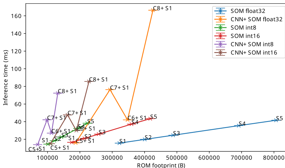
Figure 6.7: Inference time for quantized and non-quantized SOM and CNN+SOM models for UCI-HAR running on the SparkFun Edge board.
