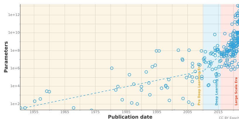
Figure 2.2: Parameter trend in machine learning [18].
