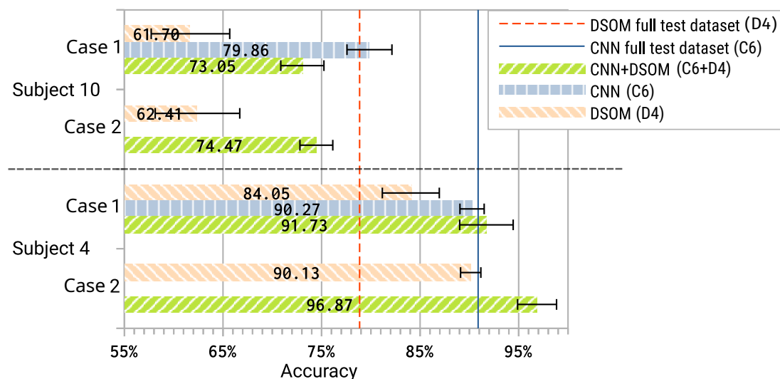
Figure 5.8: Accuracy of test subjects n°4 and n°10 of UCI-HAR with unsupervised fine-tuning.
