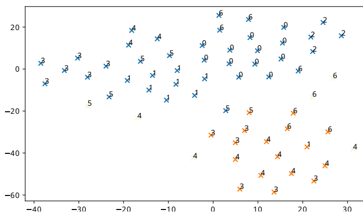
Figure 5.14: t-SNE visualization of the 8 \times 8 DSOM neurons prototype vector on UCA-EHAR with labels after step n^{\circ}2 .
