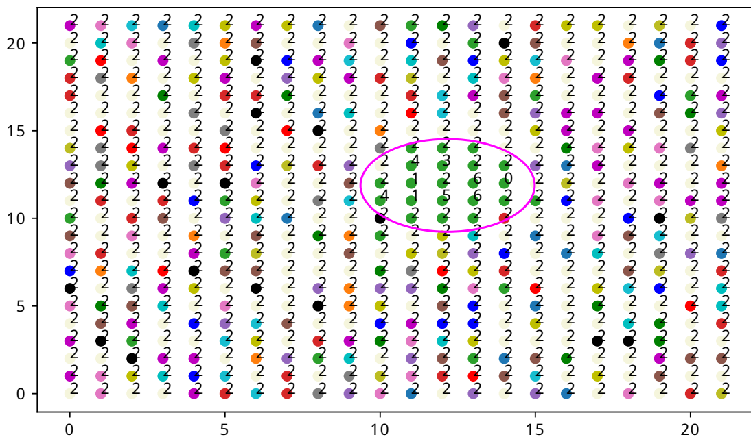
Figure 5.12: Labelled 22 \times 22 DSOM 2-dimensional neurons grid on UCA-EHAR after step n^2 .
