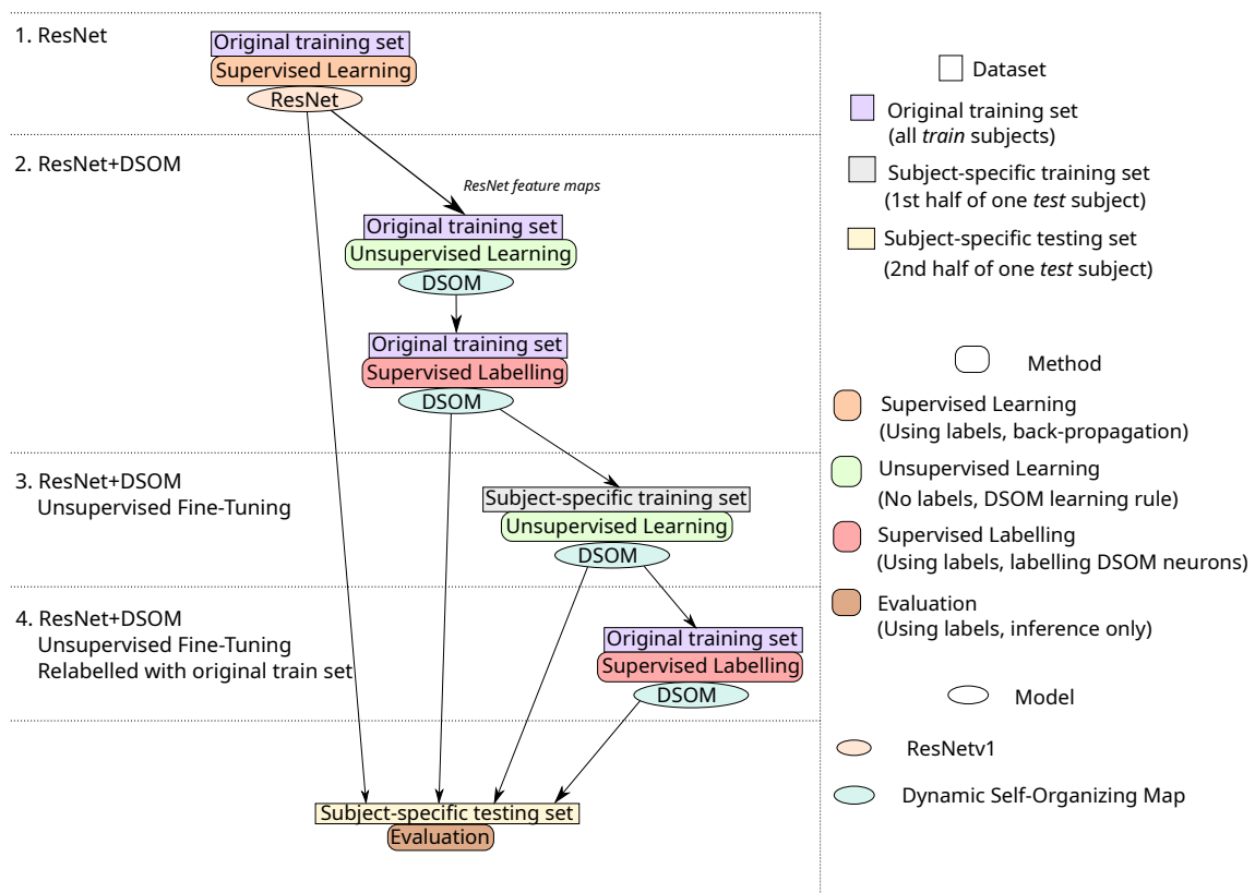
Figure 5.9: Method for unsupervised fine-tuning on UCA-EHAR.
