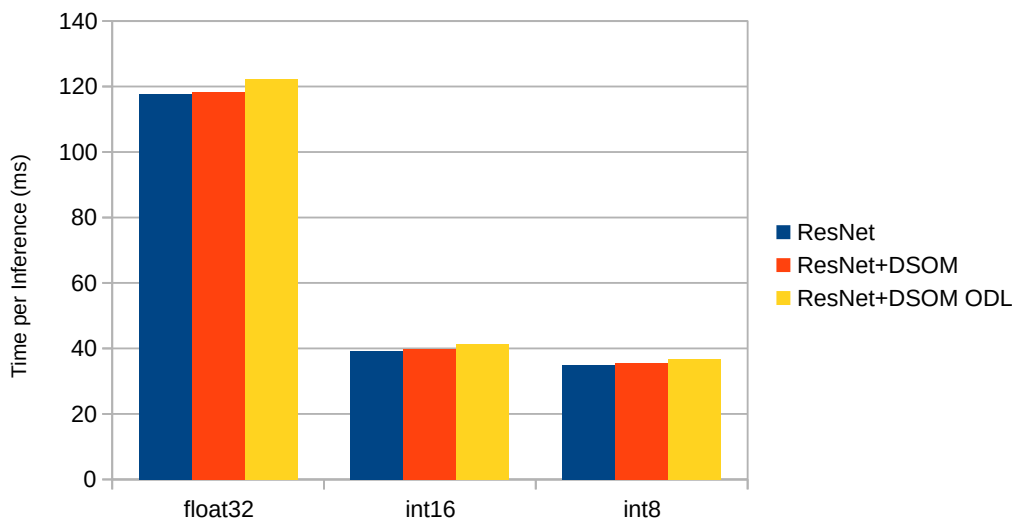
Figure 6.10: Inference time for a ResNet and ResNet+DSOM (with and without on-device learning) models for UCA-EHAR deployed on the SparkFun Edge board with and without quantization.
