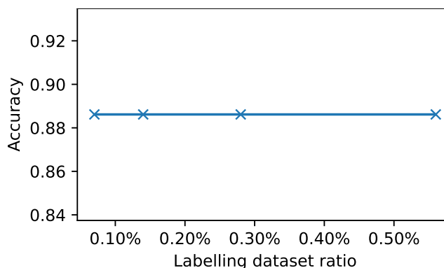
Figure 5.13: Accuracy vs. percentage of the training set used for labelling of the 4 \times 4 DSOM trained from ResNet feature maps after step n^{\circ}2 .
