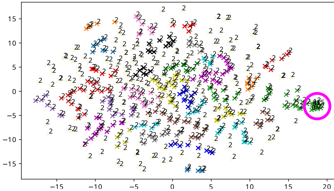
Figure 5.11: t-SNE visualization of the 22 \times 22 DSOM neurons prototype vector on UCA-EHAR with labels after step n^2 .
