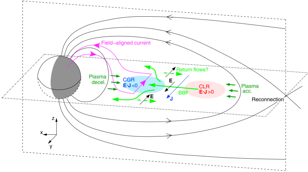
FIGURE 2.4 – Schematic image representing the association between Energy Conversion Regions (ECRs) and BBFs in the equatorial plane (adapted from Hamrin et al. (2011)).
