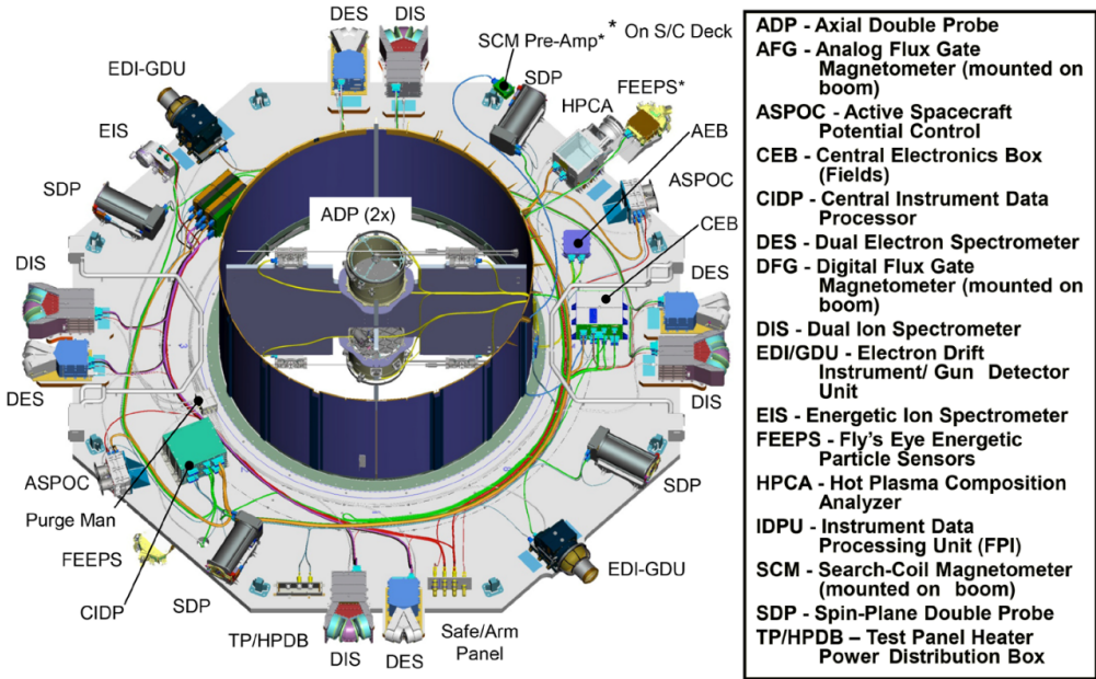
FIGURE 3.3 – FIELDs sensors on the MMS spacecraft. Adapted from Burch et al. (2015)
