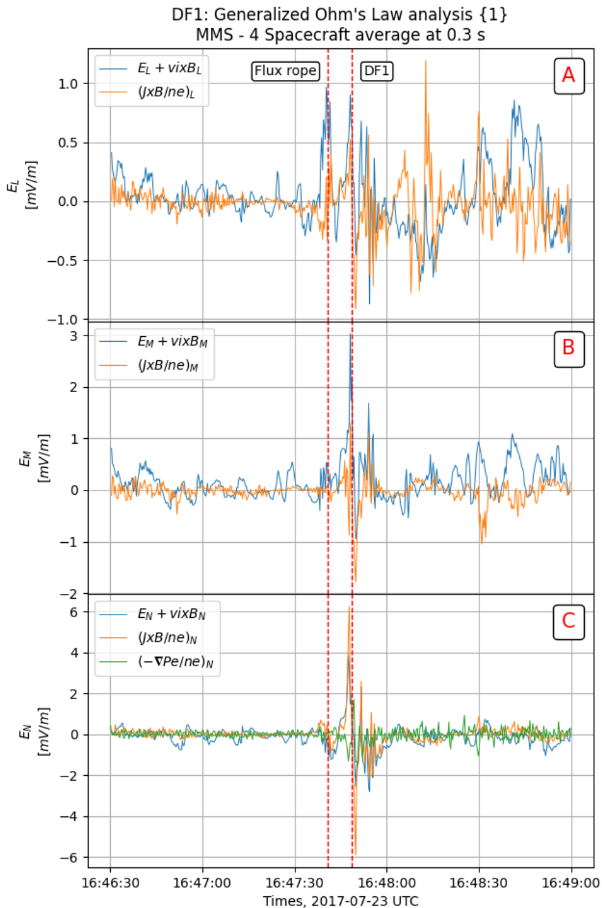
FIGURE 4.3 – Panels A, B, and C show L, M, N components of Ion Ohm's Law terms respectively : \mathbf{E} + \mathbf{v}_i \times \mathbf{B} (blue line), (\mathbf{J}_{part} \times \mathbf{B}) / (ne) (orange line). Panel C also includes electron pressure gradient term along N (green line).
