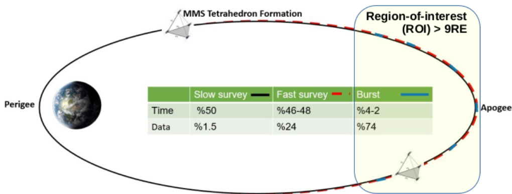
FIGURE 3.2 – A day in the life of MMS orbit indicates the region of interest in light yellow (ROI).
