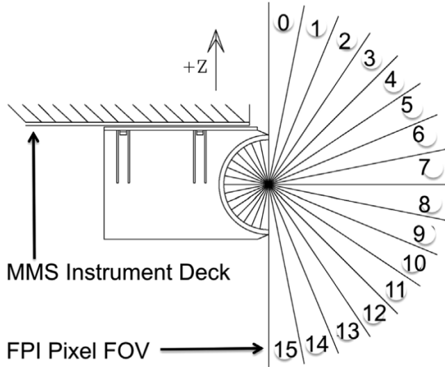
FIGURE 3.5 – Each FPI 180^\circ polar angle top hat is mounted so that the 180^\circ fan spans from the spacecraft spin axis to the anti-spin axis. Each sensor is oriented so that the 16 pixels (each nominally 11.25^\circ wide) of its 180^\circ Field Of View (FOV) are viewing radially in velocity space, spanning the 180^\circ pole-to-pole range in the spinning spacecraft reference frame, Adapted from Pollock et al. (2016).
