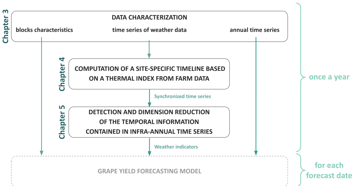
Figure 3.3 – Positioning of the two research axes aiming at valuing the time series of meteorological data in the framework of yield the forecasting method. The yield model, in light grey, constitutes a a further work perspective to achieve the yield forecasting method.
