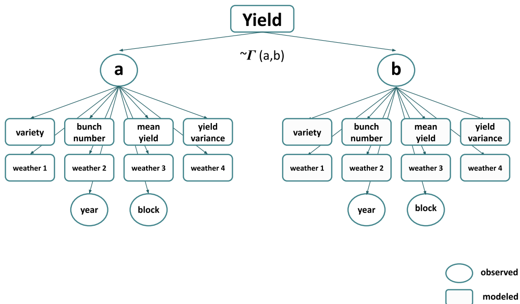
Figure 6.3 – Preliminary representation of a hierarchical Bayesian model for grape yield forecasting. Yield is considered to follow a Gamma law of parameter a and b. These a and b parameters are modelled according to covariates referring to the variety, the mean number of bunches per vine, the mean and variance of previous yield performances for the considered block, weather indicators and two random effects (year and block effects).
