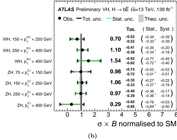
Figure 5.25: Expected (lines) versus observed (markers) VH ( V \rightarrow \text{lepton} ) cross-sections times the H \rightarrow b\bar{b} branching fraction in the reduced 1.2 STXS scheme (a) for the combination (green) compared to the resolved only [65] (blue) and boosted only [275] (orange) analyses results. The horizontal dashed lines indicate the expected values in the p_T^{V,t} > 250 GeV category since the published resolved analysis did not include a split at a p_T^{V,t} of 400 GeV. (b) Signal strength measurement for the 7 STXS bins. The grey shaded area shows the theoretical uncertainty on the SM prediction (taken from Ref. [5]).
