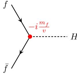
Figure 1.6: Leading order fermion couplings to the Higgs and interaction vertex factor as predicted by the Yukawa theory.
