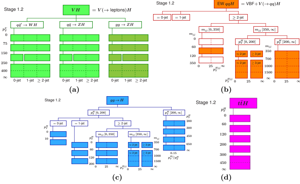
Figure 1.9: STXS stage 1.2 bin definitions for (a) VH, V(\rightarrow \text{leptons})H , (b) vector boson fusion (VBF) and VH, V(\rightarrow qq) , (c) gg \rightarrow H and (d) t\bar{t}H processes (taken from Ref. [56]).
