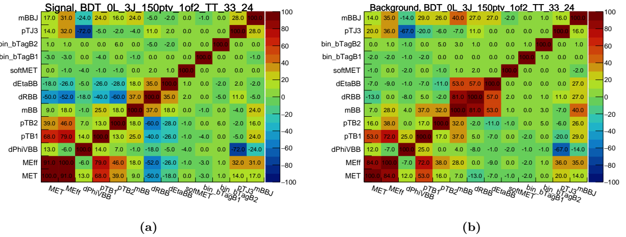
Figure 6.5: BDT input variables correlation matrices for the (a) signal and (b) background events in the 2 b -tagged 3-jets region as predicted by the nominal simulation using truth tagging.
