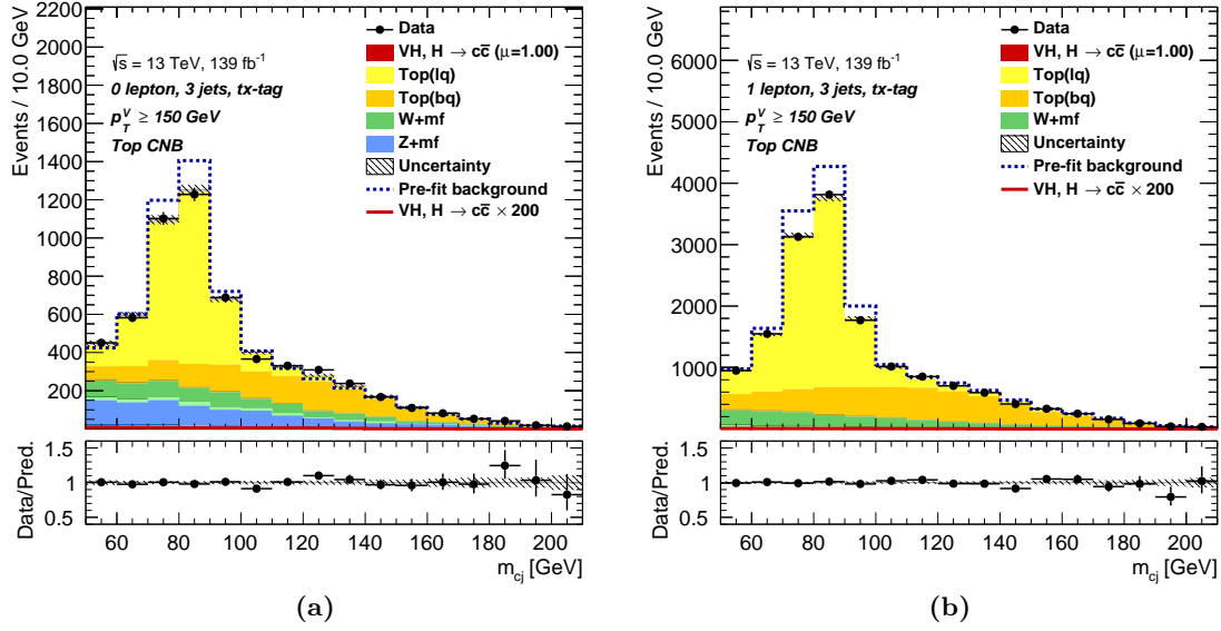
Figure 5.13: Top TNB control region (abusively called CNB CR) in the (a) 0- and (b) 1-lepton channels for p_T^V > 150 GeV. The mixed flavour (mf) components refer to bc , bl and cl true flavour of the two jets constituting the Higgs candidate system. The ratios of the data to the sum of the fitted signal and background are shown in the lower panels.
