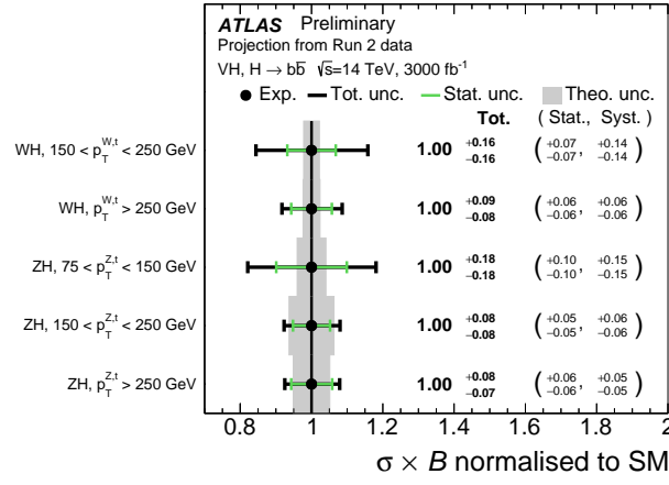
Figure 5.56: Signal strength for the resolved VH, H \rightarrow b\bar{b} signal in the reduced 1.2 STXS scheme as extrapolated to the HL-LHC conditions. The theory uncertainties are shown as a grey band and reduced by a factor 1/2 with respect to the Run 2 analysis (taken from Ref. [339]).
