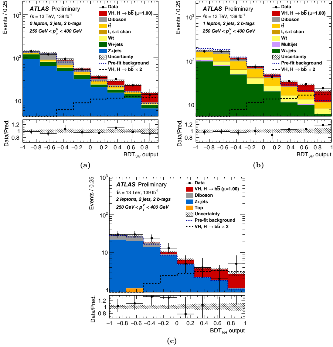
Figure 5.27: (a) 0-lepton, (b) 1-lepton and (c) 2-lepton post-fit distributions of the BDT discriminant in the resolved regime 2 b -tagged 2-jets signal region for 250 < p_T^V < 400 \text{ GeV} . The background processes are normalized thanks to the global likelihood fit, the total pre-fit background distribution is shown as a dashed blue line. The Higgs boson signal is shown as a filled histogram on top of the fitted backgrounds normalized to the signal yield extracted from data ( \mu = 1.00 ), and unstaked as an unfilled histogram (dashed black line), scaled by the multiplicative factor indicated in the legend. The size of the combined statistical and systematic uncertainties for the sum of the fitted signal and background are indicated by the hatched band. The ratios of the data to the sum of the fitted signal and background are shown in the lower panels (taken from Ref. [5]).
