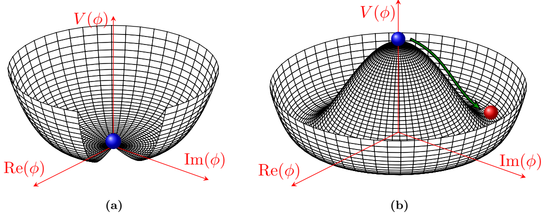
Figure 1.4: Higgs potential V(\phi) = \mu^2 |\phi|^2 + \lambda |\phi|^4 with \lambda > 0 and either (a) \mu^2 \geq 0 or (b) \mu^2 < 0 (schemes highly inspired by Refs. [45, 46]).
