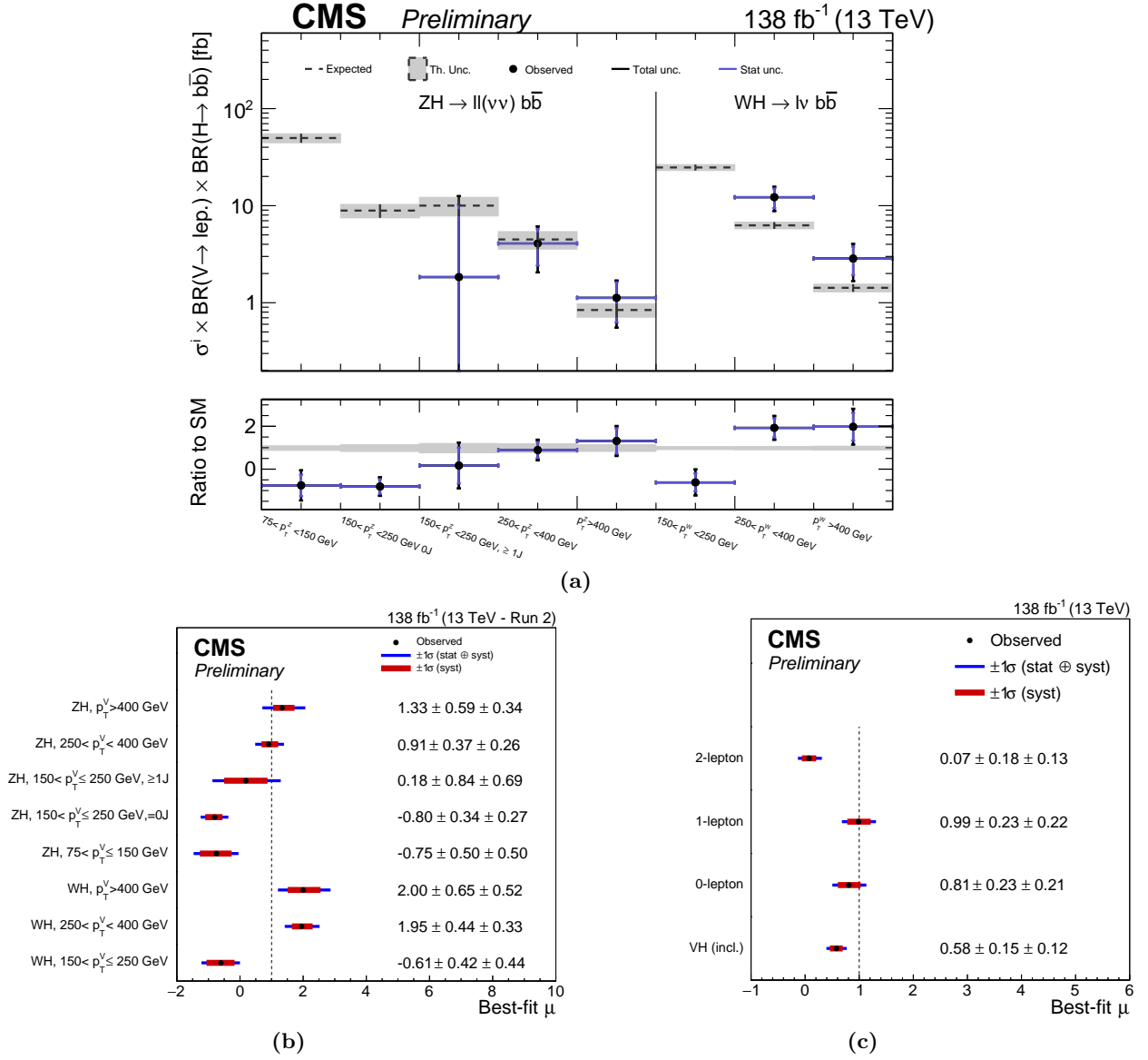
Figure 5.33: CMS full Run 2 (a) best-fit values and uncertainties for the VH ( V \rightarrow \text{leptons} ) cross-section times the H \rightarrow b\bar{b} branching fraction, in the reduced 1.2 STXS scheme. In the bottom panel, the ratio of the observed results with associated uncertainties to the SM expectations is shown. If the observed signal strength for a given STXS bin is negative, no value is quoted for \sigma\mathcal{B} . STXS signal strengths for (b) the 8 STXS bins of the analysis and (c) for the 0-, 1- and 2-lepton channels, as well as the combined signal strength (taken from Ref. [329]).
