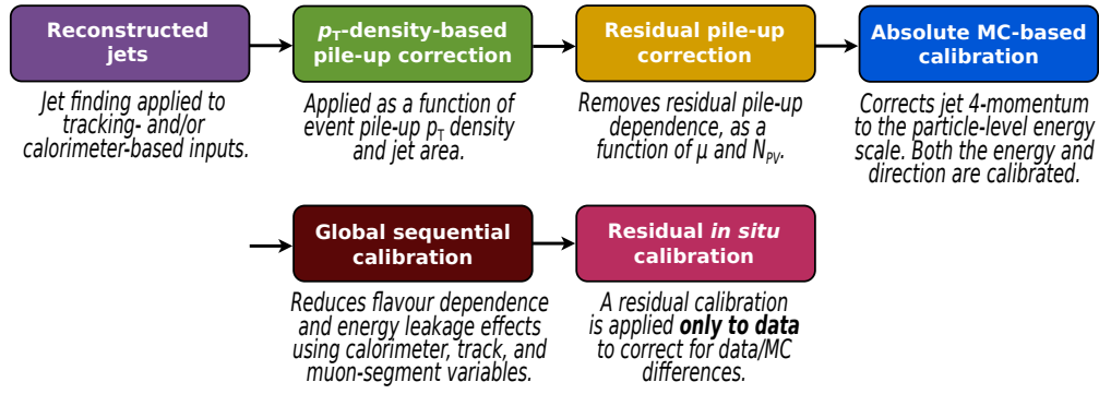
Figure 3.14: Different steps of jet calibration (taken from Ref. [193]).
