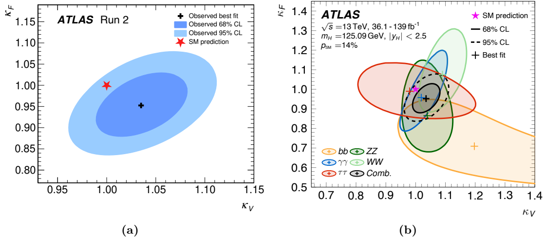
Figure 1.17: (a) Negative log-likelihood contours corresponding to the 68% and 95% confidence level in the (\kappa_V, \kappa_F) plane. They are obtained from a combined fit assuming no contributions from invisible or undetected non-SM Higgs boson decays. A p -value of 14% is found for the compatibility of the combined measurement and the SM prediction. (b) Same figure showing the individual decay modes (colour) 68% confidence level contour in the (\kappa_V^k, \kappa_F^k) plane and their combination (black). The 95% CL contour of the combined measurement is also shown (black dashes) (taken from Ref. [58]).
