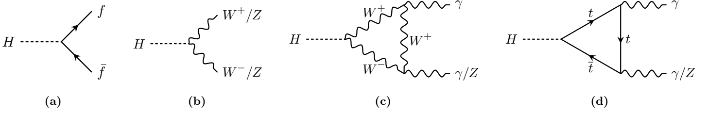
Figure 1.14: Feynman diagrams of some Higgs decay channels: Higgs decays to (a) fermions, (b) vector bosons ( V = W, Z ), and (c) and (d) two photons ( \gamma\gamma ) or a Z boson and a photon ( Z\gamma ).
