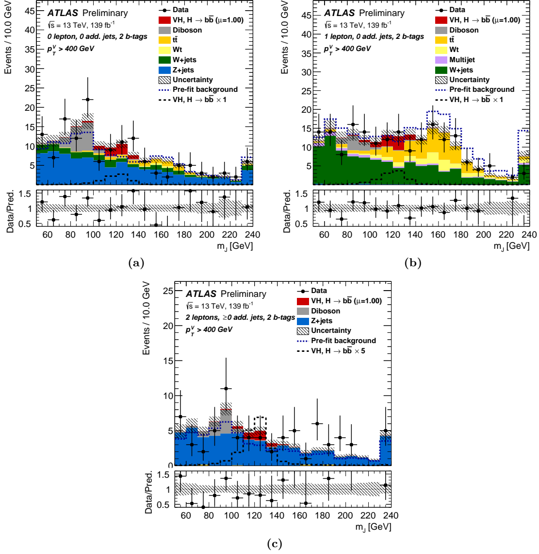
Figure 5.28: (a) 0-lepton, (b) 1-lepton and (c) 2-lepton post-fit distributions of the invariant mass of the leading large- R jet in the boosted regime high for p_T^V > 400 GeV in the (a) and (b) high purity signal regions, and (c) in the signal region as there is indeed no HP SR, LP SR and CR in the 2-lepton channel: all regions are merged together to circumvent the low statistic available. The contributions of each process are plotted after the global likelihood fit. The Higgs boson signal is shown as a filled histogram on top of the fitted backgrounds normalized to the signal yield extracted from data ( \mu = 1.00 ), and unstaked as an unfilled histogram (dashed black line), scaled by the multiplicative factor indicated in the legend. The dashed histograms show the total pre-fit background. The size of the combined statistical and systematic uncertainties for the sum of the fitted signal and background are indicated by the hatched band. The ratios of the data to the sum of the fitted signal and background are shown in the lower panels (taken from Ref. [5]).
